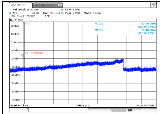
WCDMA V RMC Low channel
