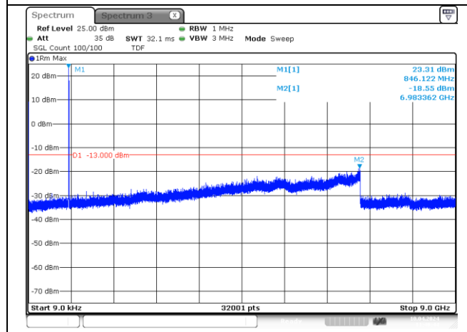
WCDMA V RMC High channel
