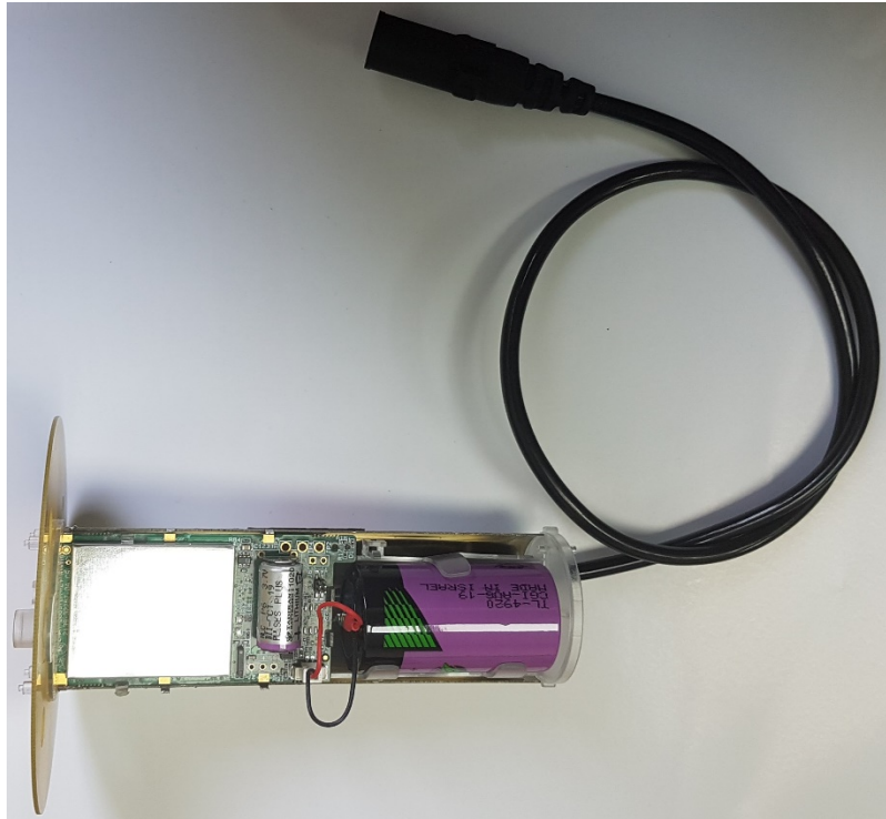
Assembly without plastic cover
