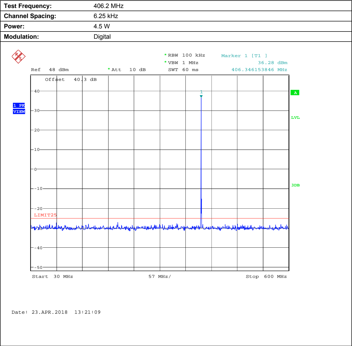
Plot 5.9.4.1.3. Conducted Transmitter Spurious Emissions for 406.2 MHz, Low Power, 30 - 600 MHz
