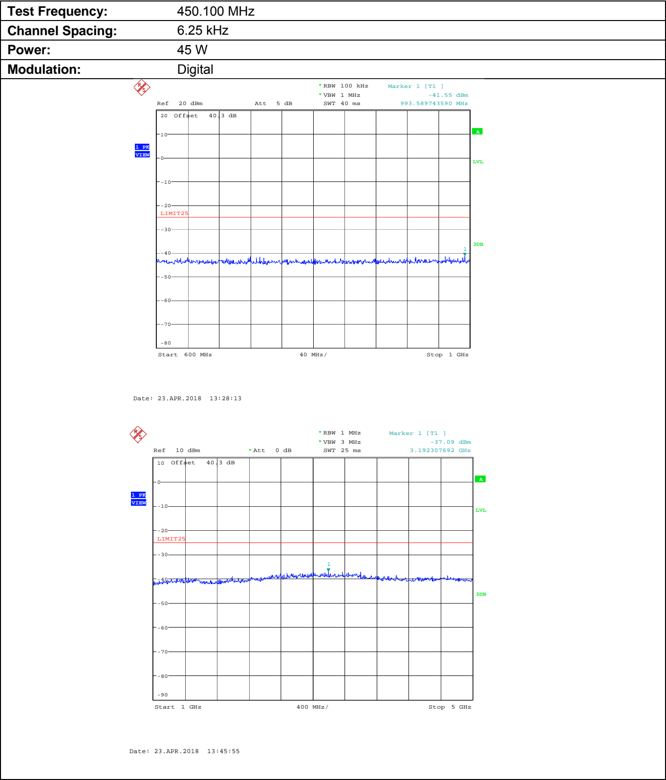
Plot 5.9.4.2.2. Conducted Transmitter Spurious Emissions for 450.100 MHz, High Power, 0.6 - 5 GHz
