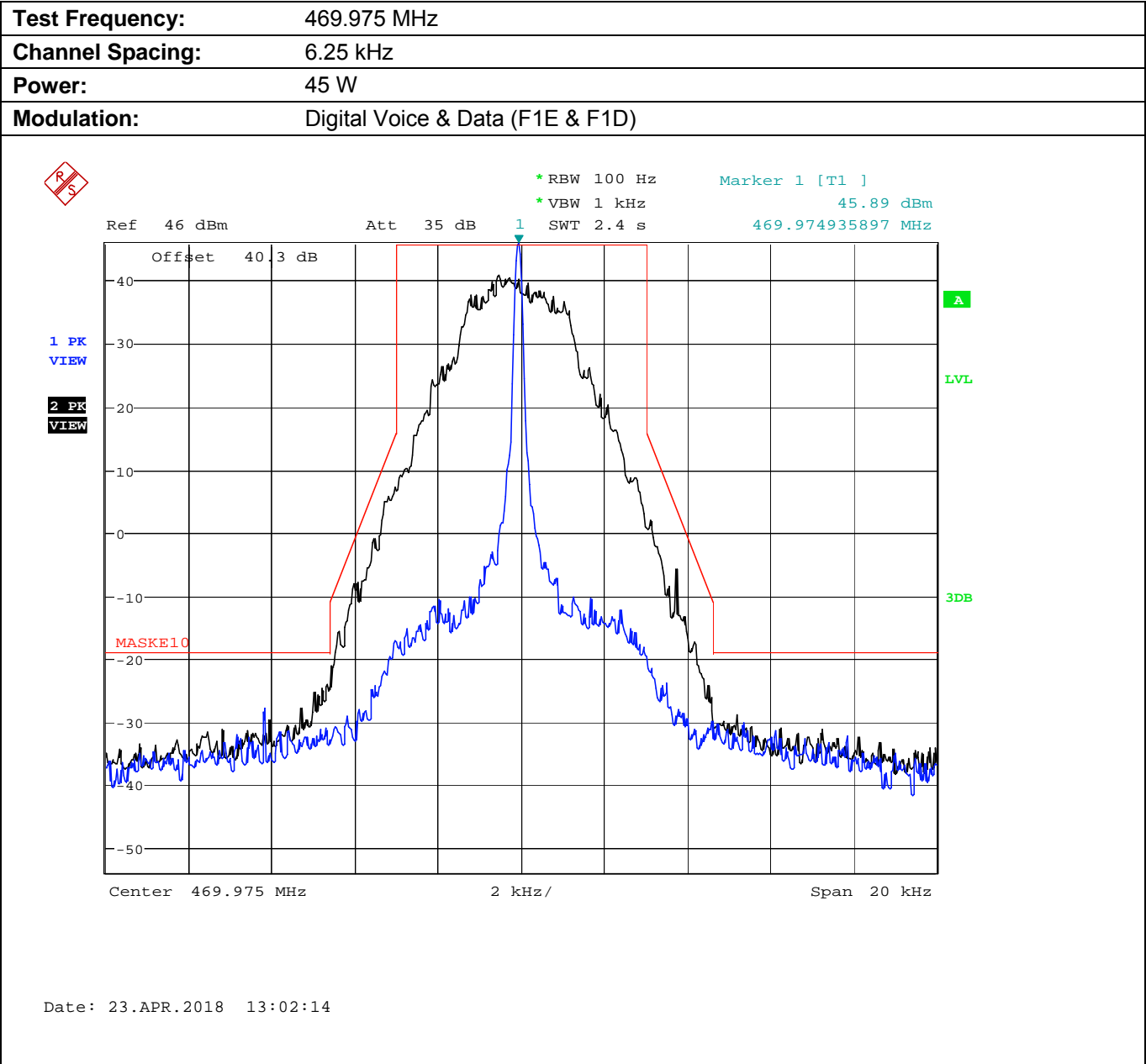
Plot 5.8.4.4.5. Emission Mask E, High Power
