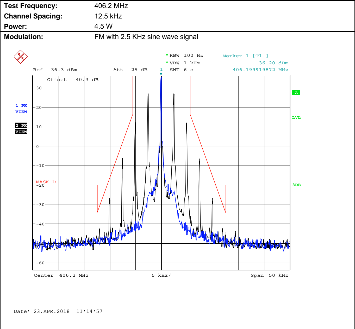
Plot 5.8.4.2.2. Emission Mask D, Low Power
