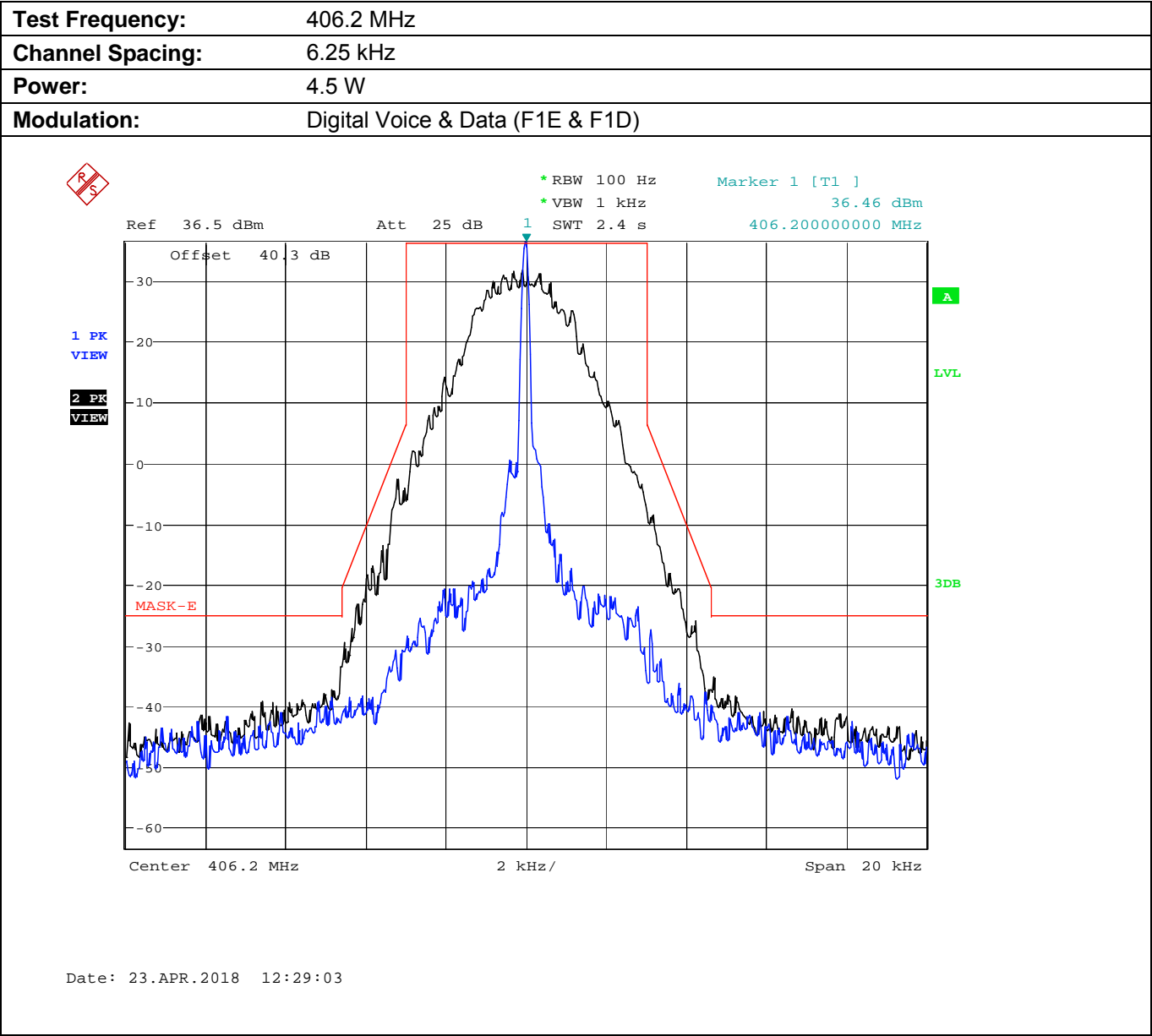
Plot 5.8.4.4.2. Emission Mask E, Low Power
