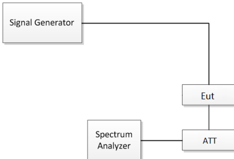
Fig.8. Noise/emission at Antenna Terminal
