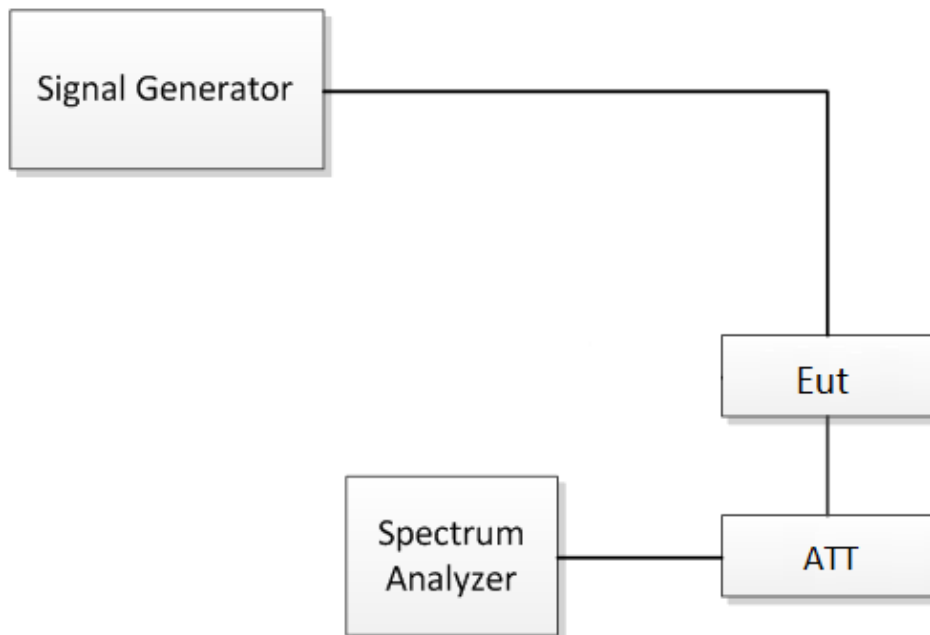
Fig.4. Emission mask test configuration
