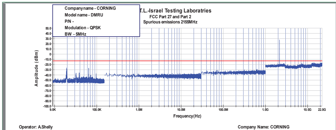
Figure 472: Spurious Emissions at Antenna Terminal QPSK, 2155MHz, B.W. 5MHz
