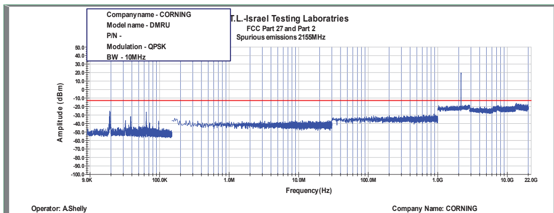
Figure 475: Spurious Emissions at Antenna Terminal QPSK, 2155MHz, B.W. 10MHz
