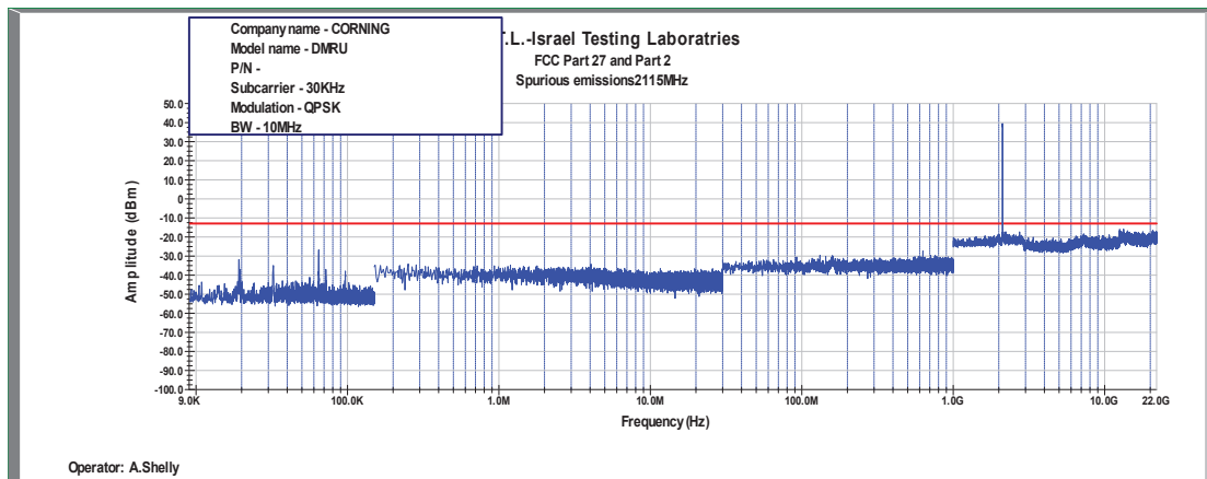
Figure 444: Spurious Emissions at Antenna Terminal QPSK, 2115MHz, B.W. 10MHz, Sub Carrier 30kHz
