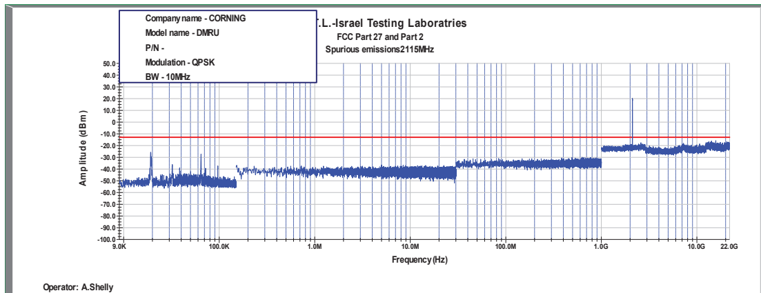
Figure 474: Spurious Emissions at Antenna Terminal QPSK, 2115MHz, B.W. 10MHz
