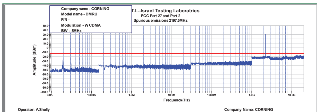
Figure 482: Spurious Emissions at Antenna Terminal WCDMA, 2197.5MHz, B.W. 5MHz
