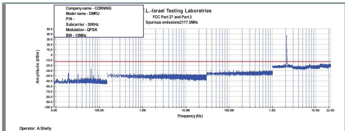
Figure 450: Spurious Emissions at Antenna Terminal QPSK, 2117.5MHz, B.W. 15MHz, Sub Carrier 30kHz
