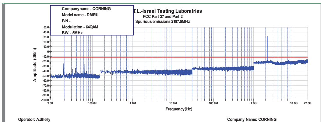
Figure 464: Spurious Emissions at Antenna Terminal 64QAM, 2197.5MHz, B.W. 5MHz
