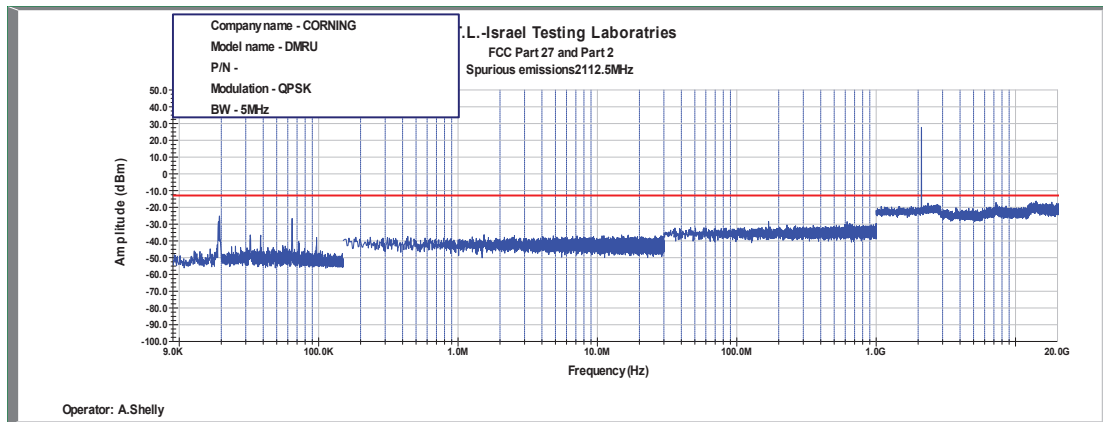
Figure 471: Spurious Emissions at Antenna Terminal QPSK, 2112.5MHz, B.W. 5MHz
