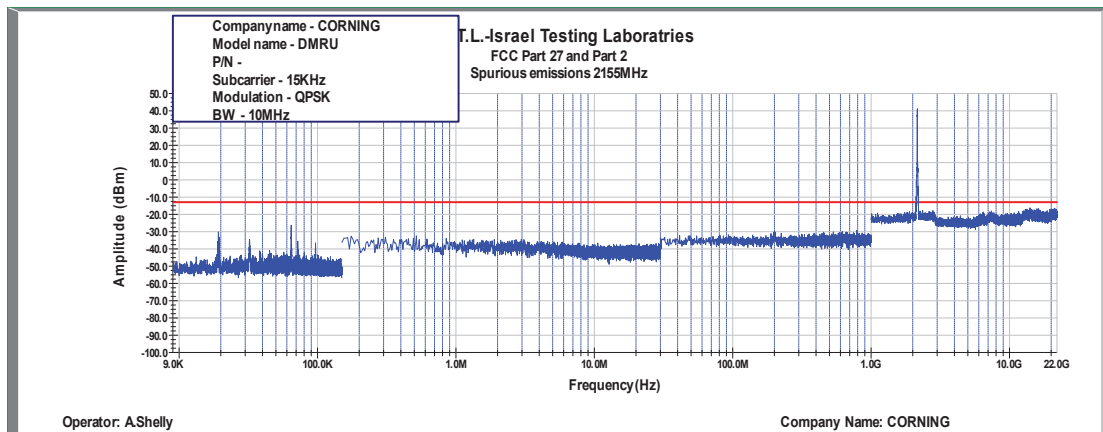
Figure 442: Spurious Emissions at Antenna Terminal QPSK, 2155MHz, B.W. 10MHz, Sub Carrier 15kHz
