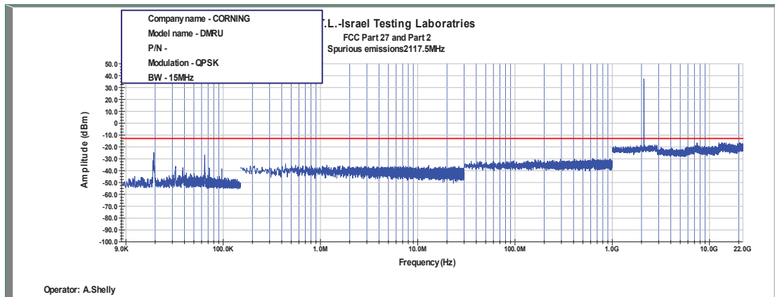
Figure 477: Spurious Emissions at Antenna Terminal QPSK, 2117.5MHz, B.W. 15MHz
