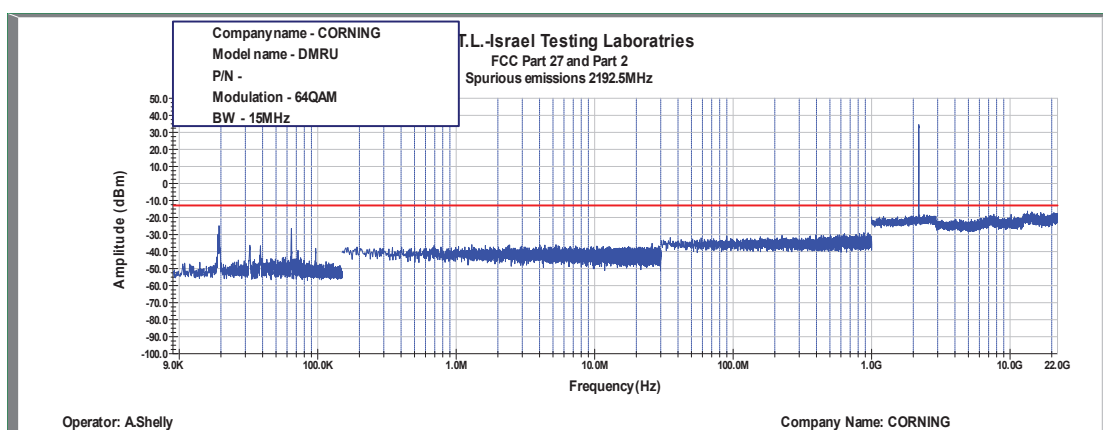
Figure 470: Spurious Emissions at Antenna Terminal 64QAM, 2192.5MHz, B.W. 15MHz
