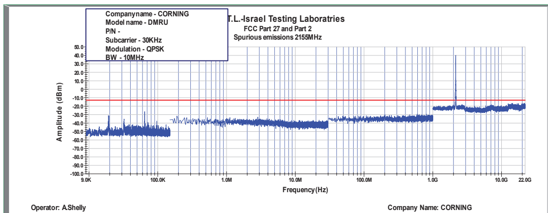
Figure 445: Spurious Emissions at Antenna Terminal QPSK, 2155MHz, B.W. 10MHz, Sub Carrier 30kHz
