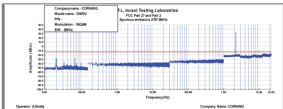
Figure 455: Spurious Emissions at Antenna Terminal 16QAM, 2197.5MHz, B.W. 5MHz
