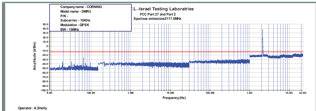
Figure 447: Spurious Emissions at Antenna Terminal QPSK, 2117.5MHz, B.W. 15MHz, Sub Carrier 15kHz
