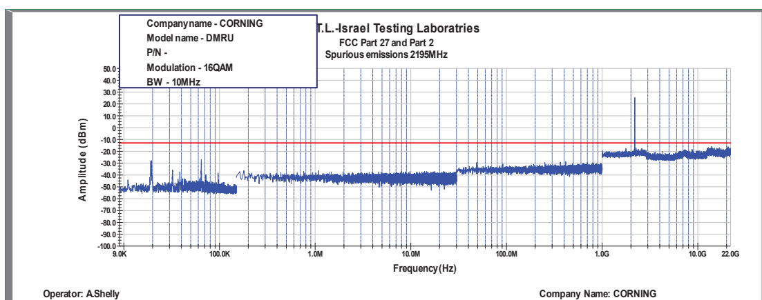
Figure 458: Spurious Emissions at Antenna Terminal 16QAM, 2195MHz, B.W. 10MHz
