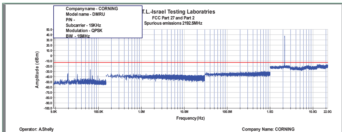
Figure 449: Spurious Emissions at Antenna Terminal QPSK, 2192.5MHz, B.W. 15MHz, Sub Carrier 15kHz
