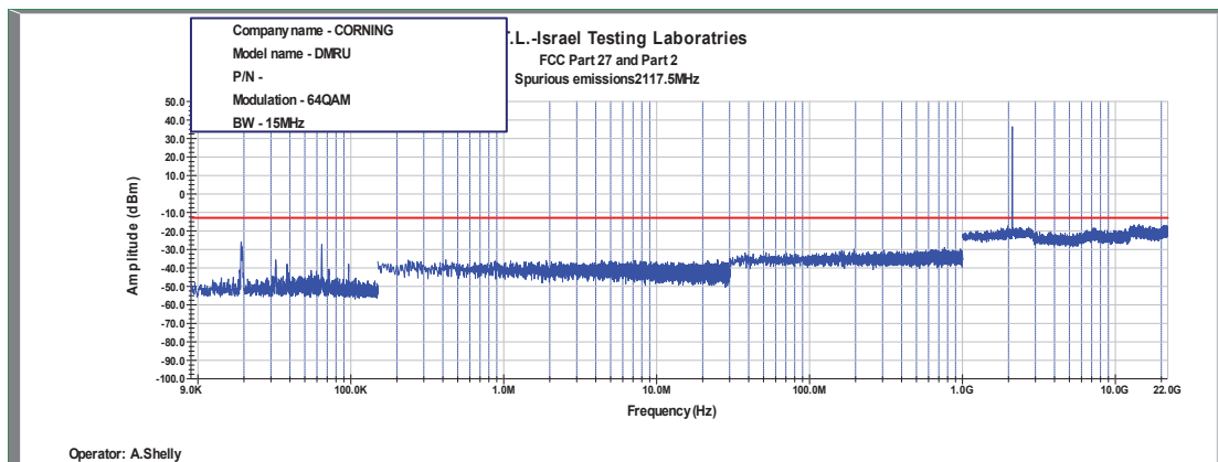
Figure 468: Spurious Emissions at Antenna Terminal 64QAM, 2117.5MHz, B.W. 15MHz
