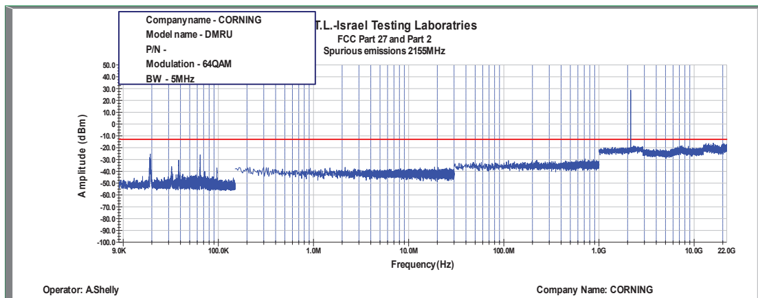
Figure 463: Spurious Emissions at Antenna Terminal 64QAM, 2155MHz, B.W. 5MHz
