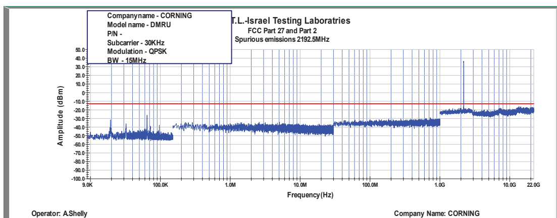
Figure 452: Spurious Emissions at Antenna Terminal QPSK, 2192.5MHz, B.W. 15MHz, Sub Carrier 30kHz
