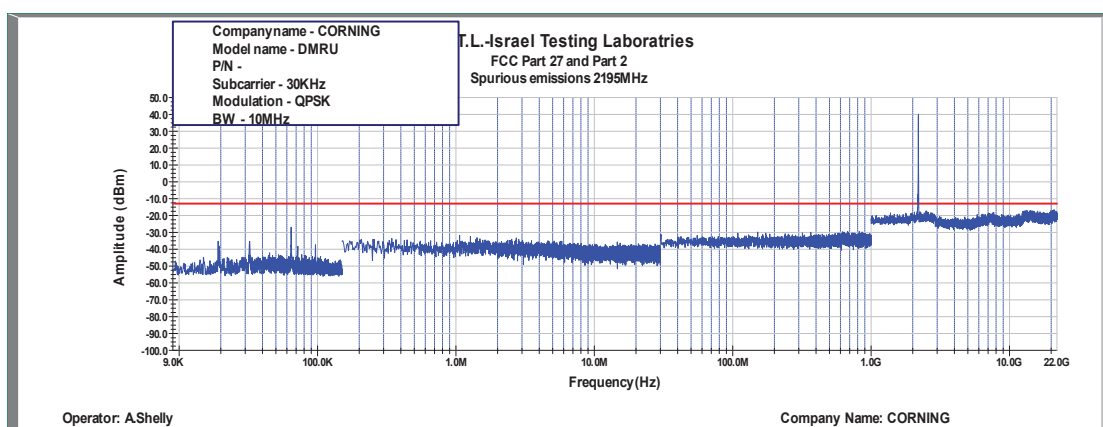
Figure 446: Spurious Emissions at Antenna Terminal QPSK, 2195MHz, B.W. 10MHz, Sub Carrier 30kHz
