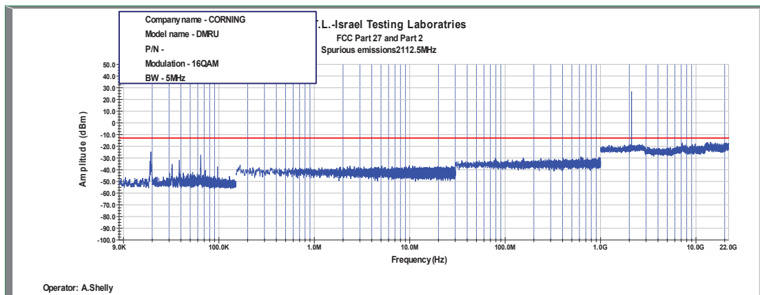
Figure 453: Spurious Emissions at Antenna Terminal 16QAM, 2112.5MHz, B.W. 5MHz
