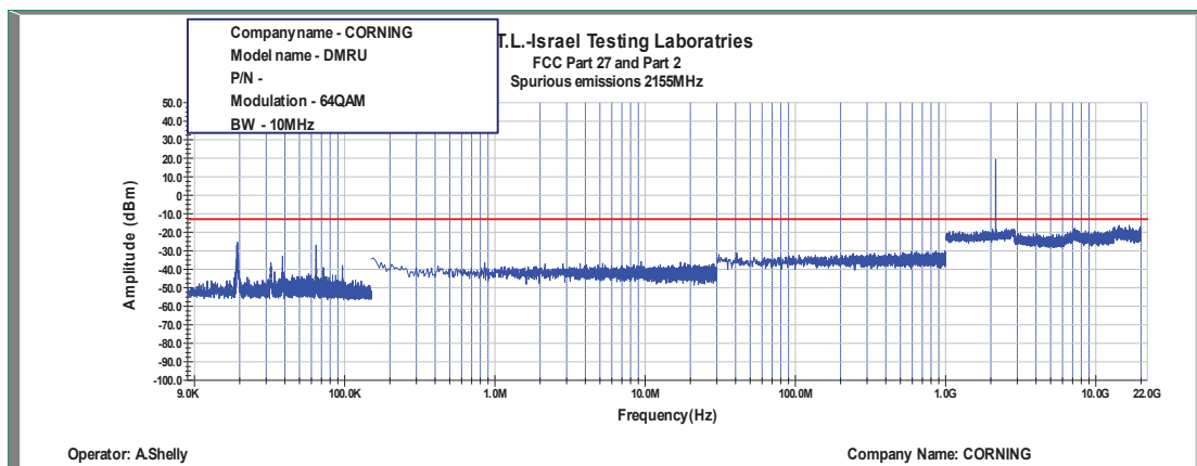
Figure 466: Spurious Emissions at Antenna Terminal 64QAM, 2155MHz, B.W. 10MHz
