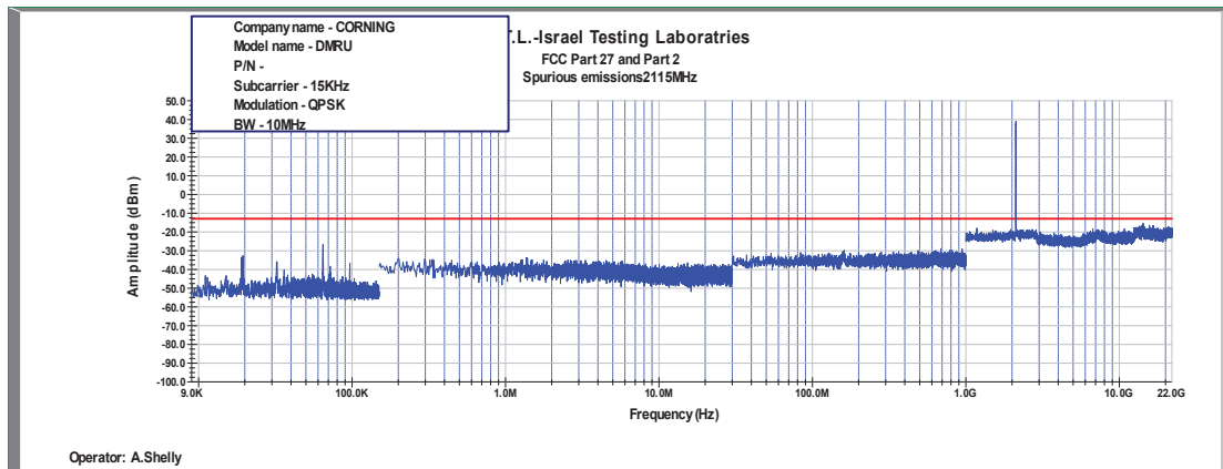
Figure 441: Spurious Emissions at Antenna Terminal QPSK, 2115MHz, B.W. 10MHz, Sub Carrier 15kHz
