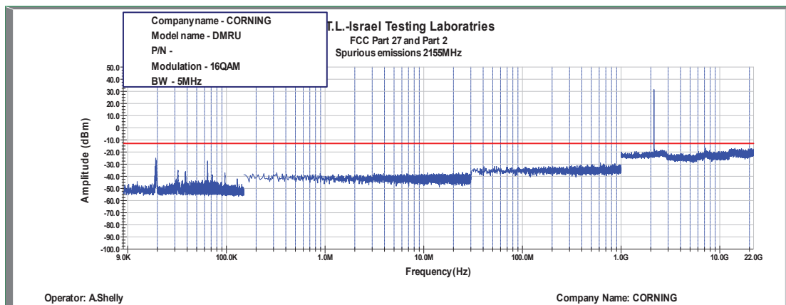
Figure 454: Spurious Emissions at Antenna Terminal 16QAM, 2155MHz, B.W. 5MHz
