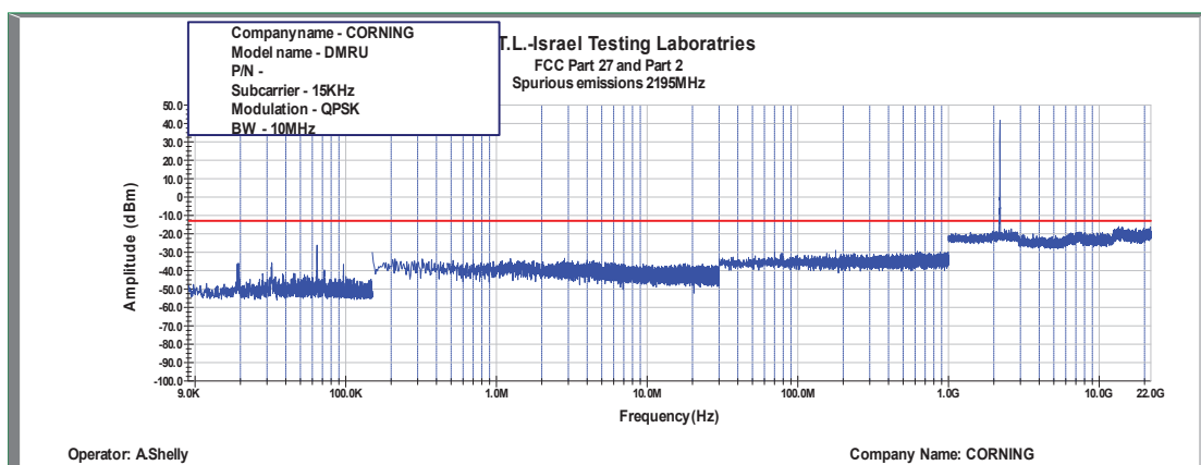
Figure 443: Spurious Emissions at Antenna Terminal QPSK, 2195MHz, B.W. 10MHz, Sub Carrier 15kHz
