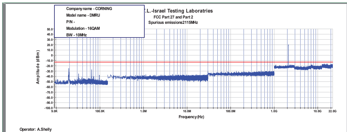
Figure 456: Spurious Emissions at Antenna Terminal 16QAM, 2115MHz, B.W. 10MHz
