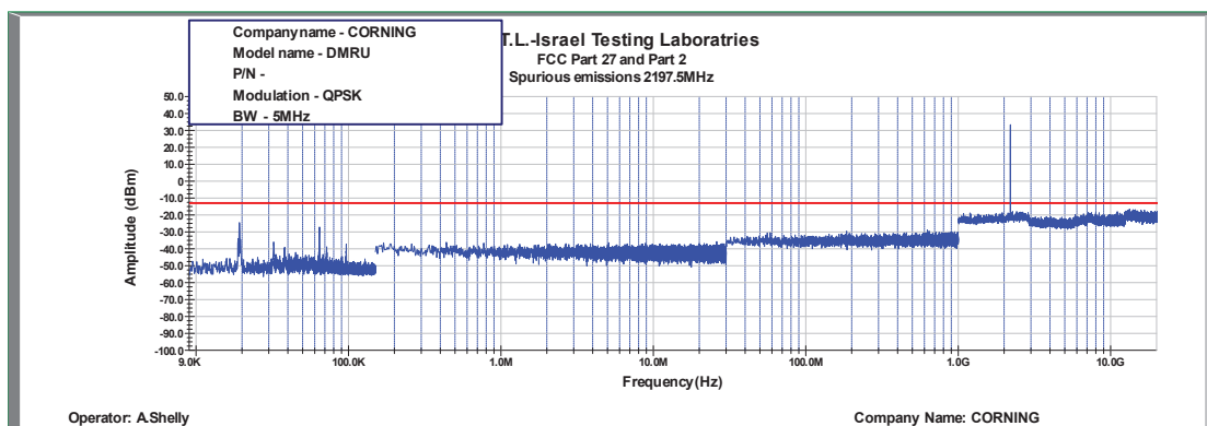
Figure 473: Spurious Emissions at Antenna Terminal QPSK, 2197.5MHz, B.W. 5MHz
