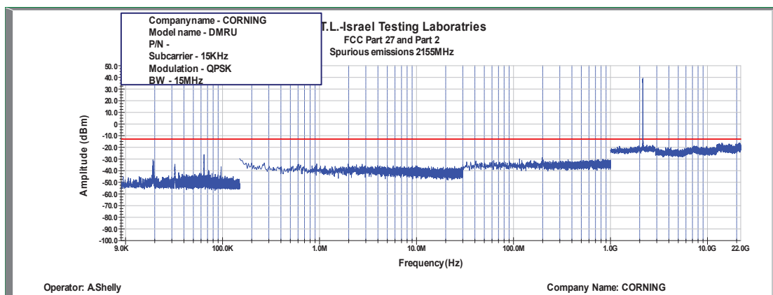
Figure 448: Spurious Emissions at Antenna Terminal QPSK, 2155MHz, B.W. 15MHz, Sub Carrier 15kHz
