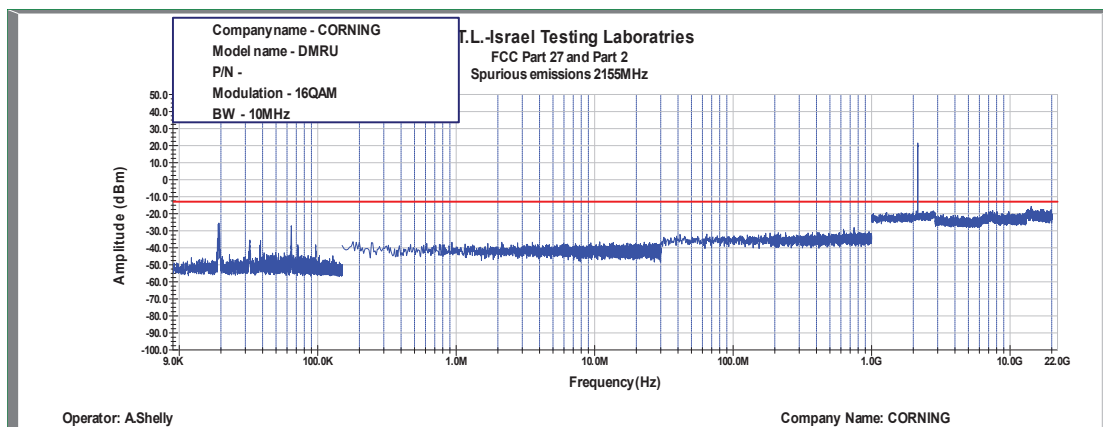
Figure 457: Spurious Emissions at Antenna Terminal 16QAM, 2155MHz, B.W. 10MHz
