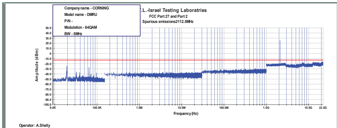
Figure 462: Spurious Emissions at Antenna Terminal 64QAM, 2112.5MHz, B.W. 5MHz
