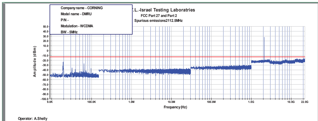
Figure 480: Spurious Emissions at Antenna Terminal WCDMA, 2112.5MHz, B.W. 5MHz
