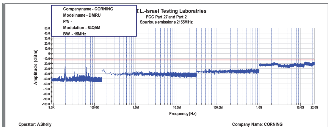
Figure 469: Spurious Emissions at Antenna Terminal 64QAM, 2155MHz, B.W. 15MHz
