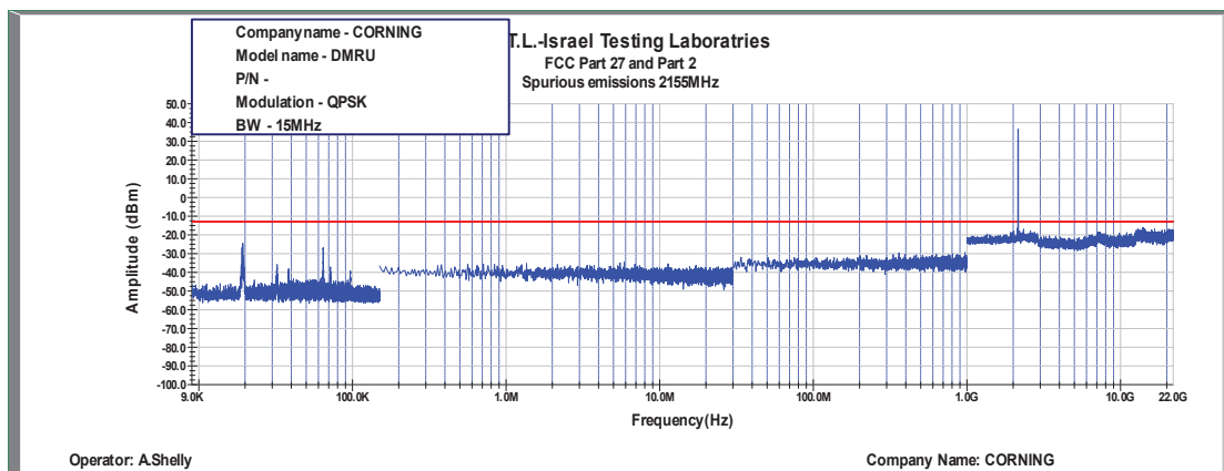
Figure 478: Spurious Emissions at Antenna Terminal QPSK, 2155MHz, B.W. 15MHz
