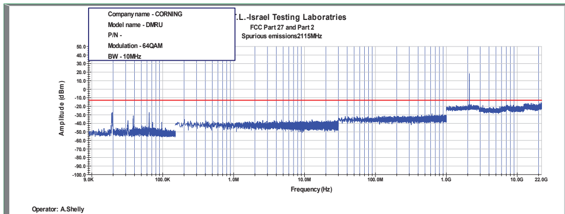
Figure 465: Spurious Emissions at Antenna Terminal 64QAM, 2115MHz, B.W. 10MHz
