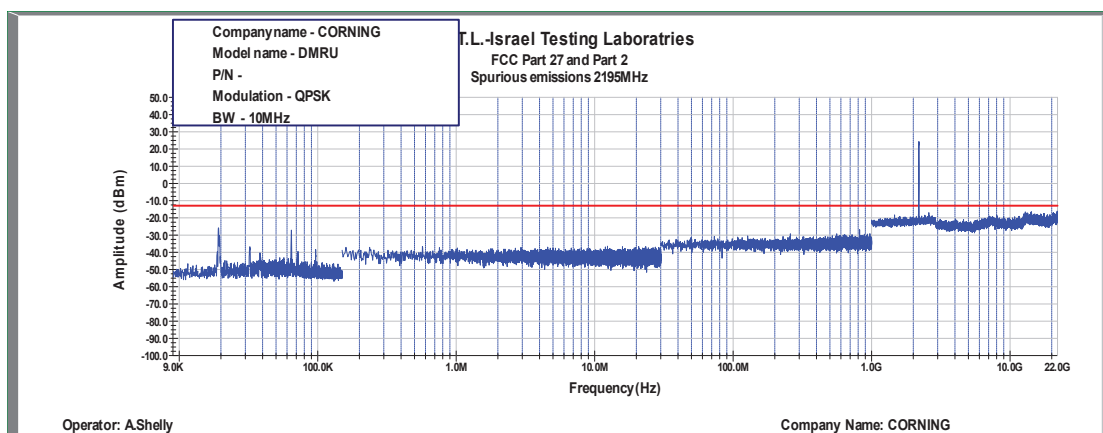
Figure 476: Spurious Emissions at Antenna Terminal QPSK, 2195MHz, B.W. 10MHz
