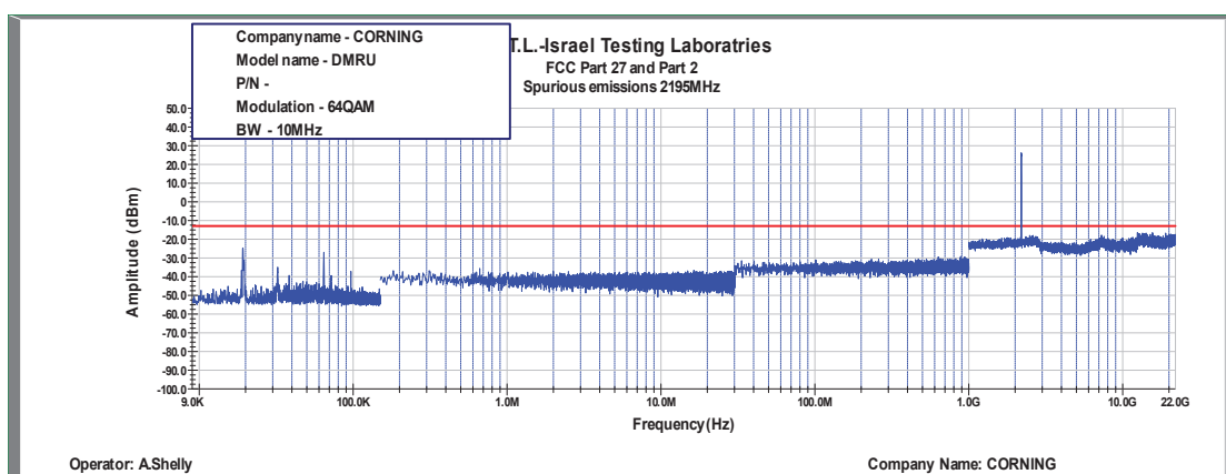
Figure 467: Spurious Emissions at Antenna Terminal 64QAM, 2195MHz, B.W. 10MHz
