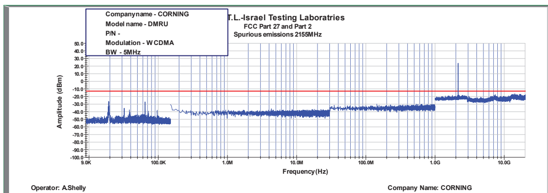
Figure 481: Spurious Emissions at Antenna Terminal WCDMA, 2155MHz, B.W. 5MHz
