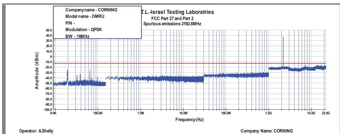
Figure 479: Spurious Emissions at Antenna Terminal QPSK, 2192.5MHz, B.W. 15MHz
