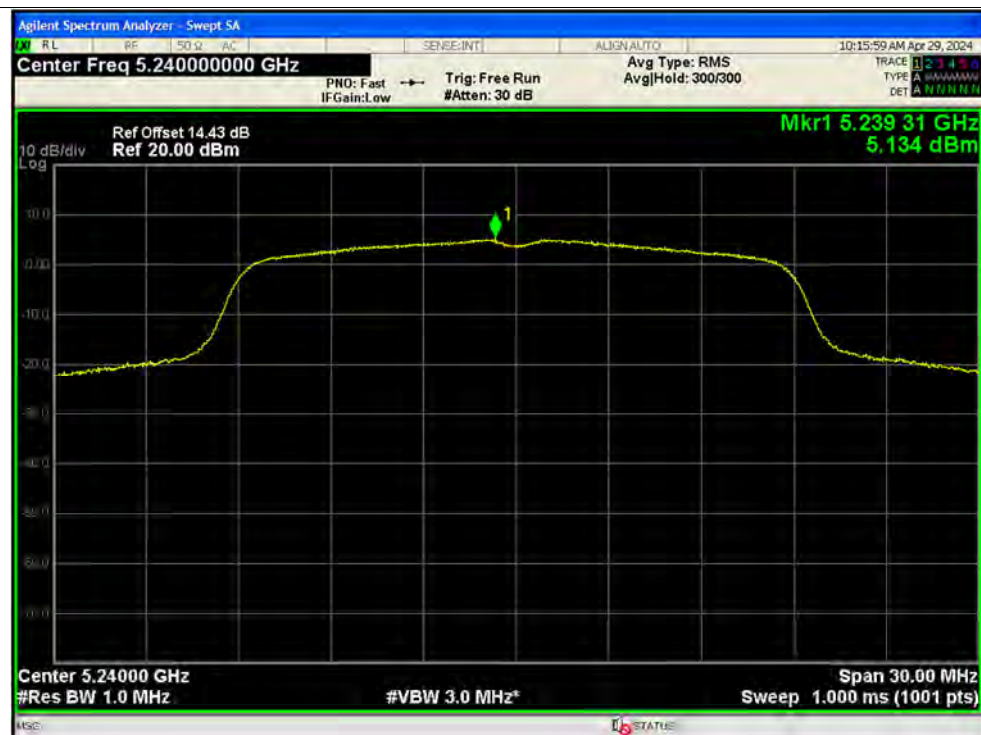
PSD NVNT ac20 5240MHz Ant2 MIMO
