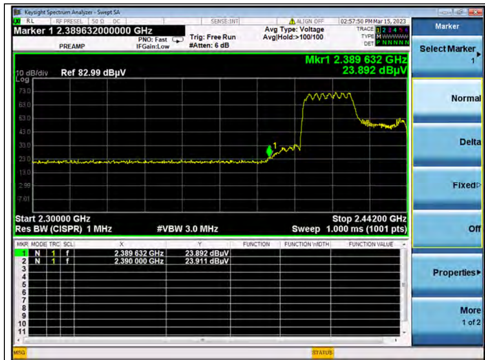
(PEAK, Channel 3, 802.11ax (HEW40) RU242)
