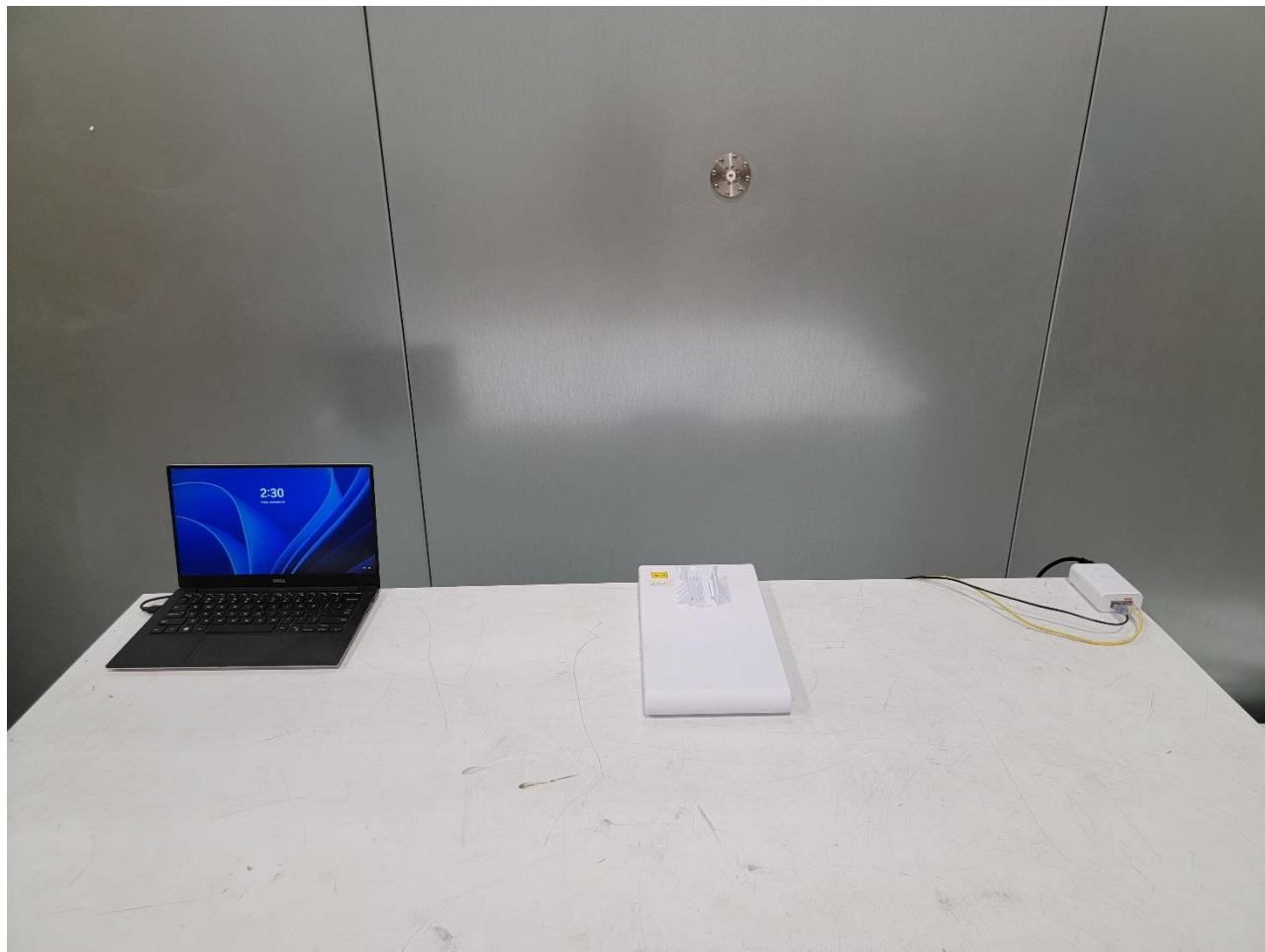
Photograph 5: View Test Set Up Front of Conducted Emissions
