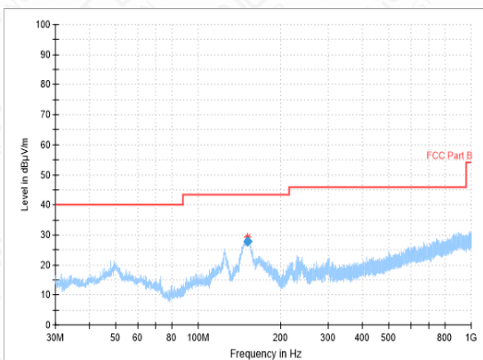
RSE-11G-CH11-30MHz-1GHz
