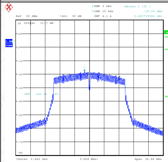
11N20SISO-Ant1-2462-PASS
