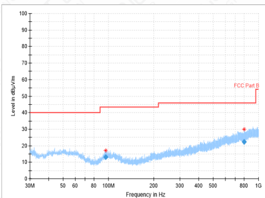
RSE-11G-CH1-30MHz-1GHz
