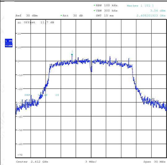
11G-Ant1-2412-0~Reference-PASS
