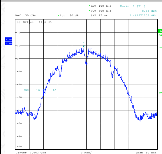
11B-Ant1-2462-0~Reference-PASS
