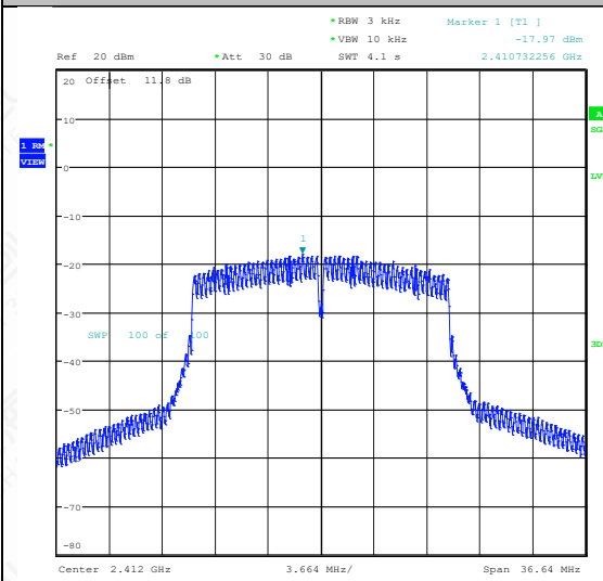
11N20SISO-Ant1-2412-PASS
