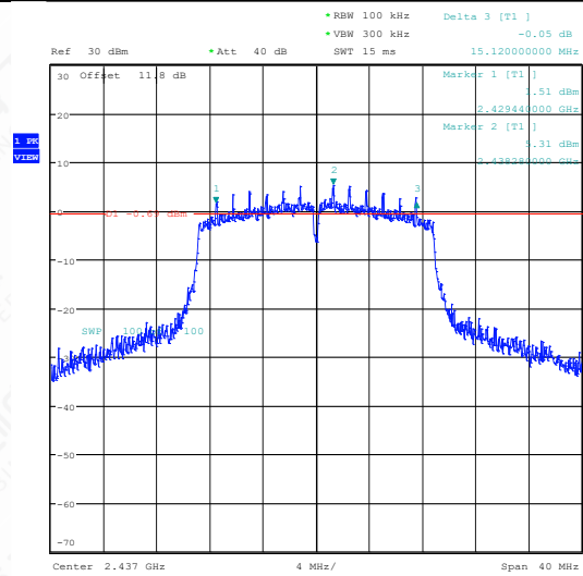
11N20SISO-Ant1-2437-PASS
