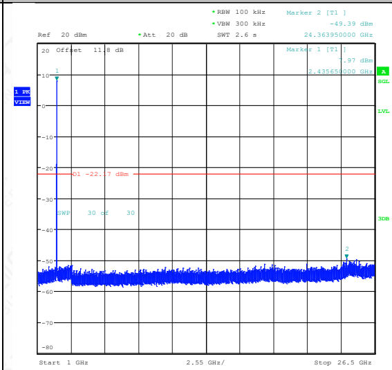
11B-Ant1-2437-1000~26500-PASS
