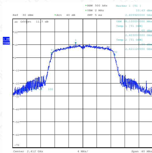
11N20SISO-Ant1-2412
