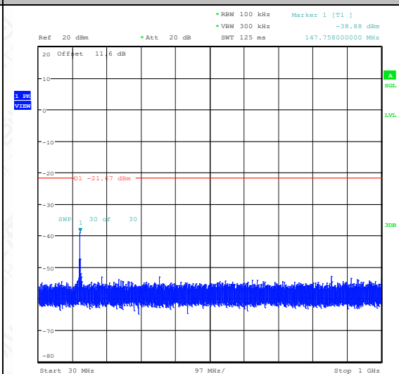
11B-Ant1-2462-30~1000-PASS
