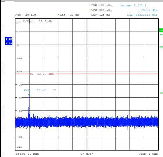
11B-Ant1-2437-30~1000-PASS
