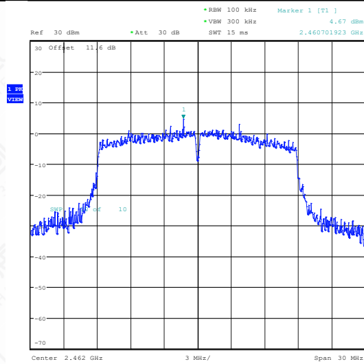
11N20SISO-Ant1-2462-0~Reference-PASS
