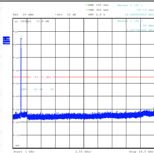
11N20SISO-Ant1-2462-1000~26500-PASS
