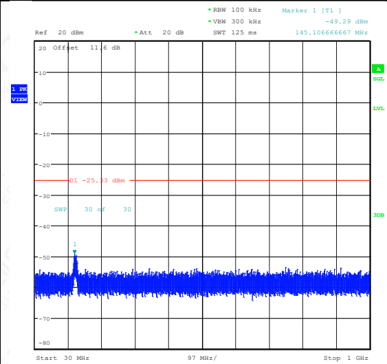
11N20SISO-Ant1-2462-30~1000-PASS
