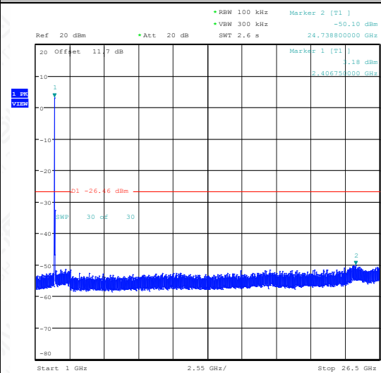
11G-Ant1-2412-1000~26500-PASS
