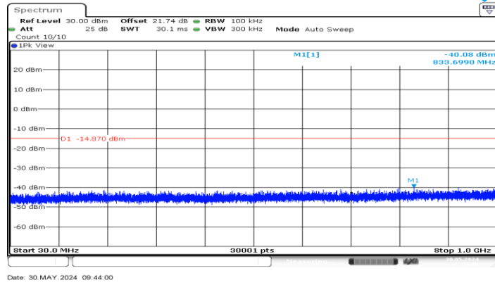
BLE_2M_Ant1_2402_30~1000
