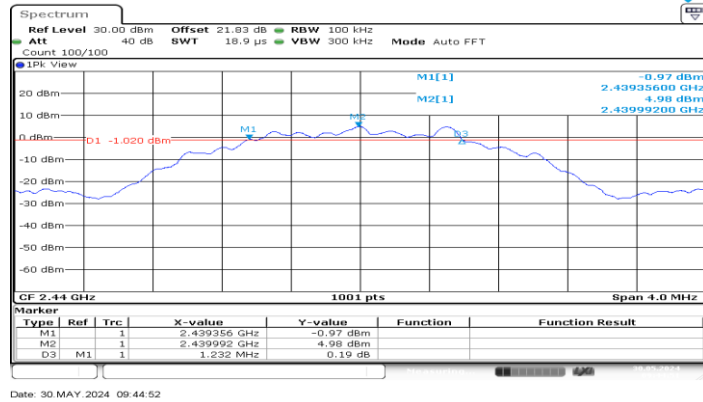
BLE_2M_Ant1_2440
