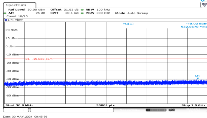
BLE_2M_Ant1_2440_0~Reference
