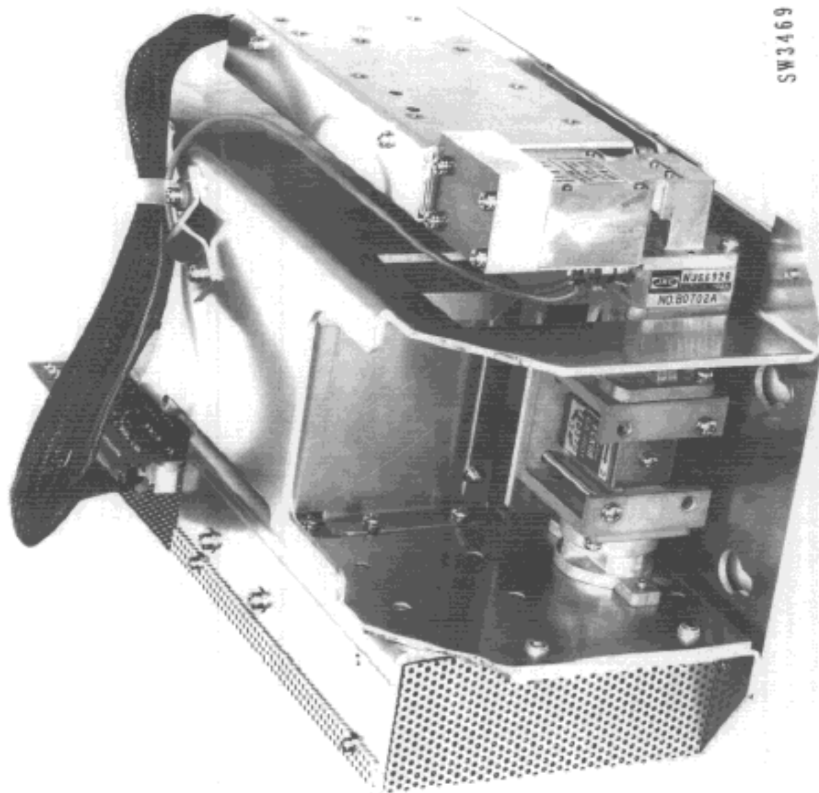
PHOTO. 21 TRANCEIVER ASSEMBLY OF SCANNER UNIT NKE-1055
