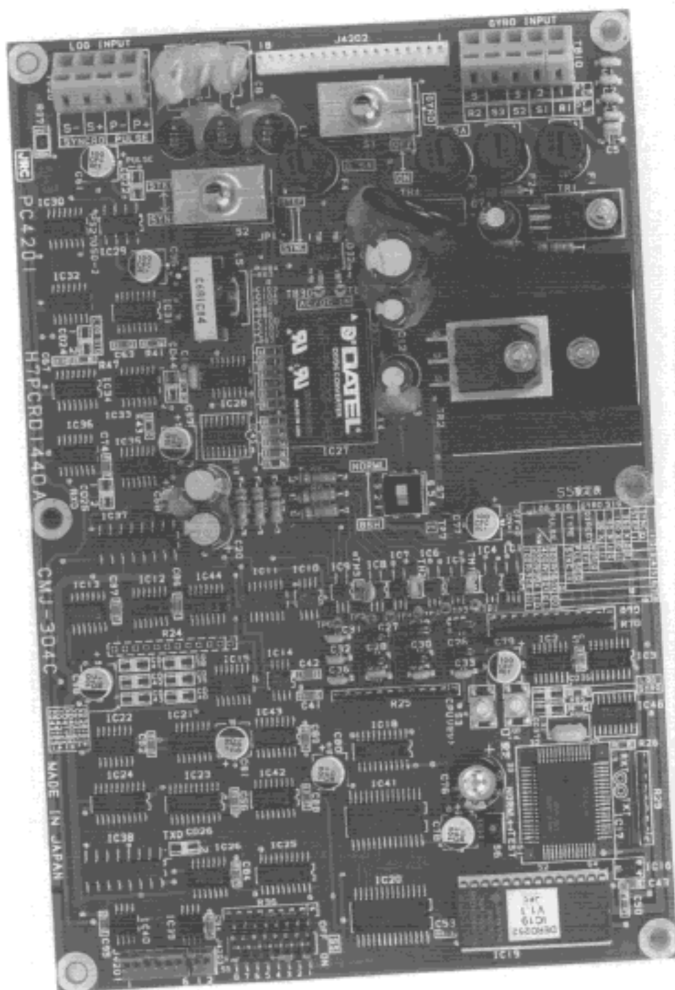
PHOTO. 19 NSK CIRCUIT CMJ-304C
