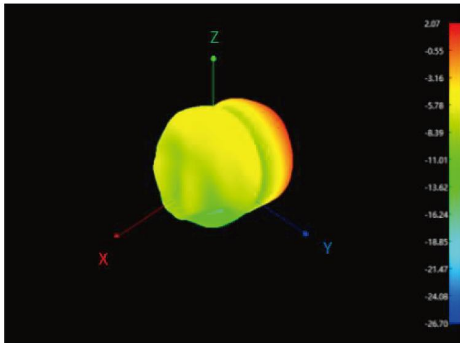
2440MHz 3D
