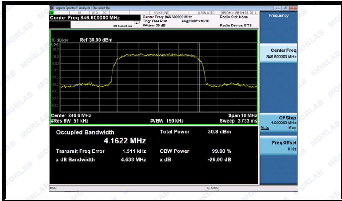
(Plot O: HSDPA 850 MHz Channel = 4233)
