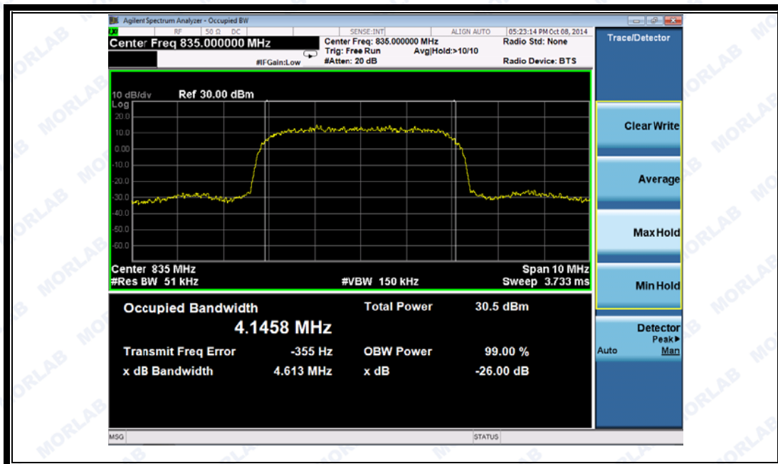
(Plot T: HSUPA850 MHz Channel = 4175)
