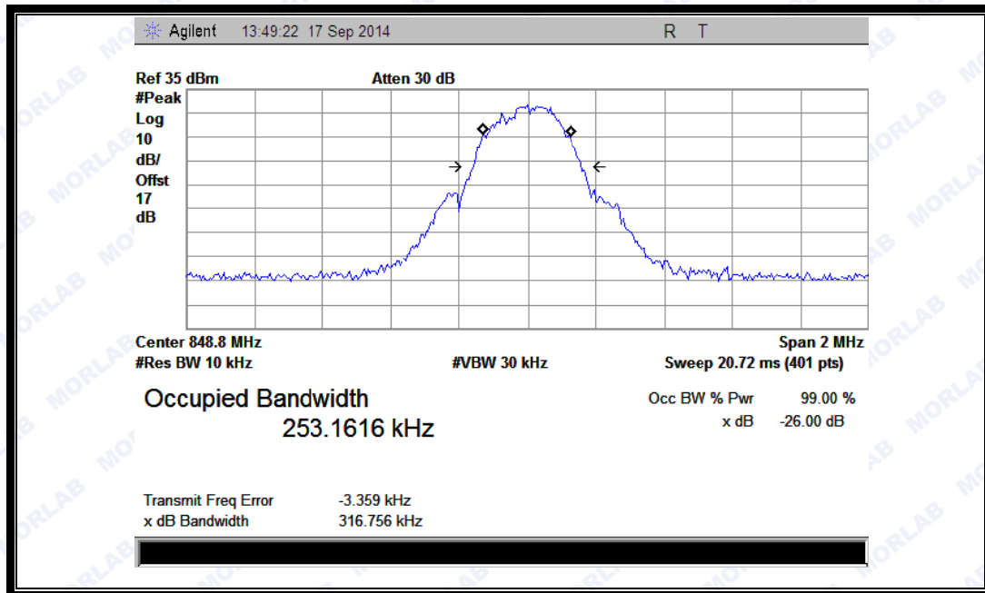
(Plot G1: GSM 850MHz Channel = 251)
