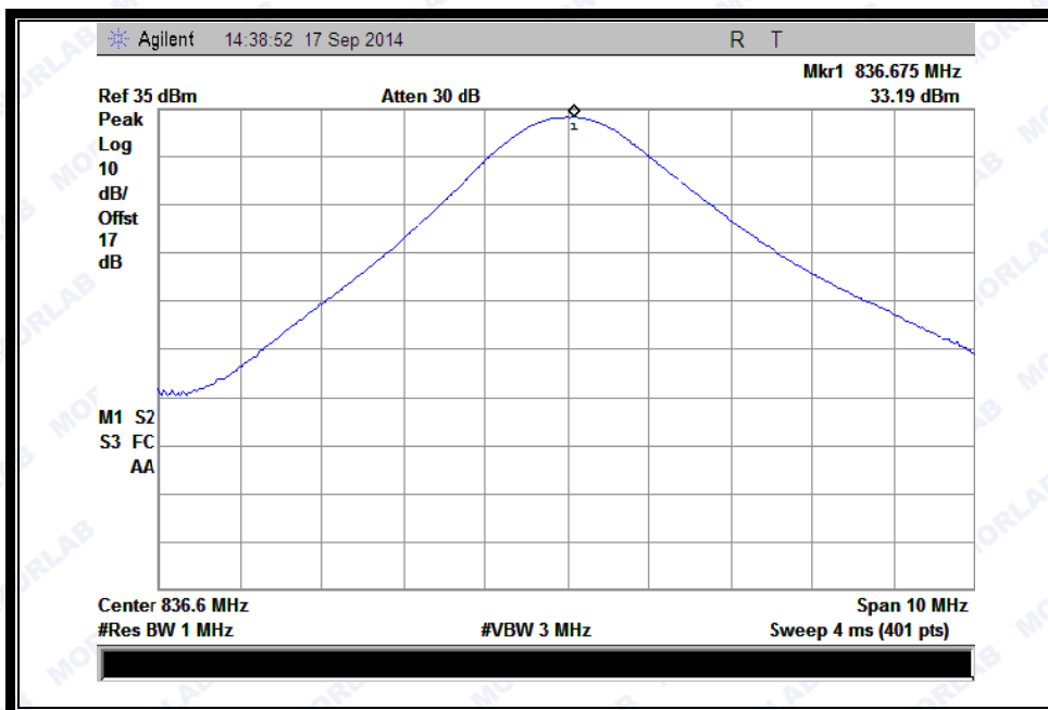
(Plot A2:GSM 850MHz Channel = 190)
