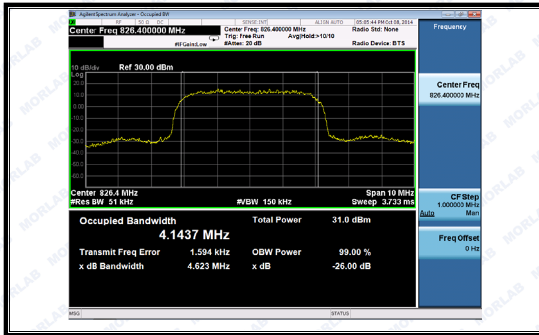
(Plot M: HSDPA 850MHz Channel = 4132)
