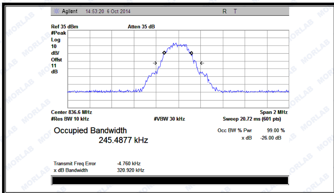
(Plot L1: GPRS 850MHz Channel = 190)
