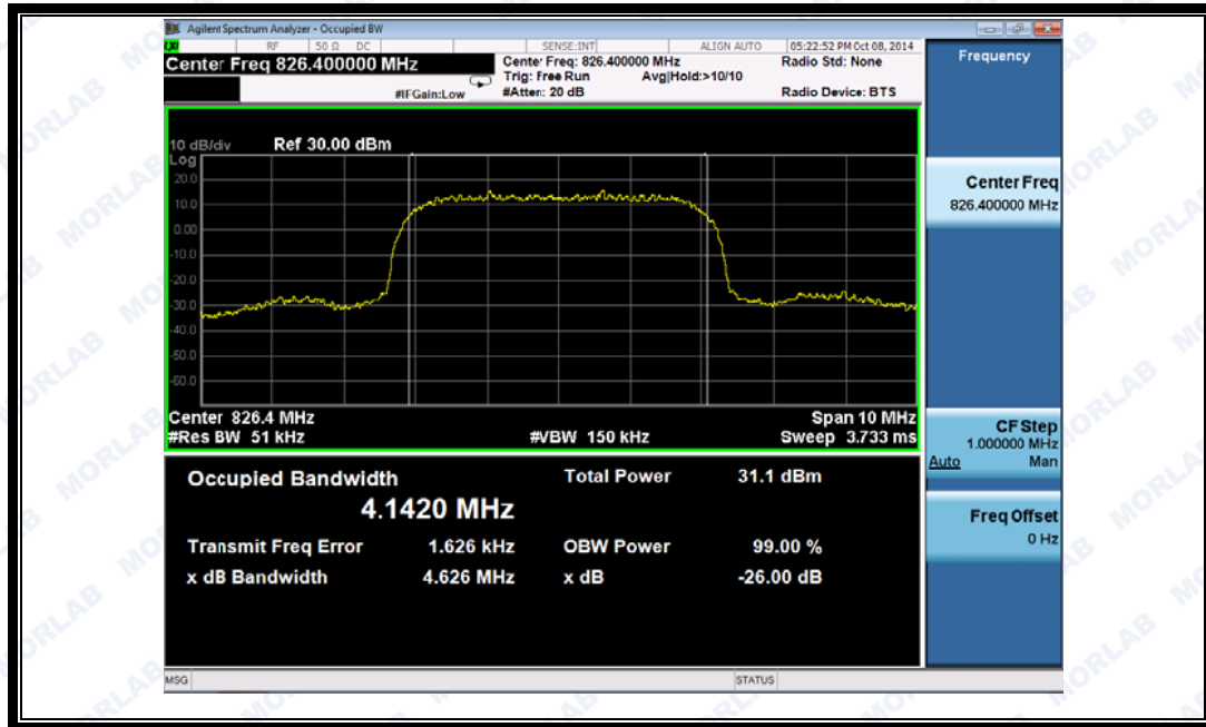
(Plot S: HSUPA850 MHz Channel = 4132)
