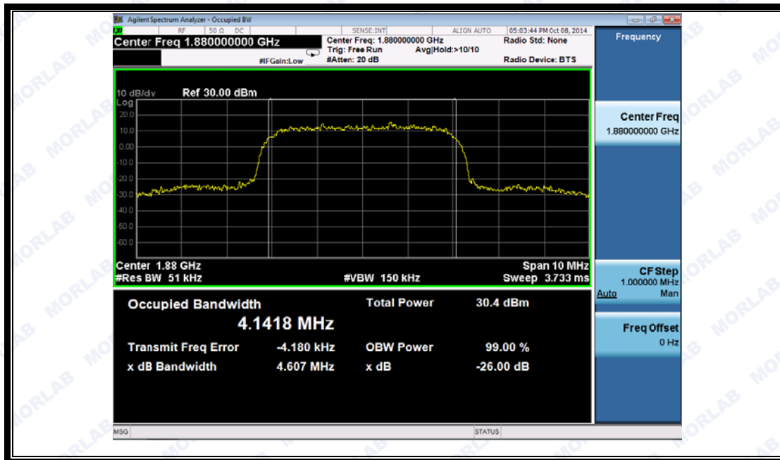
(Plot Q: HSDPA1900 MHz Channel = 9400)
