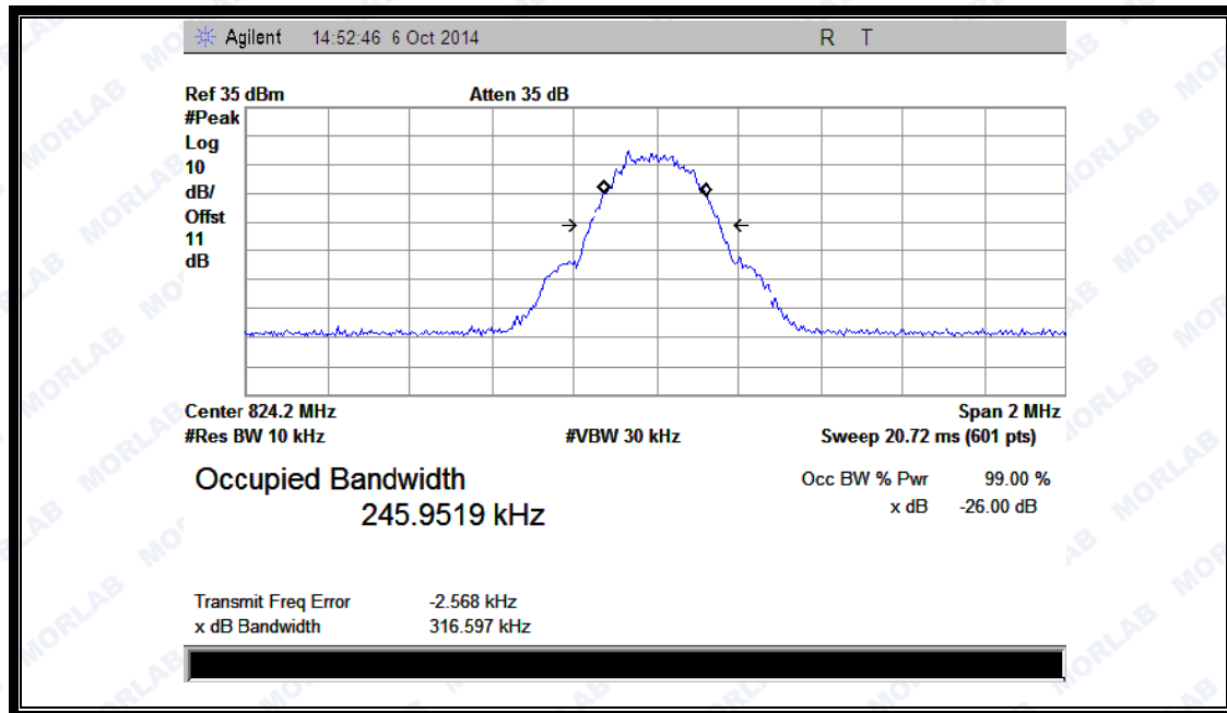
(Plot K1: GPRS 850MHz Channel = 128)
