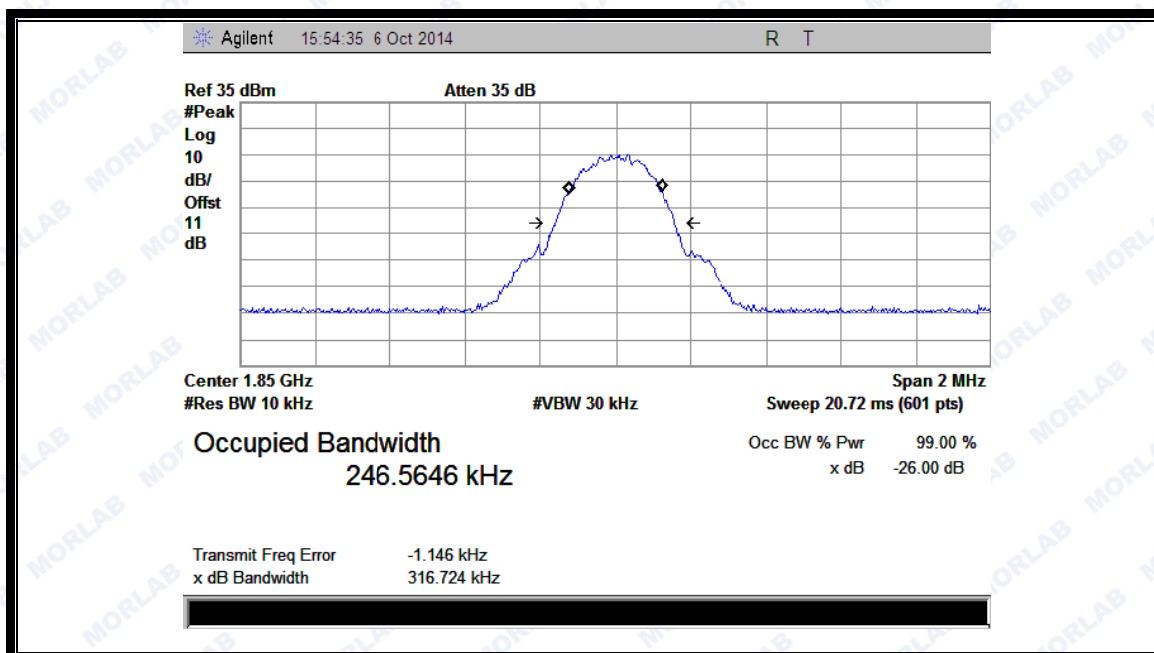
(Plot N1: GPRS 1900MHz Channel = 512)
