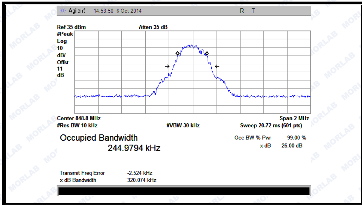
(Plot M1: GPRS850MHz Channel = 251)
