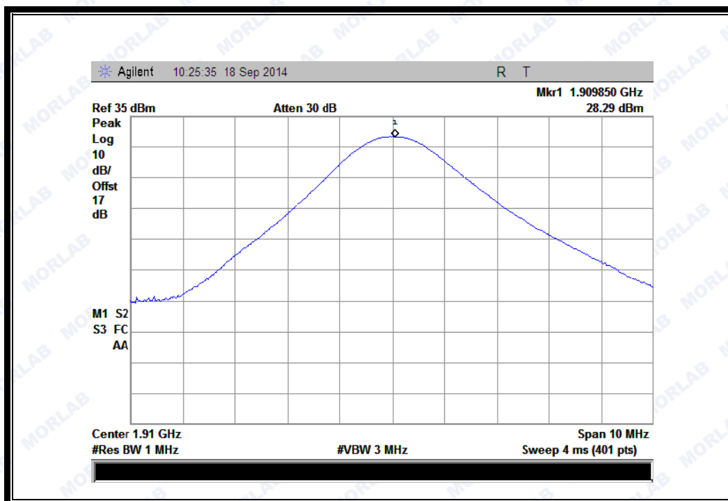
(Plot F3:EGPRS 1900Hz Channel = 810)
