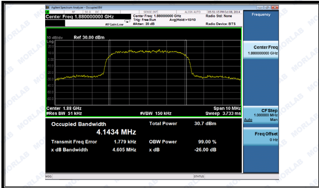
(Plot C1: HSPA+1900 MHz Channel = 9400)
