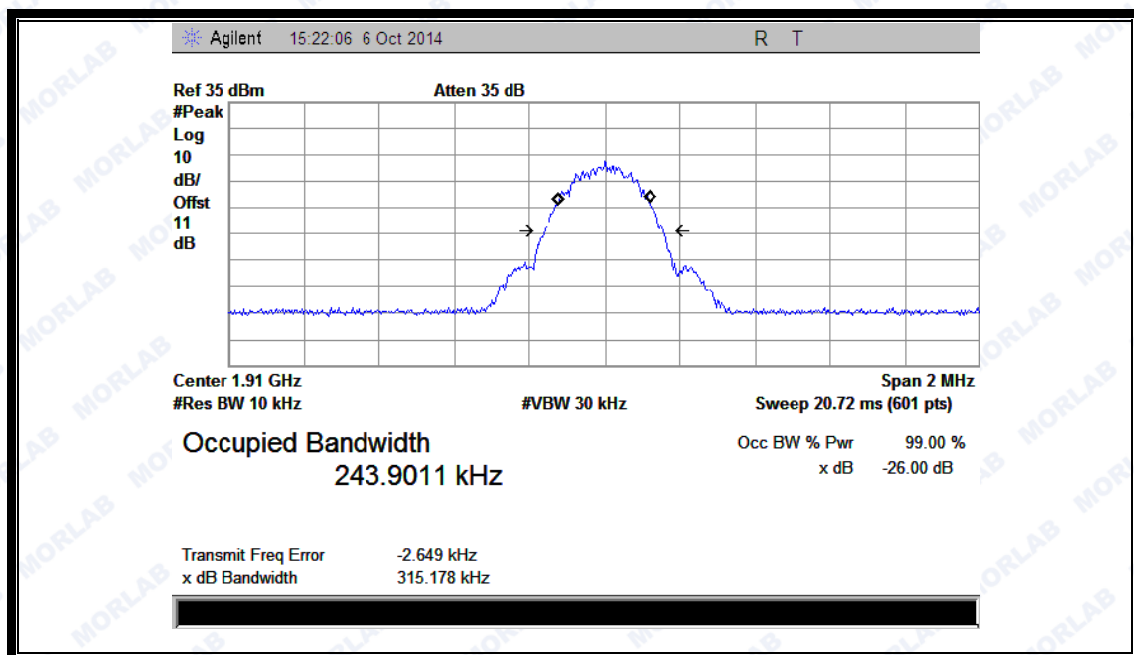
(Plot P1: GPRS 1900MHz Channel = 810)
