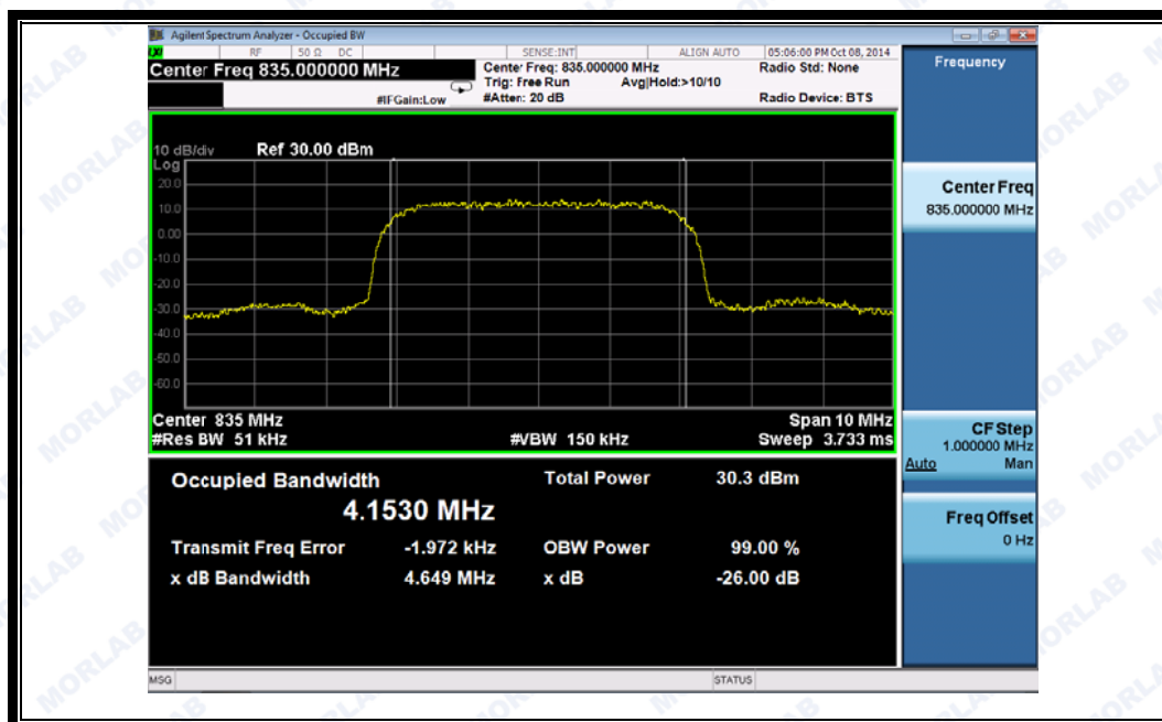
(Plot N: HSDPA850 MHz Channel = 4175)
