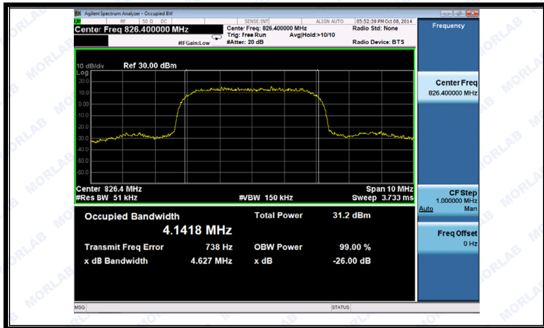
(Plot Y: HSPA+850 MHz Channel = 4132)
