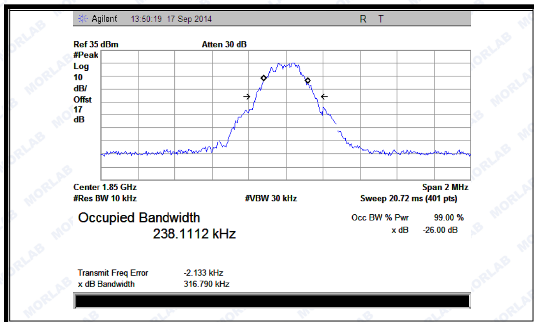
(Plot H1: GSM 1900MHz Channel = 512)
