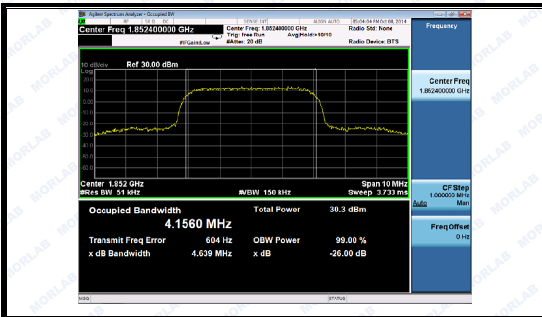
(Plot P: HSDPA1900 MHz Channel = 9262)
