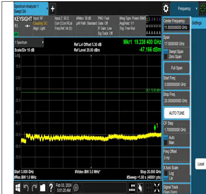
Band66_1.4MHz_QPSK_131979_1RB#0_3000~20000_3000~20000
