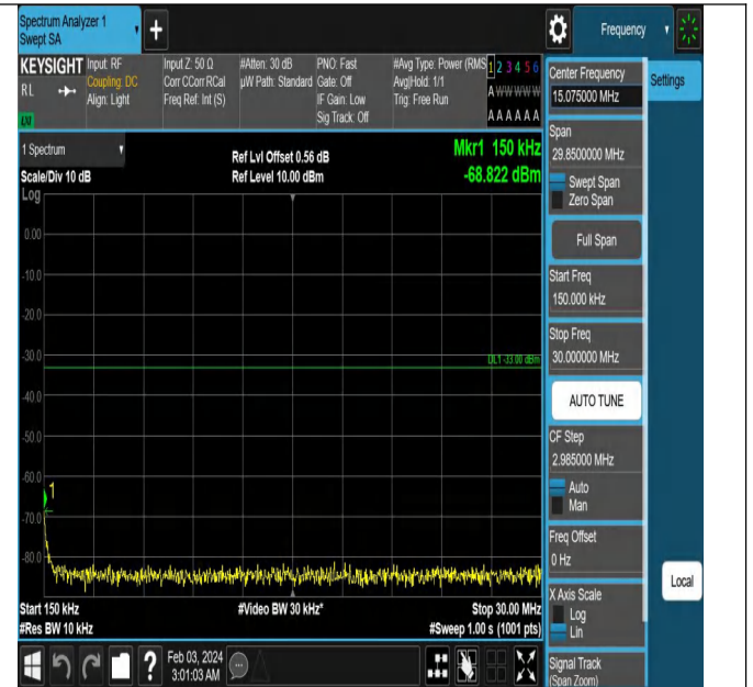
Band66_1.4MHz_QPSK_131979_1RB#0_0.15~30_0.15~30
