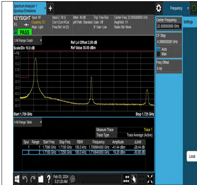
Band66_15MHz_QPSK_132047_1RB#0
