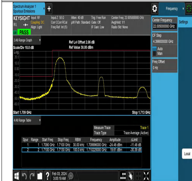
Band66_3MHz_QPSK_131987_1RB#0
