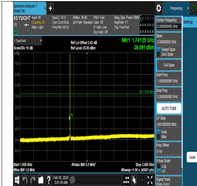
Band66_1.4MHz_QPSK_132322_1RB#0_1000~3000_1000~3000
