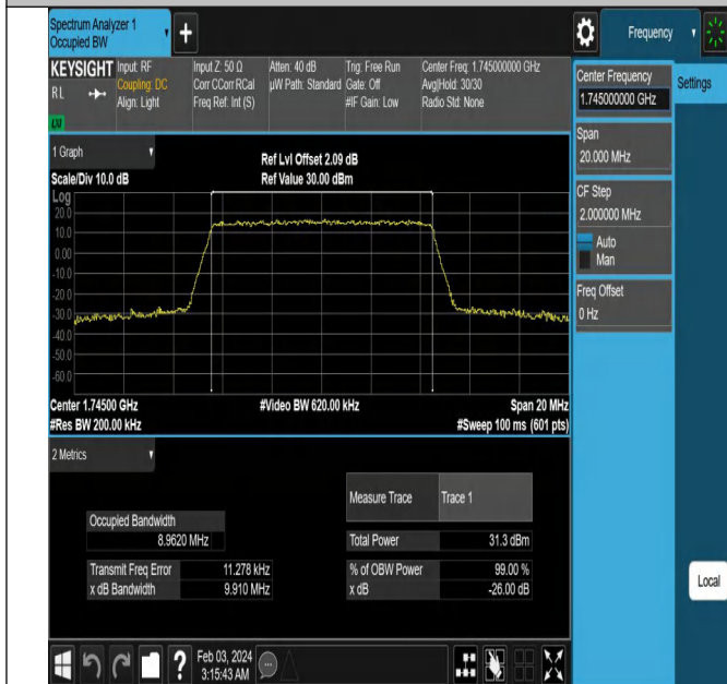
Band66-10MHz-QPSK-132322-50RB#0-PASS
