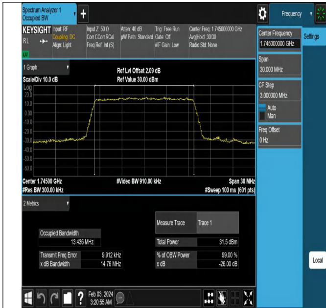
Band66-15MHz-QPSK-132322-75RB#0-PASS
