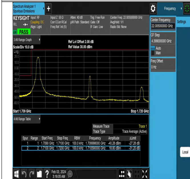
Band66_10MHz_QPSK_132022_1RB#0
