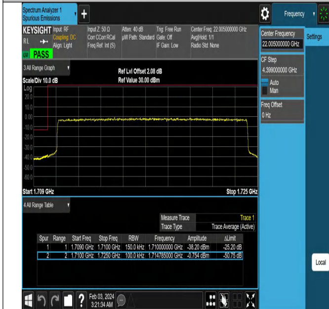
Band66_15MHz_QPSK_132047_75RB#0
