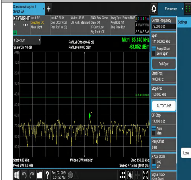
Band66_1.4MHz_QPSK_132665_1RB#0_0.009~0.15_0.009~0.15
