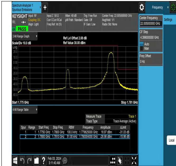
Band66_5MHz_QPSK_132647_1RB#24
