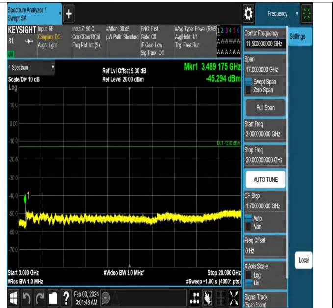
Band66_1.4MHz_QPSK_132322_1RB#0_3000~20000_3000~20000
