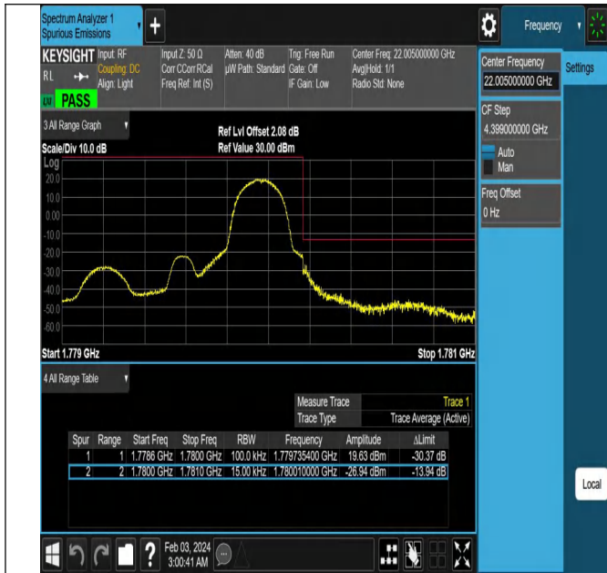
Band66_1.4MHz_QPSK_132665_1RB#5
