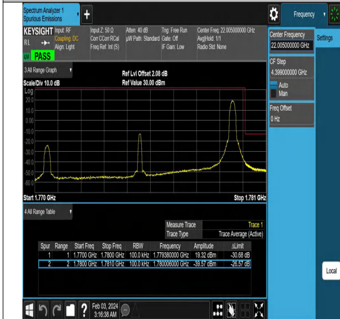
Band66_10MHz_QPSK_132622_1RB#49
