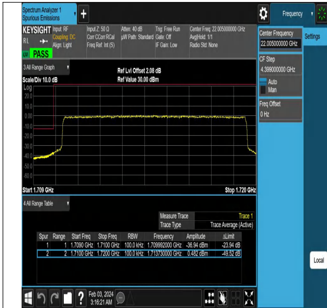
Band66_10MHz_QPSK_132022_50RB#0
