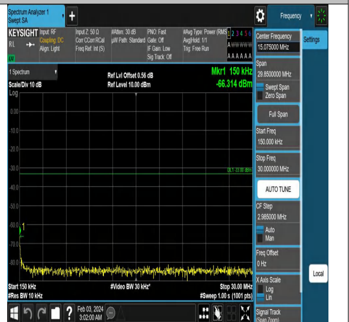
Band66_1.4MHz_QPSK_132665_1RB#0_0.15~30_0.15~30
