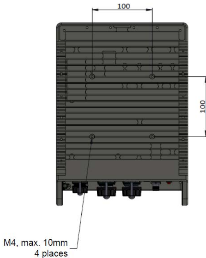
Figure 6: Pearl Mobile Gateway Module Mounting Points
