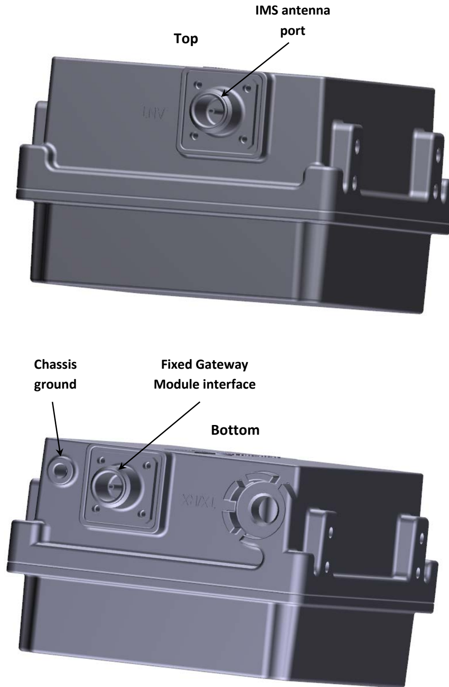
Figure 5: Pearl TTU Module Interconnect
