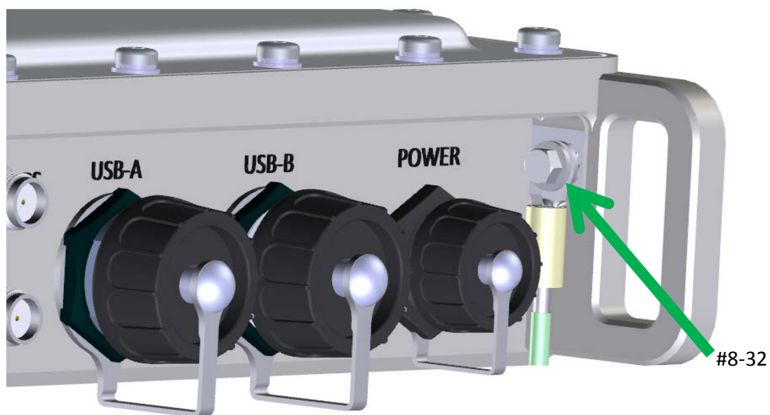
Figure 26: Module de passerelle mobile Pearl Ground Point
