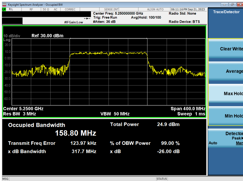
Plot 7-37. 26dB Bandwidth Plot MIMO ANT2 (160MHz BW 802.11be – 2x996 Tones (UNII Band ½A) – Ch. 50)
