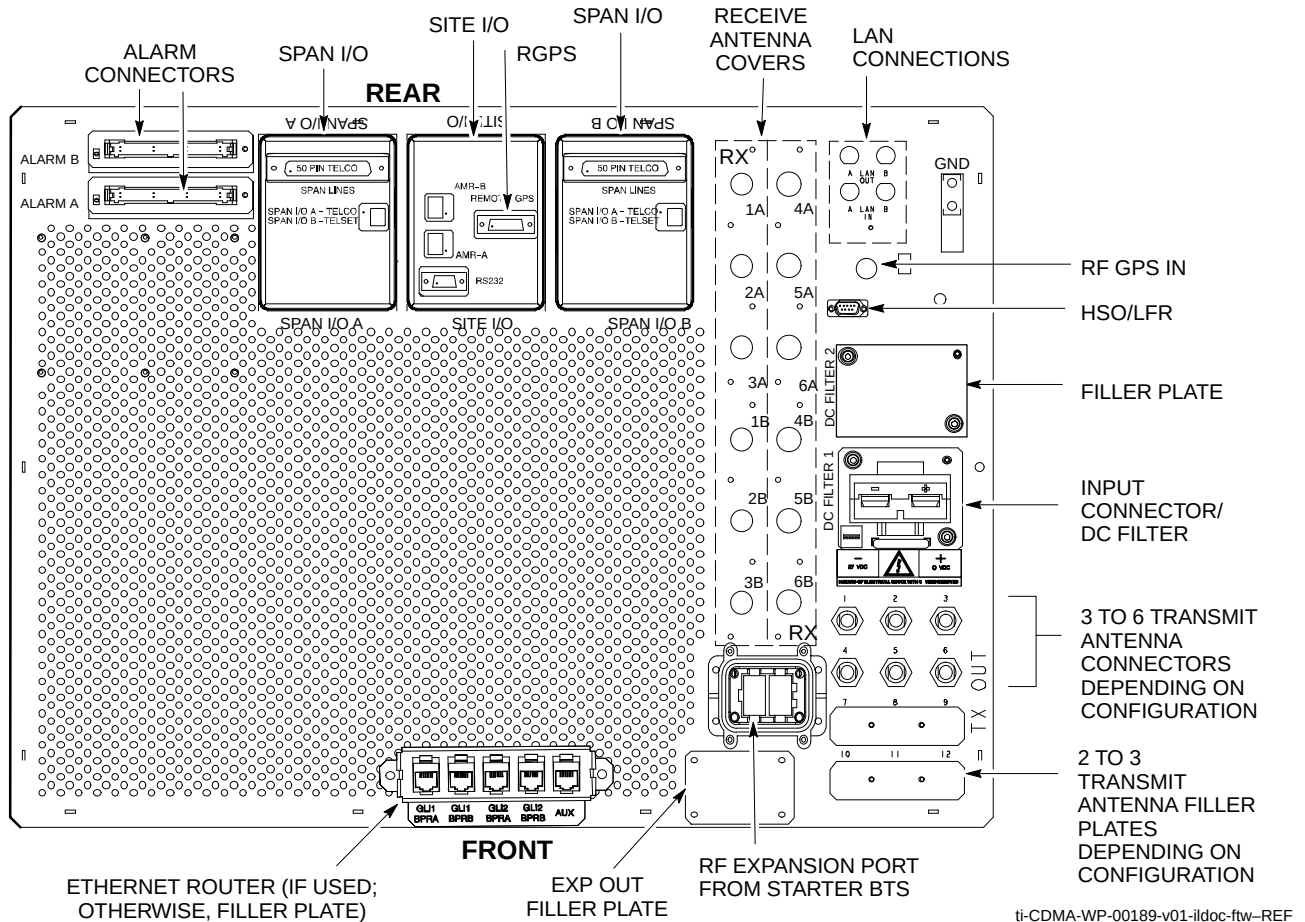
Figure 2-2: SC4812T-MC Expansion Frame I/O Plate
