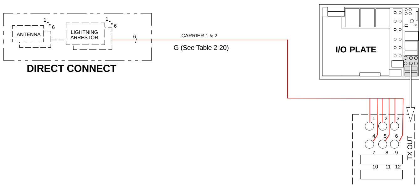
Figure 2-12: 60 Degree Sector (6 Sector) Transmit Path Cabling Details (Outside Frame)
