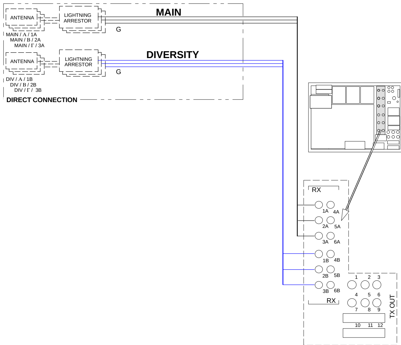
Figure 2-17: 120 Degree Sector (3 Sector) Receive Path Cabling Details
