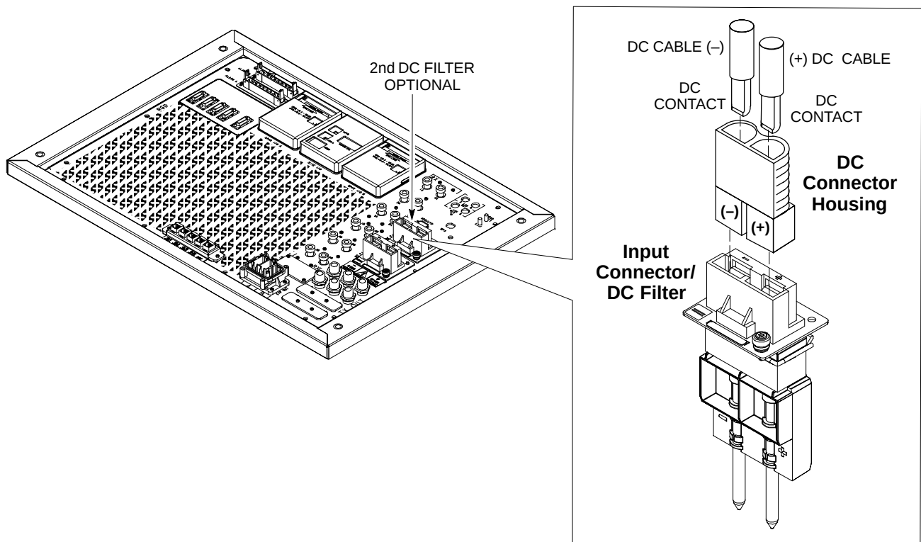
Figure 2-23: DC Power Connector/Filter
