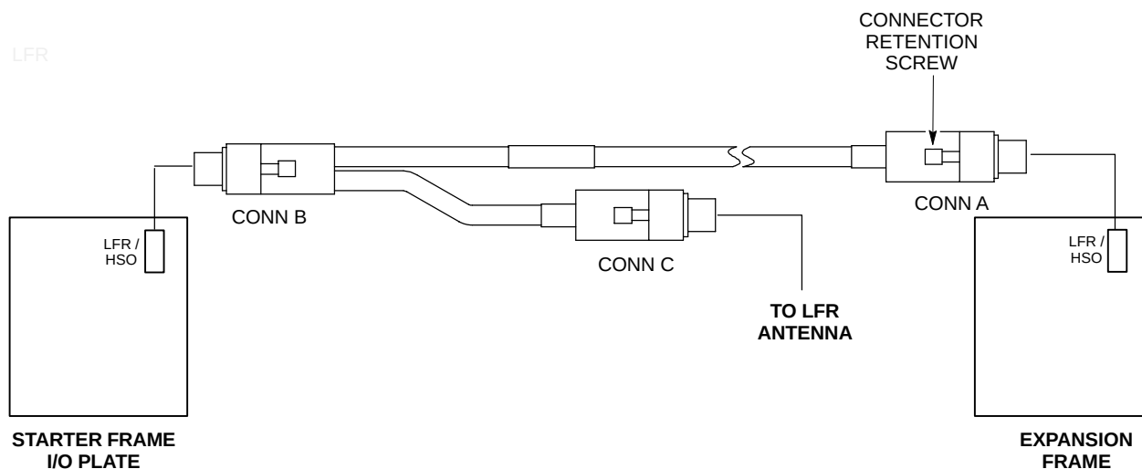
Figure 3-8: HSOX Cable (3086458H01) for Expansion Frame
