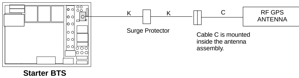
Figure 2-9: RF GPS Cabling Detail
