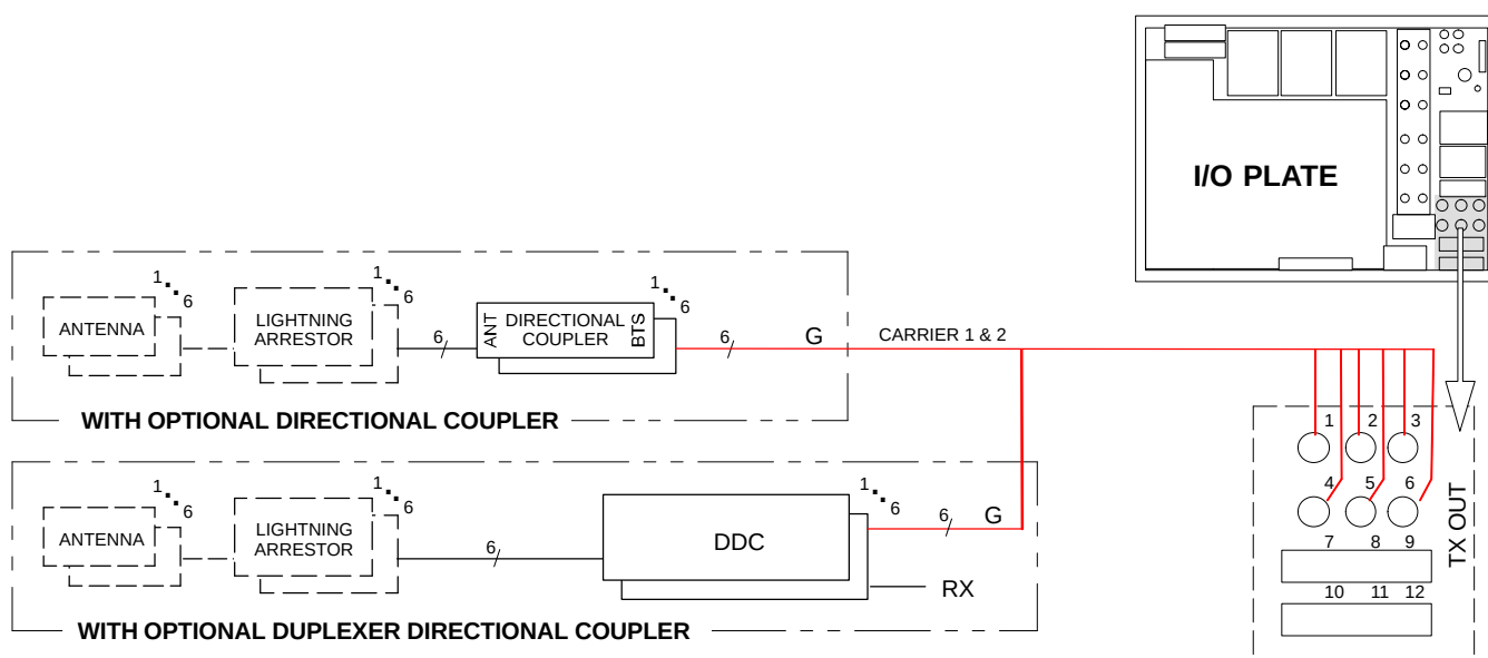
Figure 4-5: 60 Degree Sector (6 Sector) Transmit Path Cabling Details
