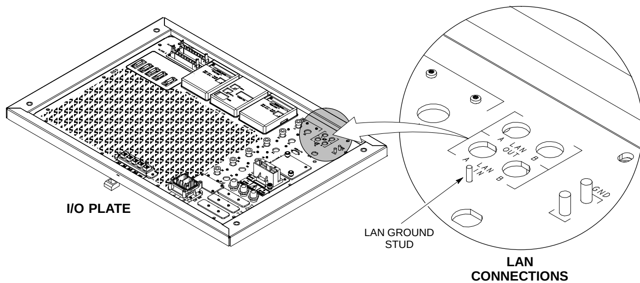
Figure 3-9: LAN Grounding Stud
