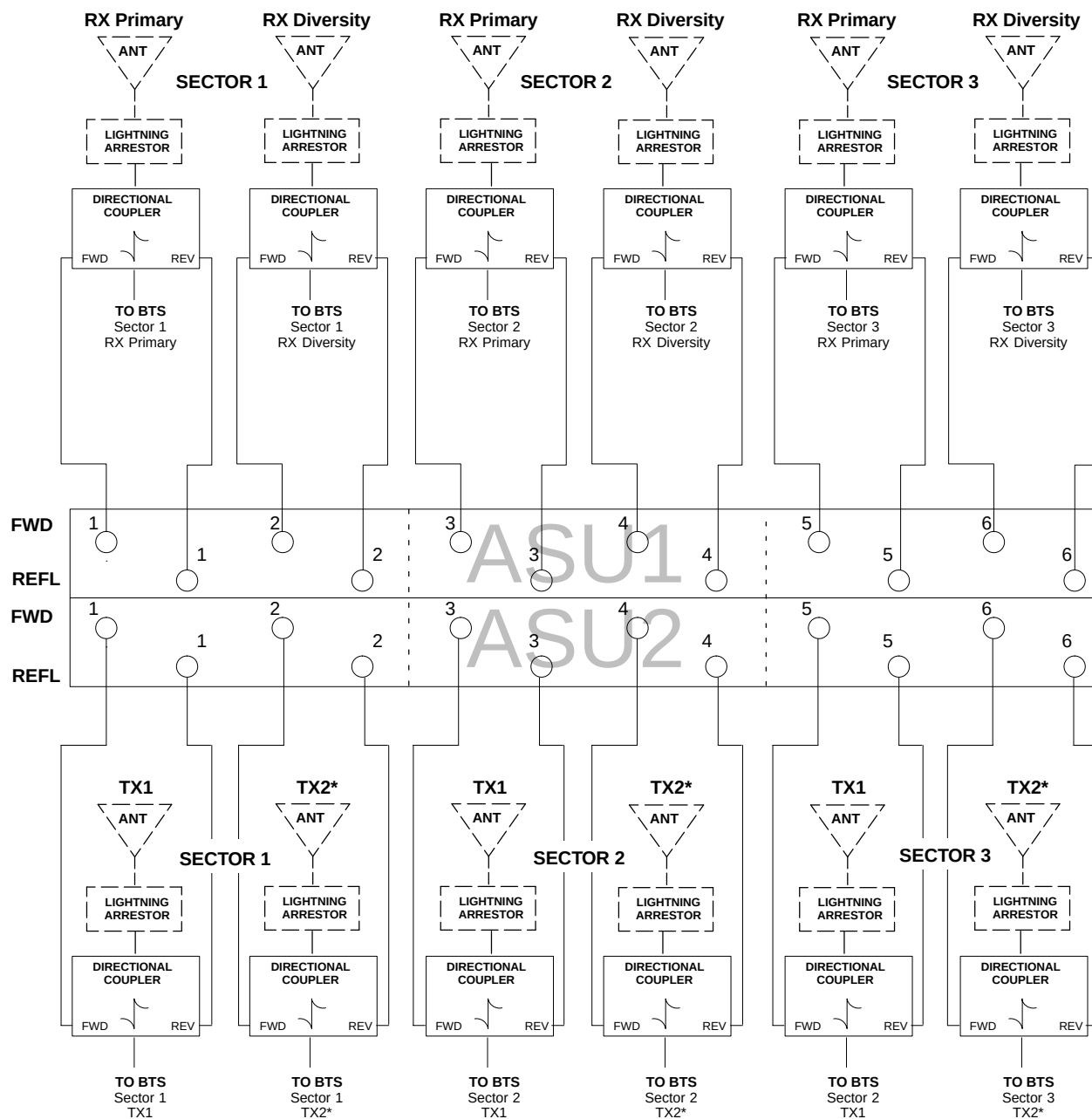
Figure 4-9: 3-Sector Non-Duplexed Cabling Configurations
