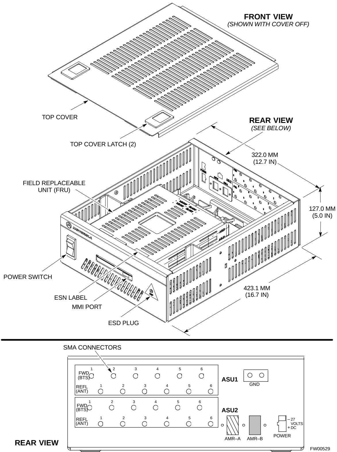
Figure 4-3: RFDS (Rack Mount Unit)
