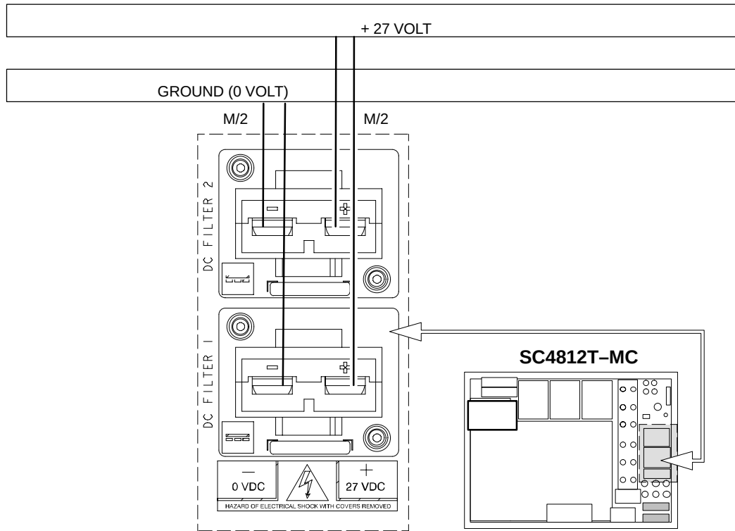
Figure 2-22: BTS Power Cabling for the + 27 V BTS Configuration using TwoPower Feeds
