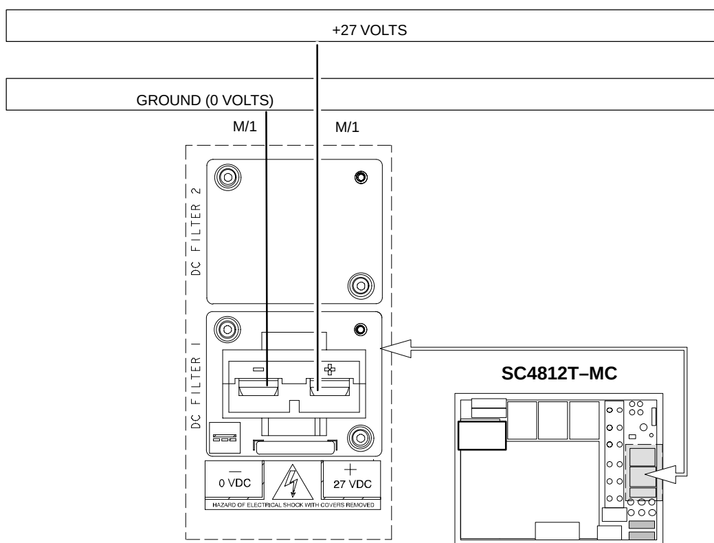
Figure 2-21: BTS Power Cabling for the +27 V BTS Configuration using One Power Feed
