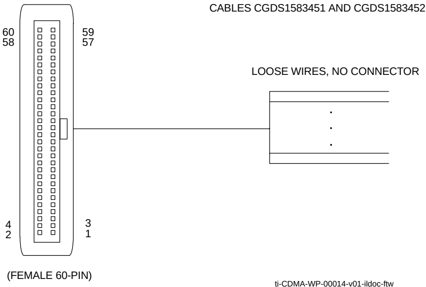
Figure 2-8: Cable B (Alarm) Pin Numbering
