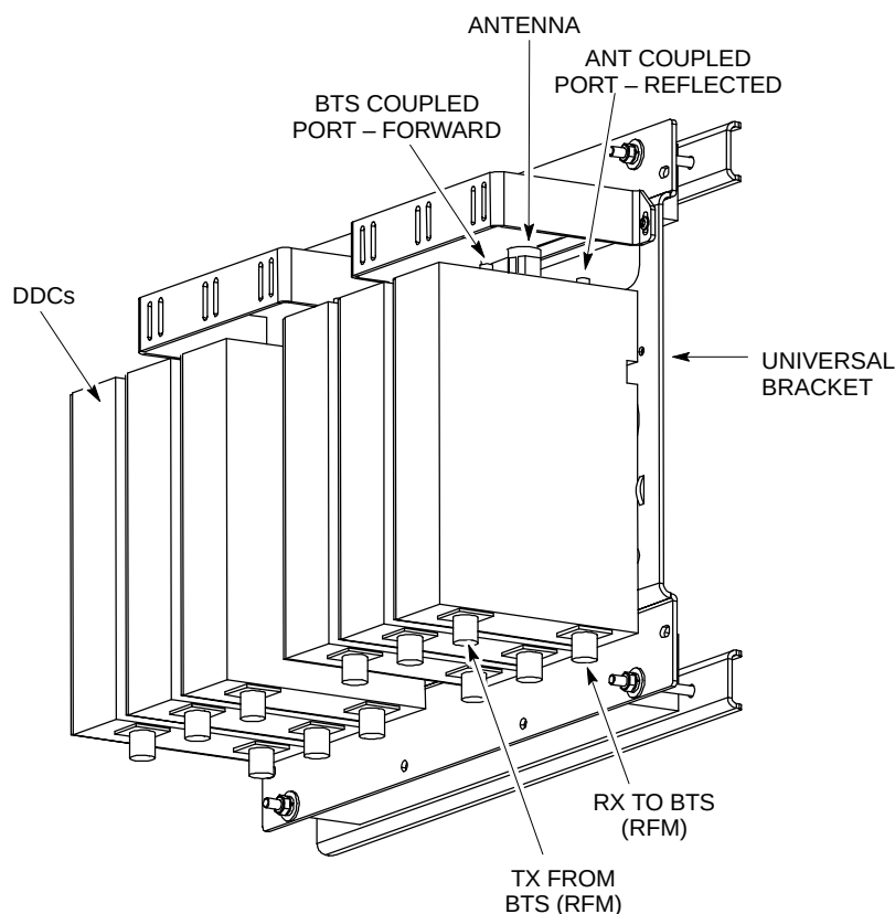
Figure 4-2: DDC (Duplexers – Directional Couplers)
