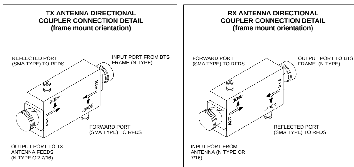
Figure 4-1: Directional Couplers
