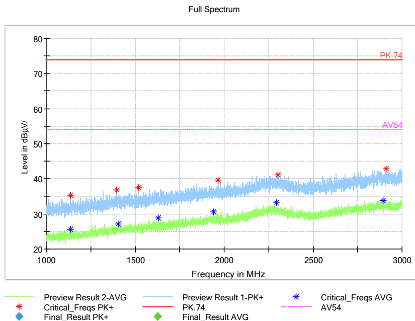
Pic8. Radiated emission (1GHz –3GHz)
