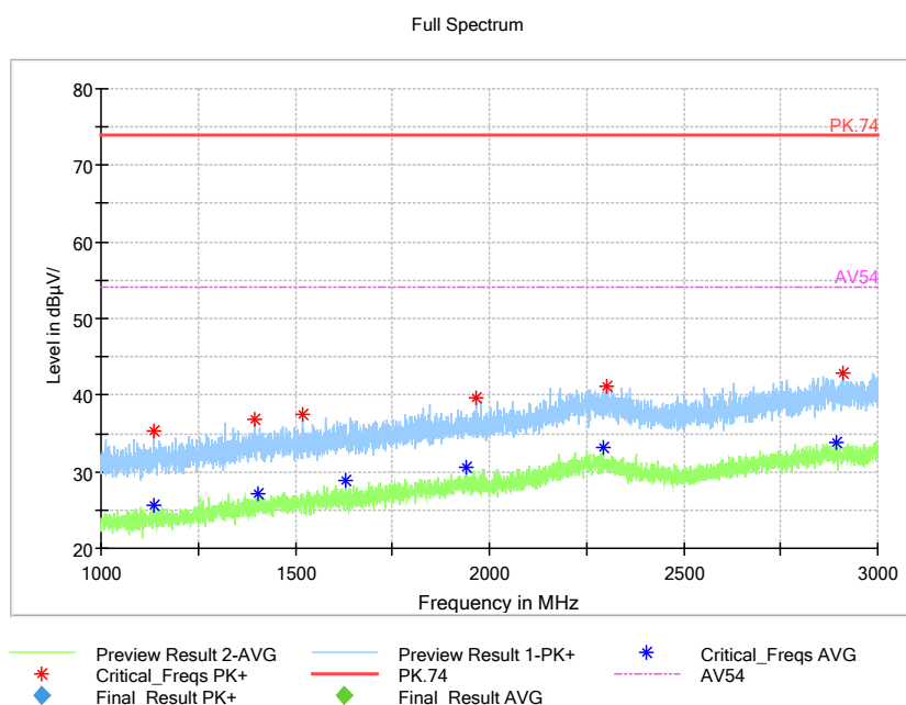
Pic13. Radiated emission (1GHz –3GHz)
