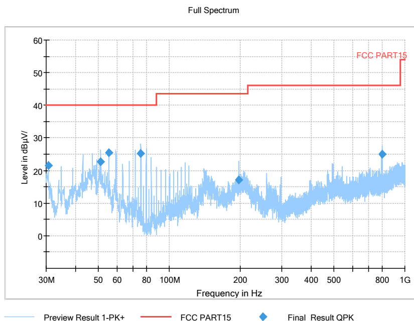
Pic12. Radiated emission(30MHz – 1GHz)
