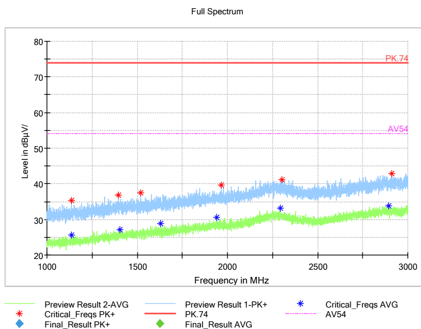
Pic18. Radiated emission (1GHz –3GHz)
