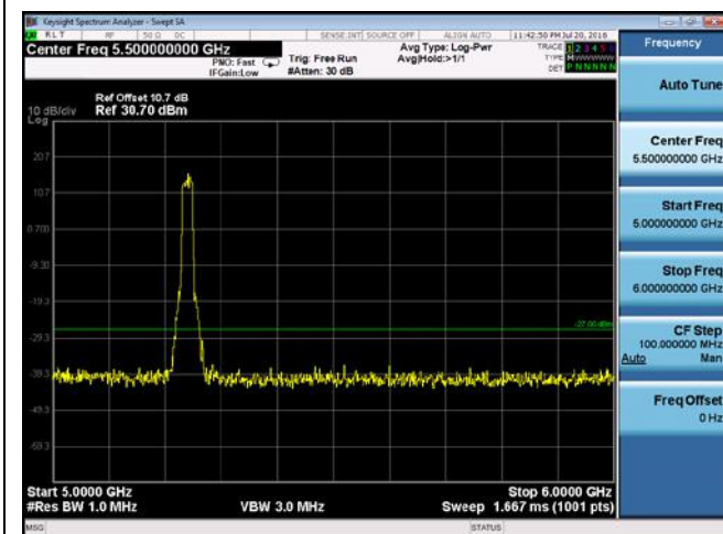
CUE-802.11n-20-5240M-chain 1(5GHz-6GHz)
