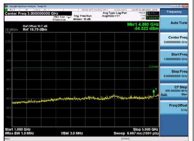
CUE-802.11a-5240M-chain 3(1GHz-5GHz)
