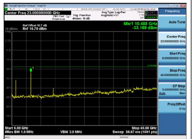
CUE-802.11n-20-5240M-chain 1(6GHz-40GHz)
