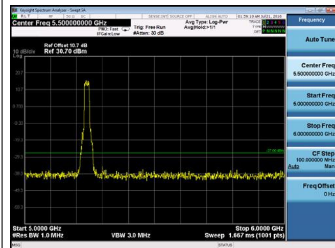
CUE-802.11n-20-5240M-chain 4(5GHz-6GHz)
