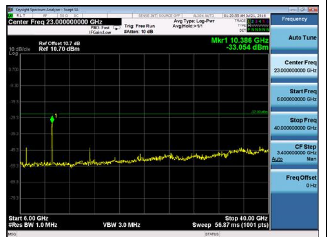
CUE-802.11n-40-5190M -chain3(6GHz-40GHz)
