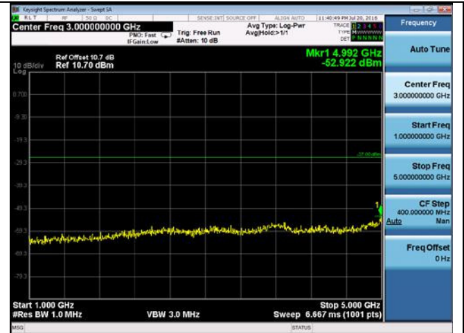
CUE-802.11n-20-5180M-chain1(1GHz-5GHz)
