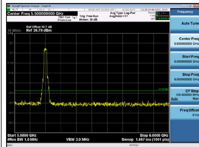
CUE-802.11n-20-5200M-chain2(5GHz-6GHz)
