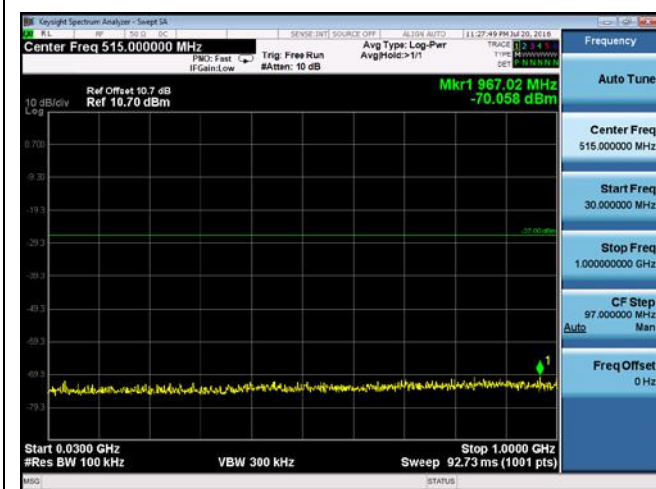
CUE-802.11a-5200M-chain1(30MHz-1GHz)
