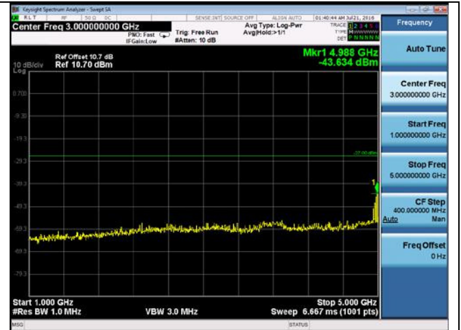
CUE-802.11a-5180M-chain4(1GHz-5GHz)
