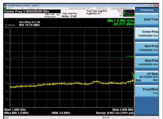
CUE-802.11n-20-5200M-chain1(1GHz-5GHz)
