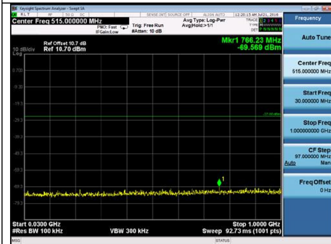
CUE-802.11n-20-5200M-chain2(30MHz-1GHz)
