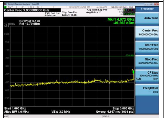
CUE-802.11n-20-5200M-chain2(1GHz-5GHz)
