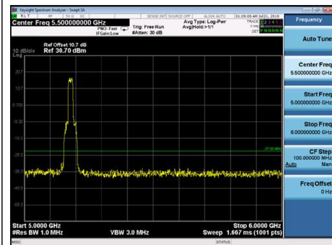
CUE-802.11n-20-5180M-chain3(5GHz-6GHz)
