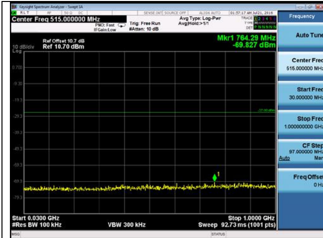
CUE-802.11n-20-5180M-chain4(30MHz-1GHz)
