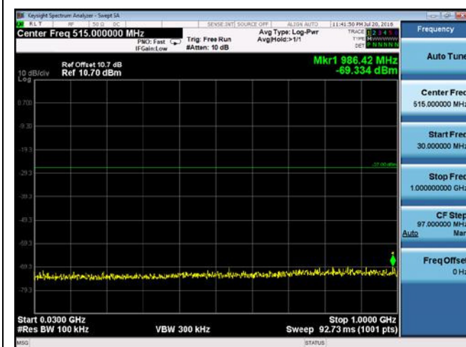
CUE-802.11n-20-5200M-chain1(30MHz-1GHz)
