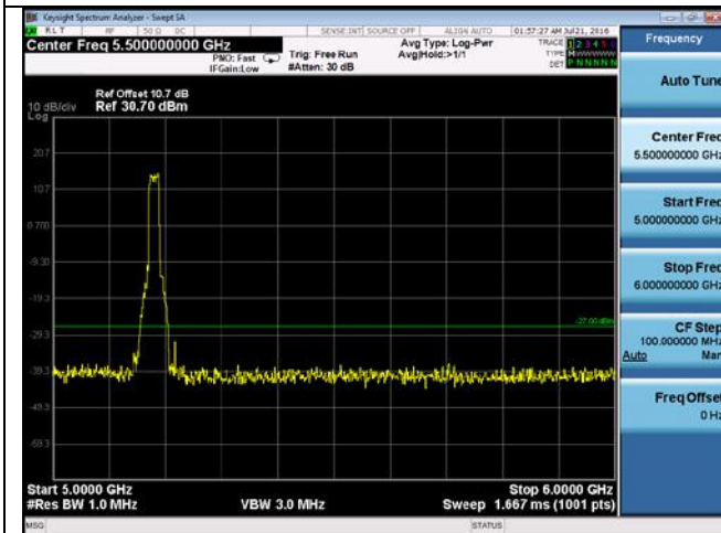
CUE-802.11n-20-5180M-chain4(5GHz-6GHz)
