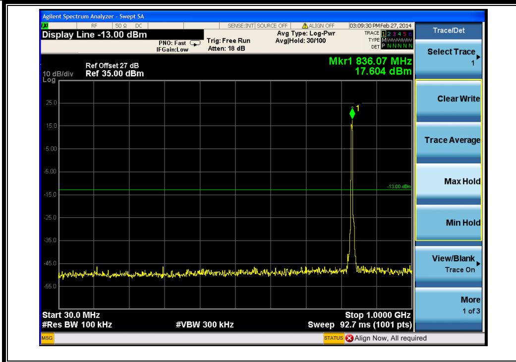
(Plot G 2: HSUPA850MHz Channel = 4175, 30MHz to 1GHz)
