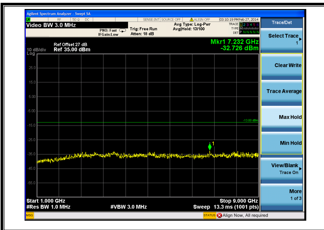
(Plot G2.1: HSUPA850MHz Channel = 4175, 1GHz to 9GHz)
