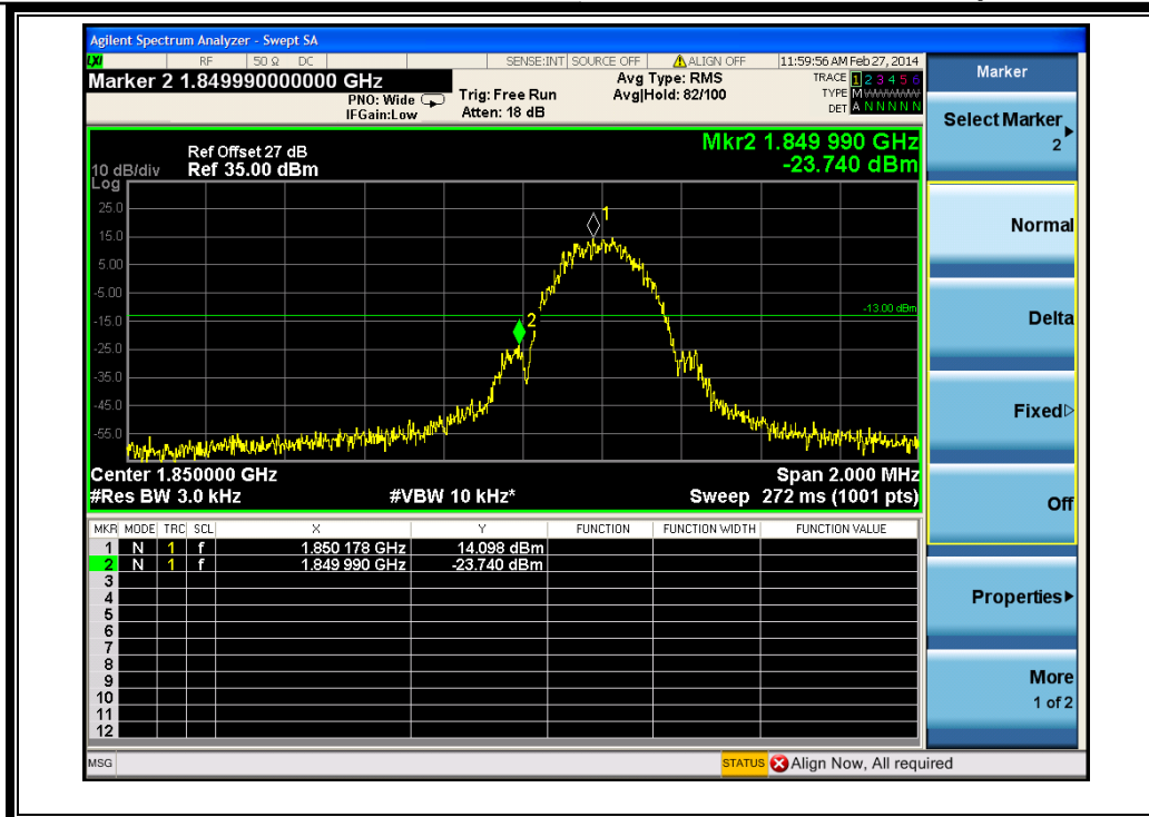
(Plot G: EGPRS 1900 Channel = 512)
