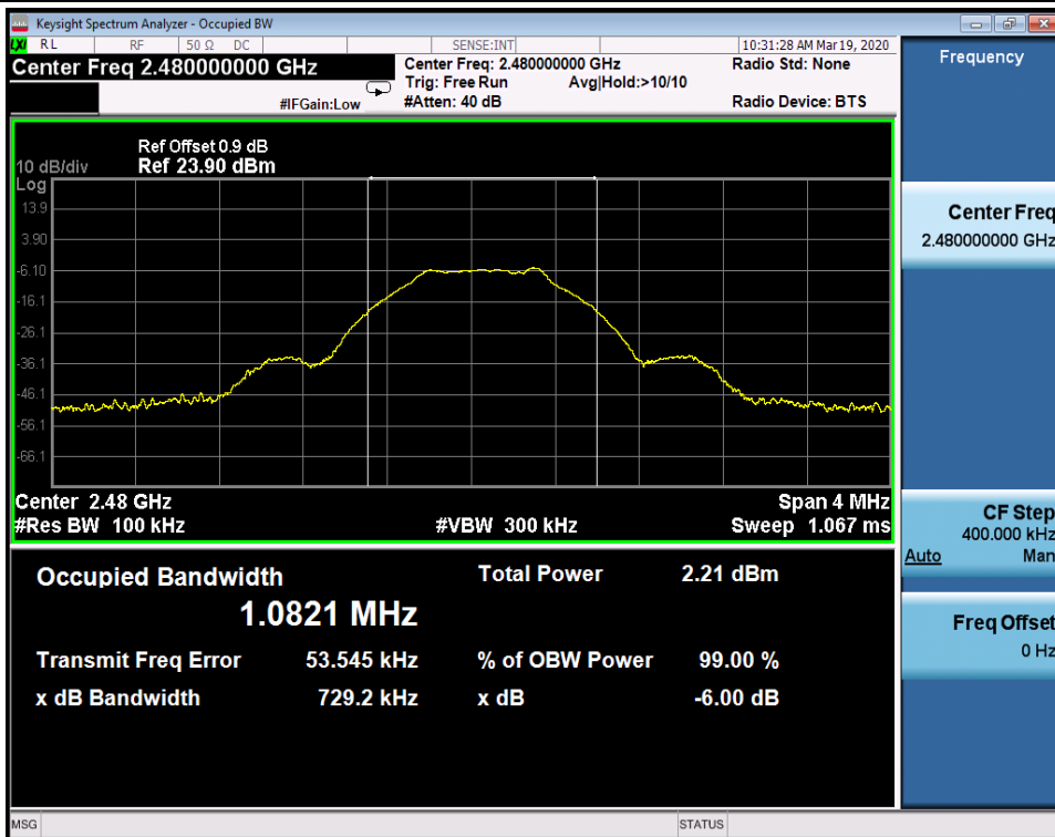
6dB Bandwidth_BLE_2480_Ant1
