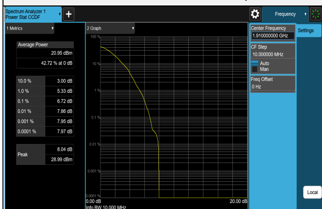
64QAM CH 26640 (1910MHz)
