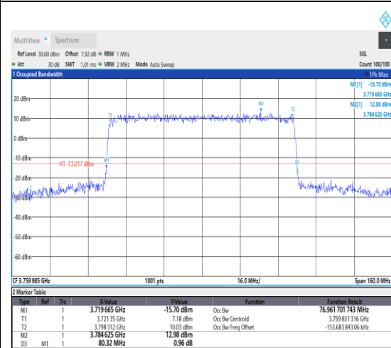
1-N78-3700-3800--30-80-H-3-DFT-16QAM-O
