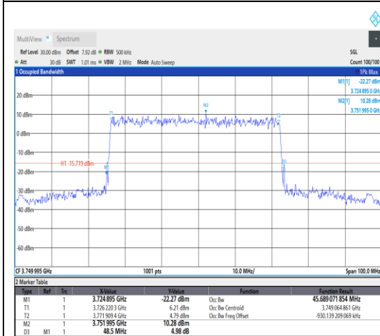
1-N78-3700-3800--30-50-M-5-DFT-256QAM-
