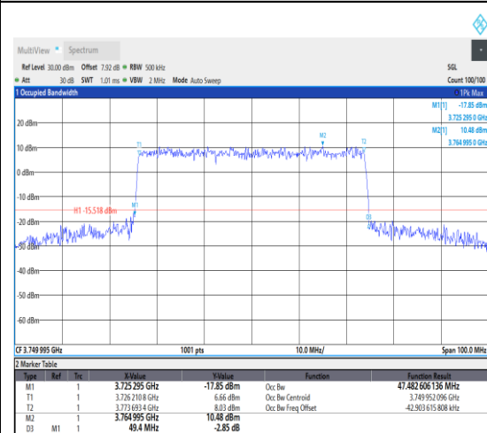
1-N78-3700-3800--30-50-M-6-CP-QPSK-Out
