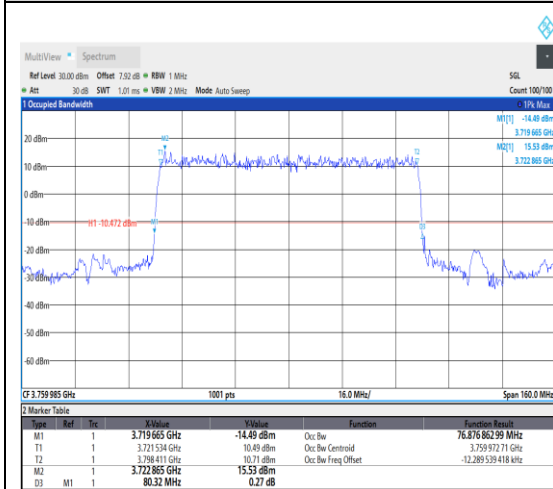
1-N78-3700-3800--30-80-H-2-DFT-PI2BPSK-
