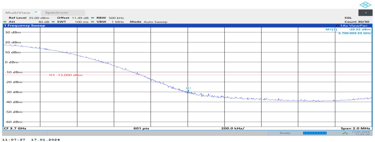
Band48-20MHz-16QAM-56640-100RB#0
