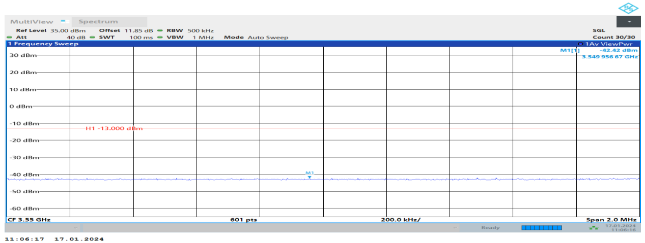
Band48-20MHz-16QAM-55340-100RB#0
