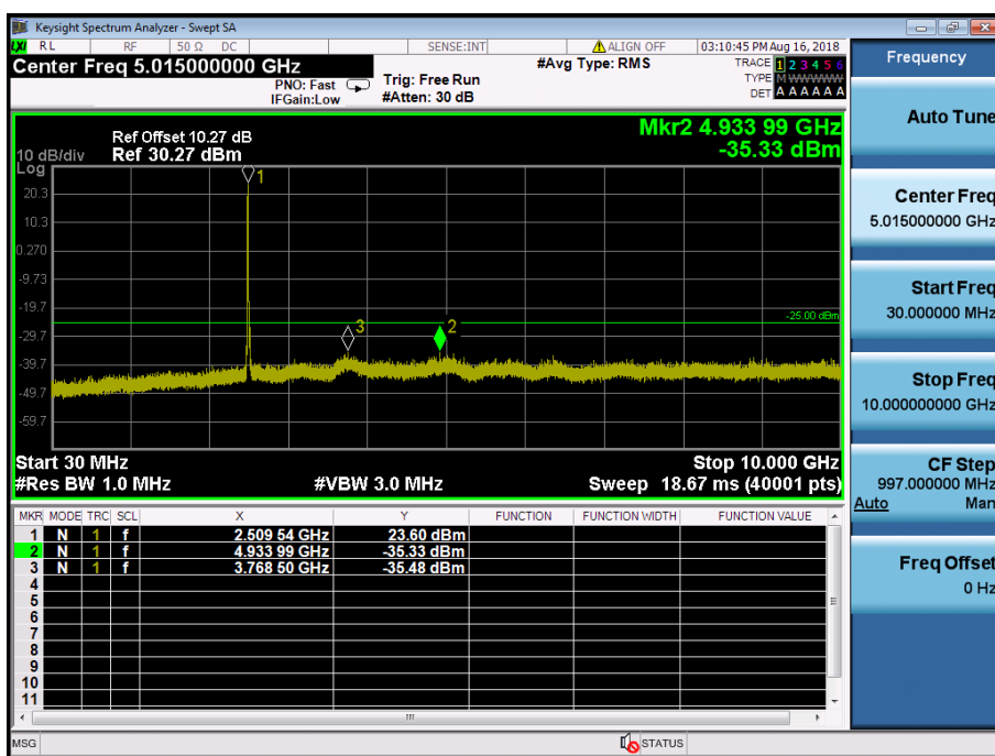
LTE Band 7 / 15MHz / QPSK - RB Size/Offset (36/18) – Low Channel
