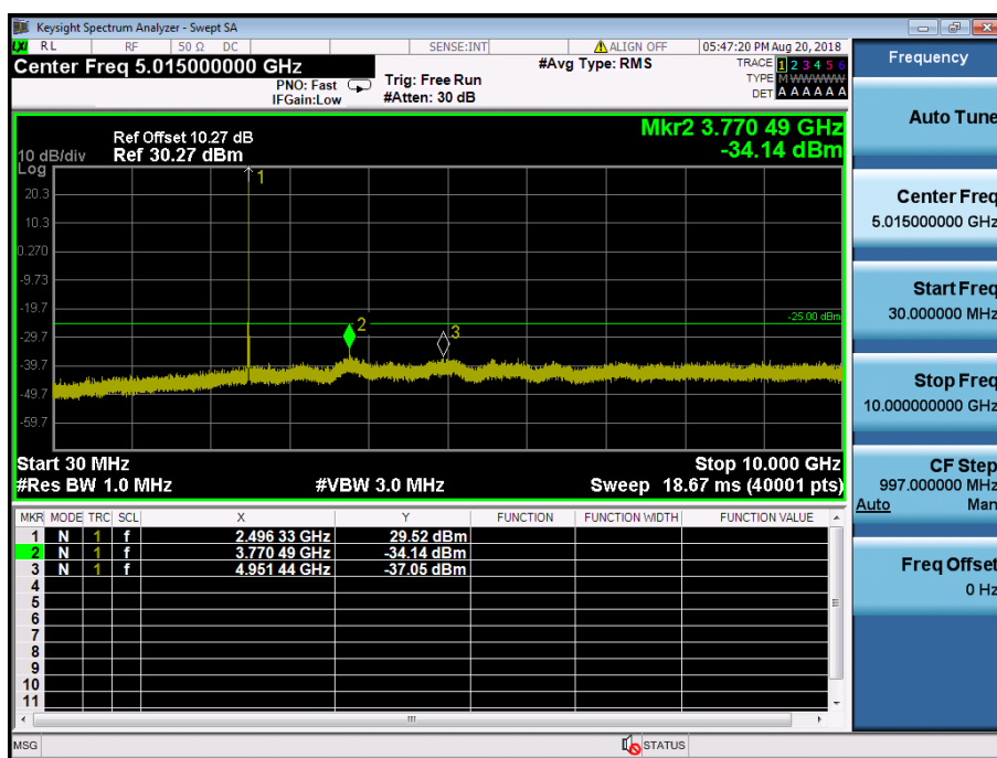
LTE Band 41 / 5MHz / QPSK - RB Size/Offset (1/0) – Low Channel
