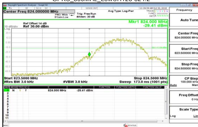
GPRS_850MHz_LowCH128-824.2
