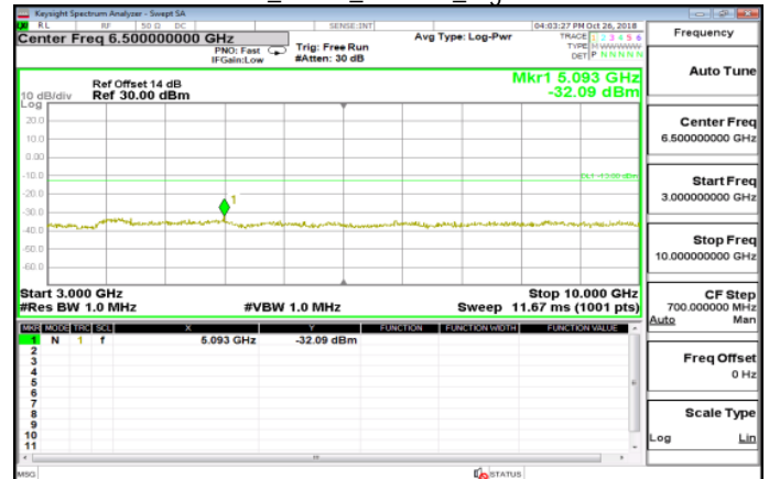
3GHz-10GHz_GPRS_850MHz_HighCH251-848.8
