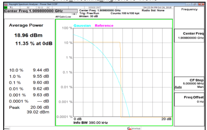
GRPS_1900MHz_HighCH810-1909.8
