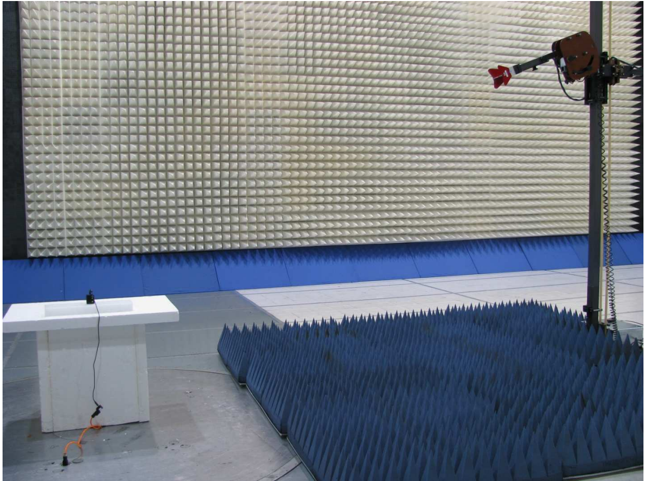
Radiated Emissions (Horn)
