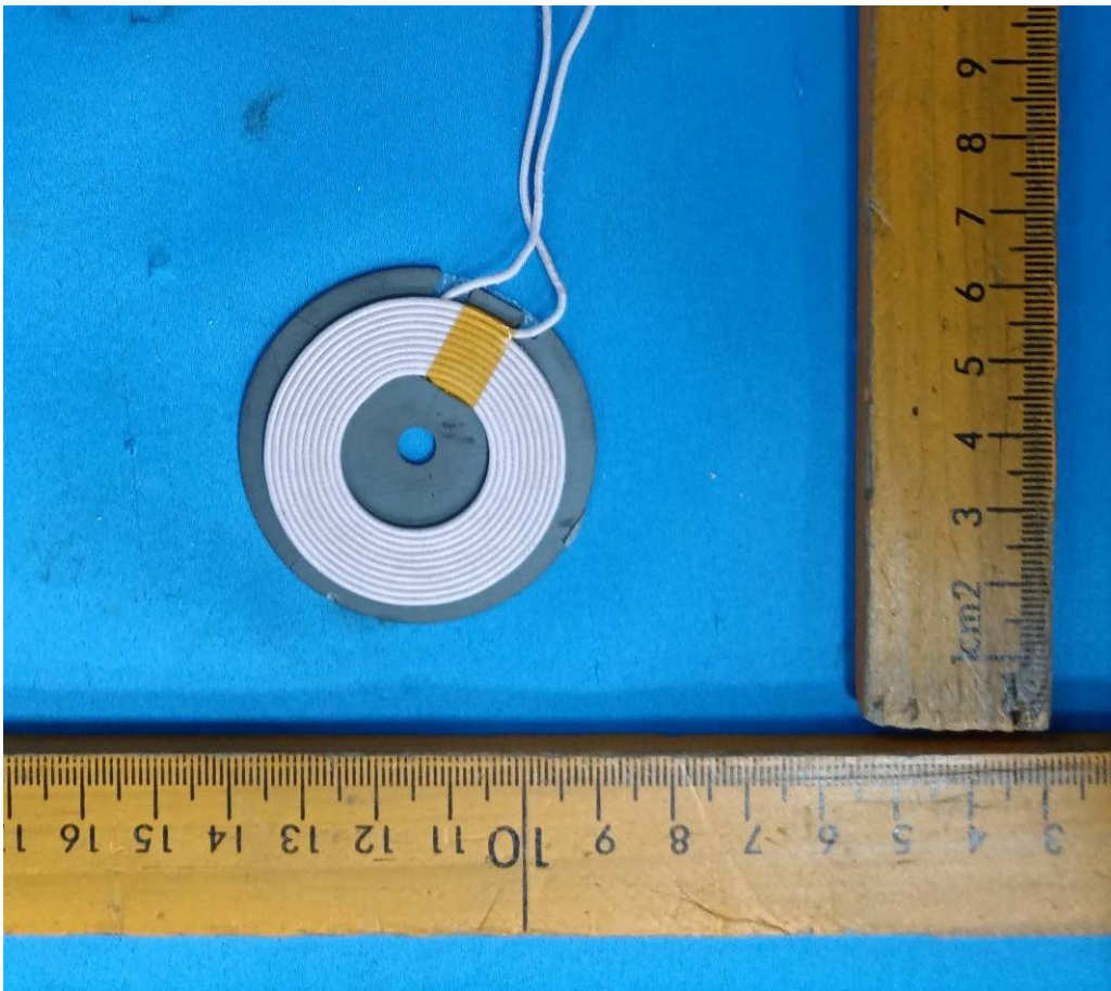
Coil
