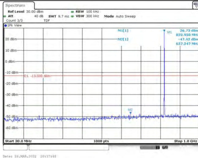
Band26-1.4MHz-16QAM-26797-1RB#0-Range1:30~1000MHz
