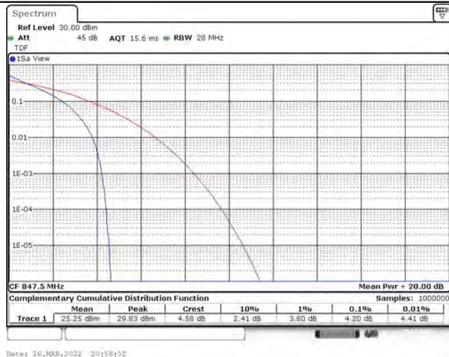
Band26-3MHz-QPSK-27025-15RB#0
