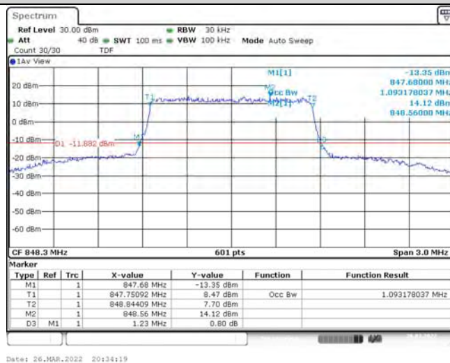
Band26-1.4MHz-QPSK-27033-6RB#0-1.093
