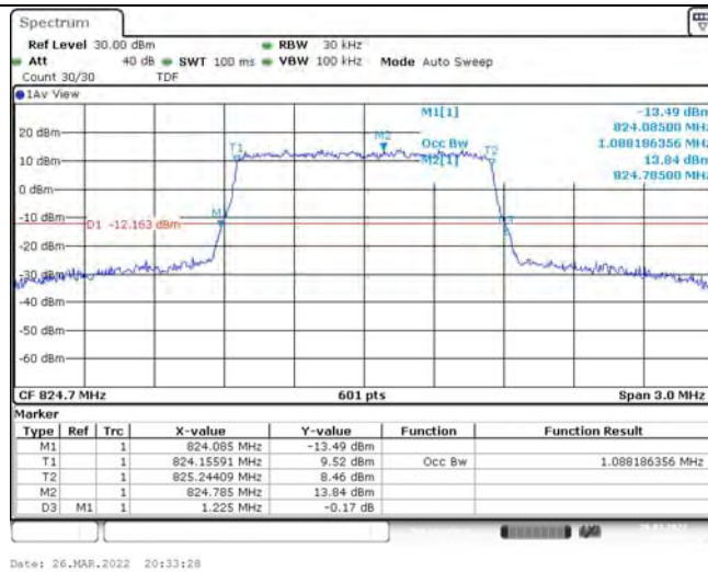
Band26-1.4MHz-QPSK-26797-6RB#0-1.088
