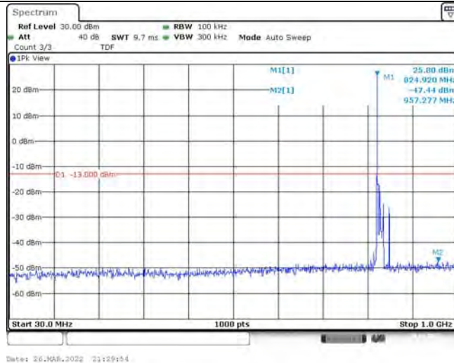
Band26-15MHz-QPSK-26865-1RB#0-Range1:30~1000MHz
