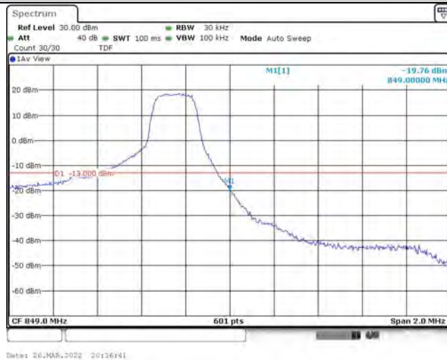
Band26-1.4MHz-QPSK-27033-1RB#5
