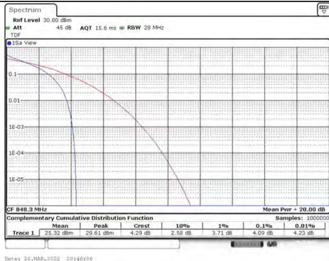
Band26-1.4MHz-QPSK-27033-6RB#0
