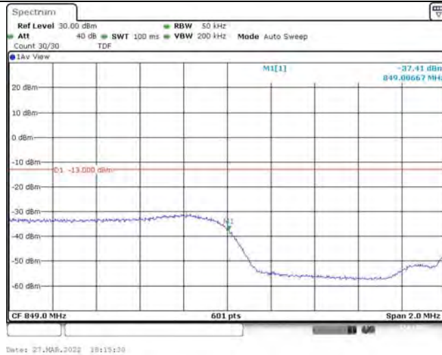
Band26-3MHz-16QAM-27025-1RB#0
