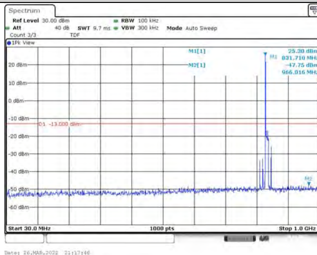
Band26-10MHz-16QAM-26915-1RB#0-Range1:30~1000MHz
