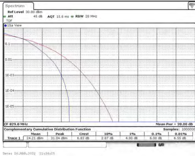
Band26-10MHz-16QAM-26840-50RB#0
