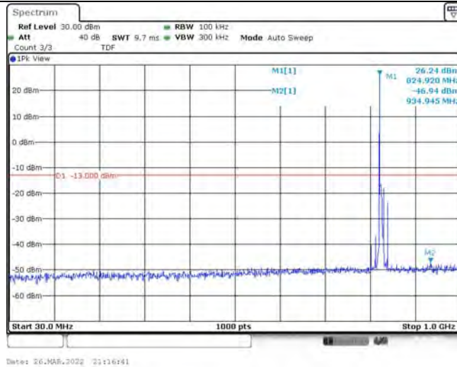
Band26-10MHz-QPSK-26840-1RB#0-Range1:30~1000MHz
