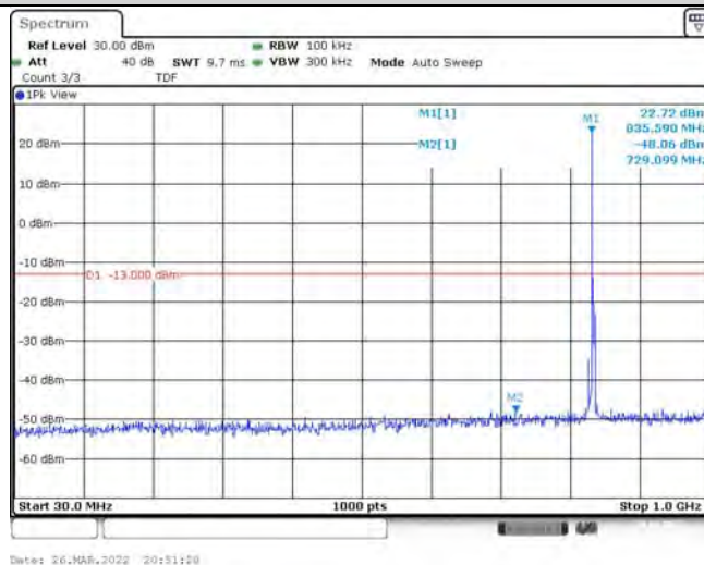
Band26-3MHz-16QAM-26915-1RB#0-Range1:30~1000MHz
