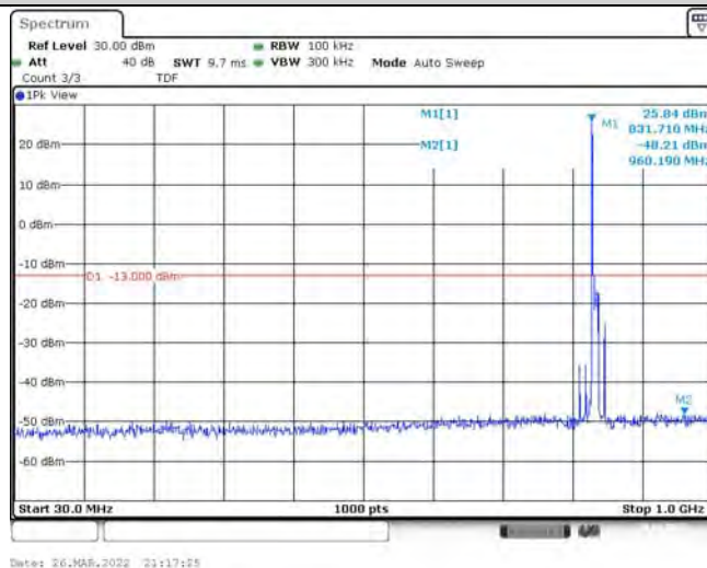
Band26-10MHz-QPSK-26915-1RB#0-Range1:30~1000MHz
