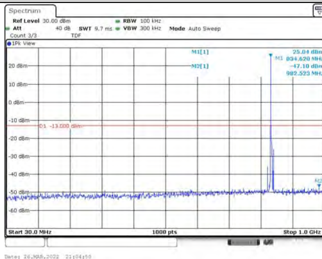
Band26-5MHz-16QAM-26915-1RB#0-Range1:30~1000MHz
