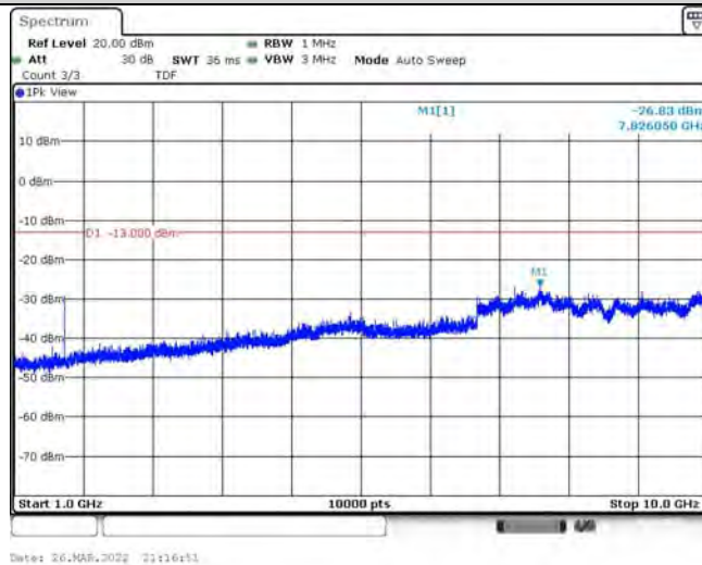
Band26-10MHz-QPSK-26840-1RB#0-Range2:1000~10000MHz
