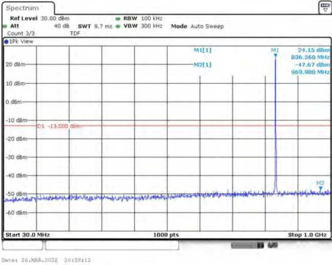
Band26-1.4MHz-QPSK-26915-1RB#0-Range1:30~1000MHz
