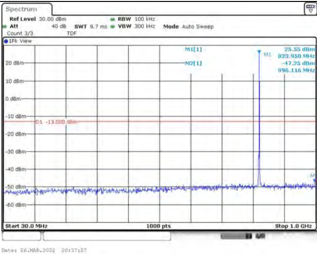
Band26-1.4MHz-QPSK-26797-1RB#0-Range1:30~1000MHz
