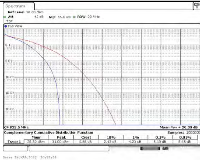
Band26-3MHz-QPSK-26805-15RB#0
