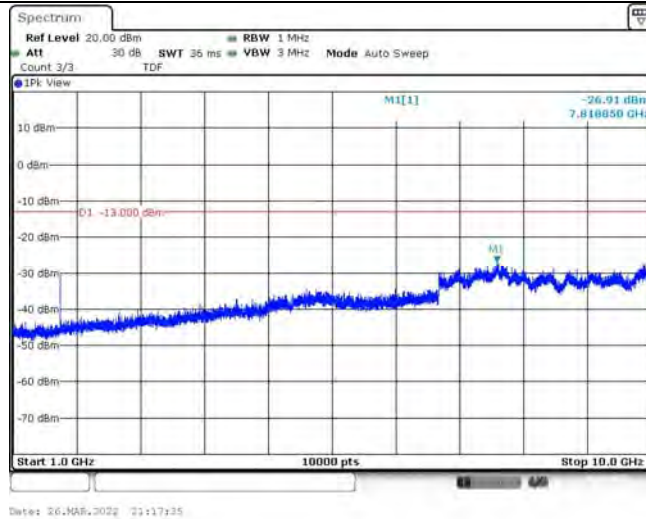
Band26-10MHz-QPSK-26915-1RB#0-Range2:1000~10000MHz
