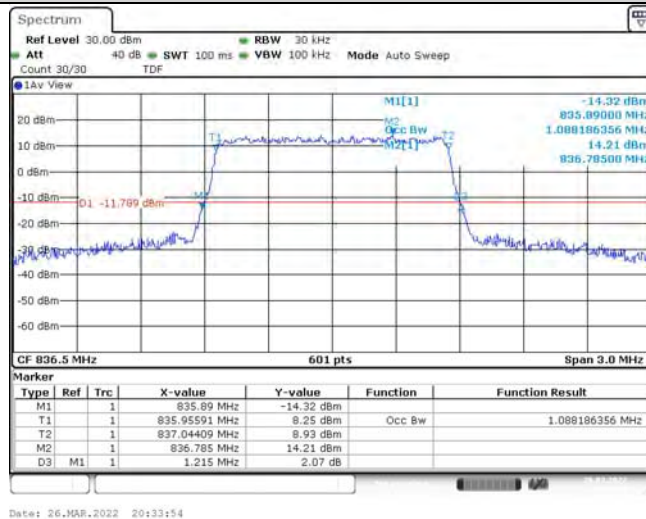
Band26-1.4MHz-QPSK-26915-6RB#0-1.088
