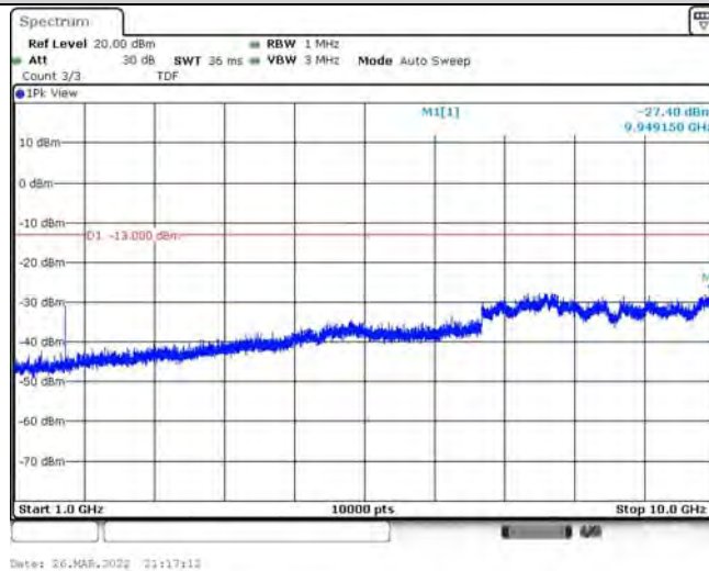
Band26-10MHz-16QAM-26840-1RB#0-Range2:1000~10000MHz
