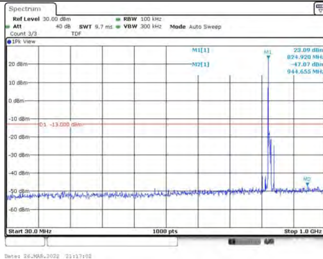
Band26-10MHz-16QAM-26840-1RB#0-Range1:30~1000MHz
