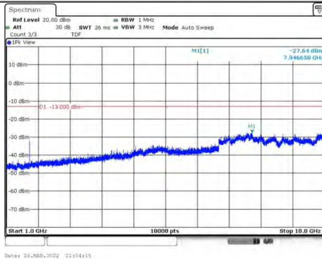
Band26-5MHz-16QAM-26815-1RB#0-Range2:1000~10000MHz
