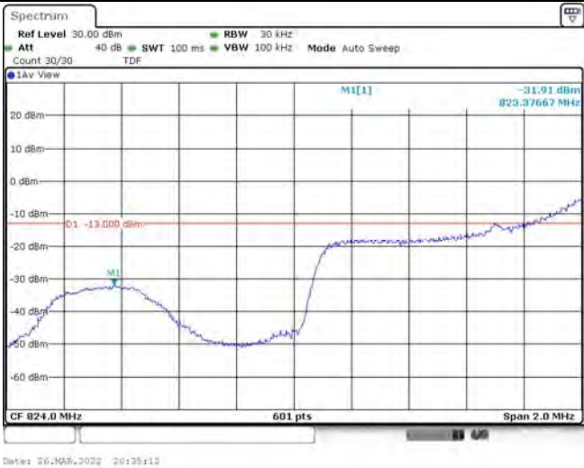
Band26-1.4MHz-QPSK-26797-1RB#5
