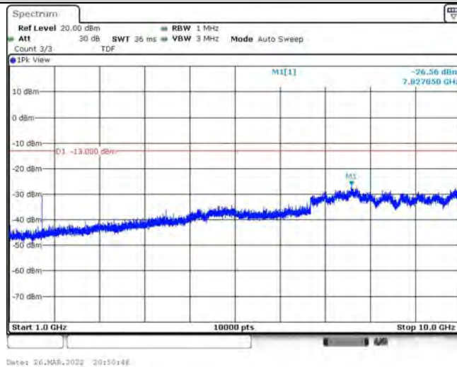
Band26-3MHz-16QAM-26805-1RB#0-Range2:1000~10000MHz
