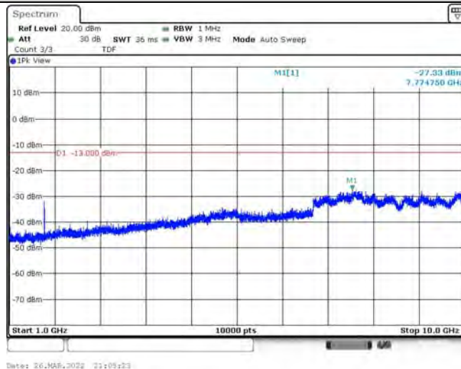
Band26-5MHz-QPSK-27015-1RB#0-Range2:1000~10000MHz
