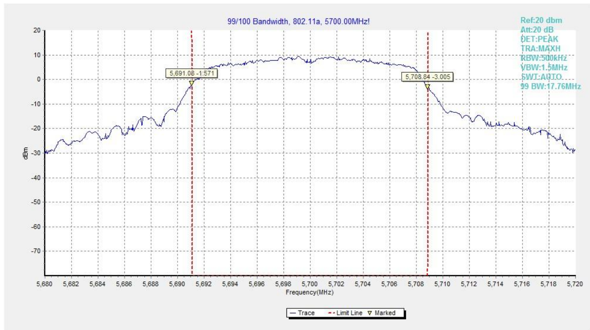
Fig. 26 99% Occupied Bandwidth (802.11a, 5700MHz)
