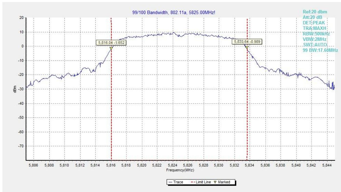
Fig. 28 99% Occupied Bandwidth (802.11a, 5825MHz)
