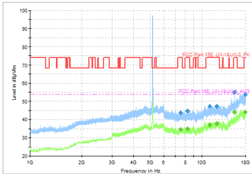
Fig. 57 Transmitter Spurious Emission (802.11a, CH36 5180MHz)
