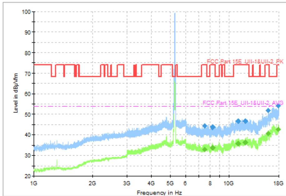
Fig. 67 Transmitter Spurious Emission (802.11n-HT40, CH54 5270MHz)
