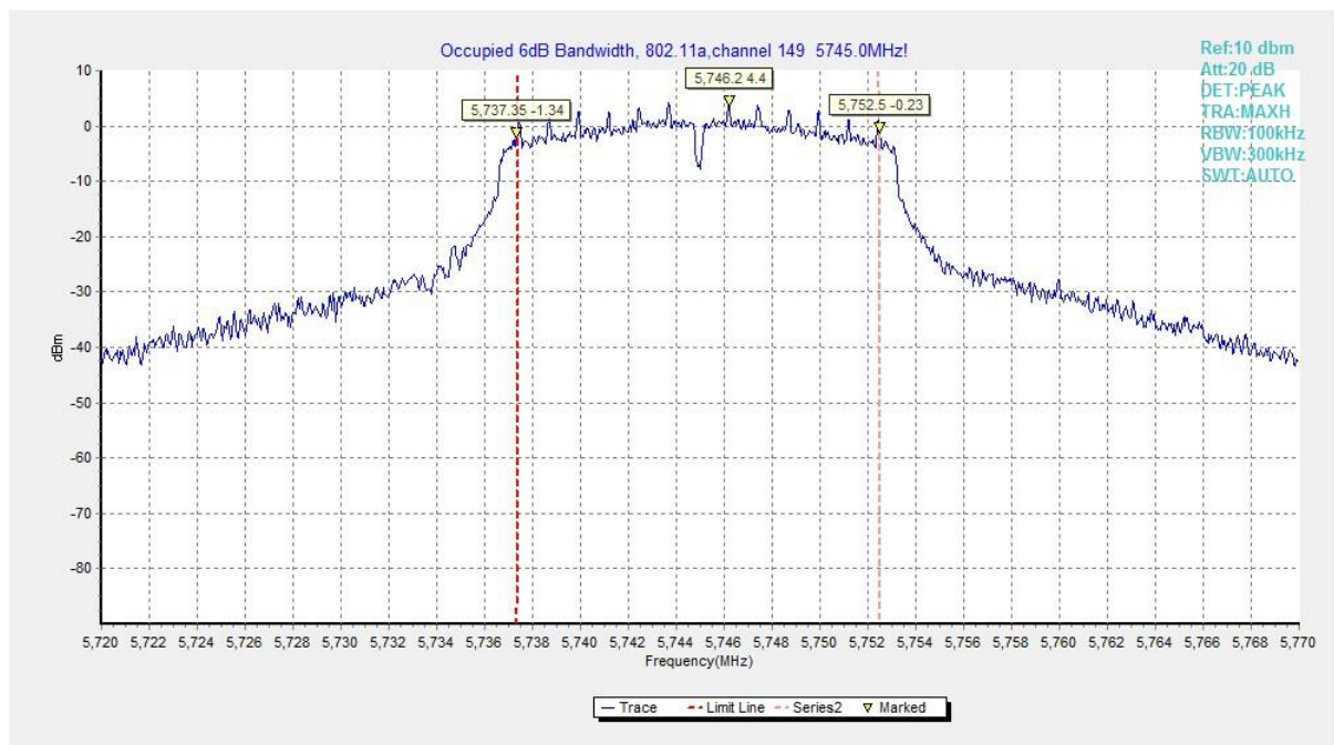
Fig. 16 Occupied 6dB Bandwidth (802.11a, 5745MHz)
