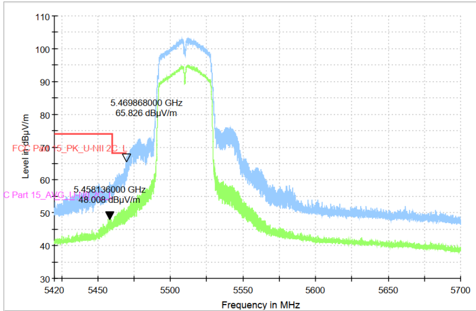
Fig. 49 Band Edges (802.11n-HT40, CH102 5510MHz)
