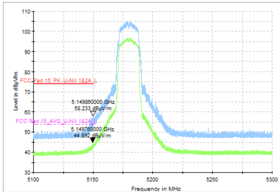
Fig. 41 Band Edges (802.11a, CH36 5180MHz)
