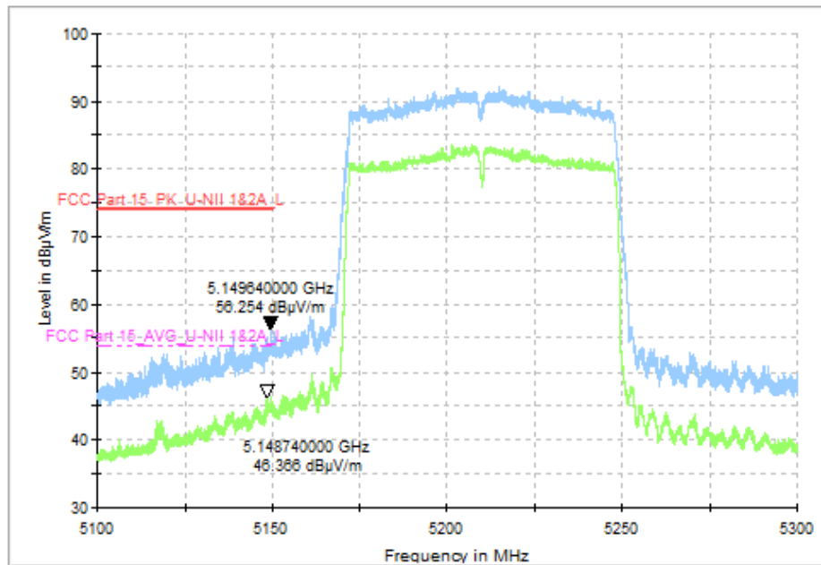
Fig. 53 Band Edges (802.11ac-VHT80, CH42 5210MHz)
