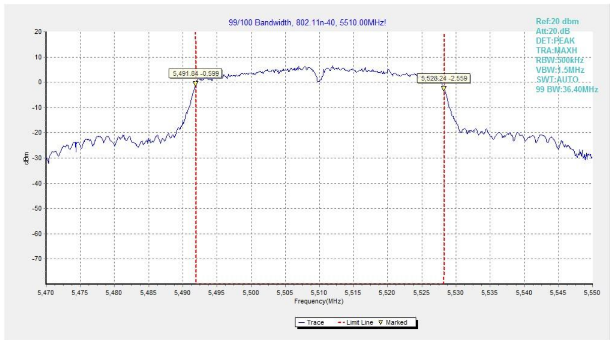
Fig. 33 99% Occupied Bandwidth (802.11n-HT40, 5510MHz)
