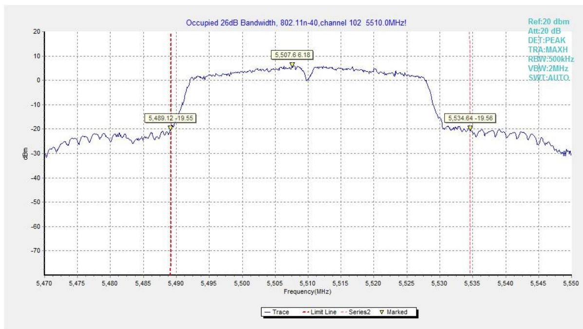
Fig. 11 Occupied 26dB Bandwidth (802.11n-HT40, 5510MHz)
