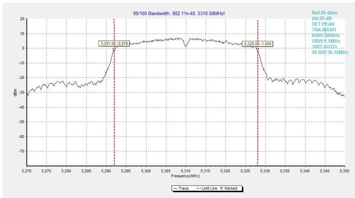
Fig. 32 99% Occupied Bandwidth (802.11n-HT40, 5310MHz)
