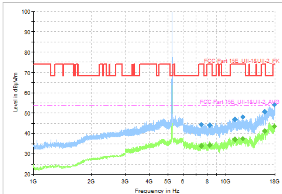
Fig. 59 Transmitter Spurious Emission (802.11a, CH52 5260MHz)
