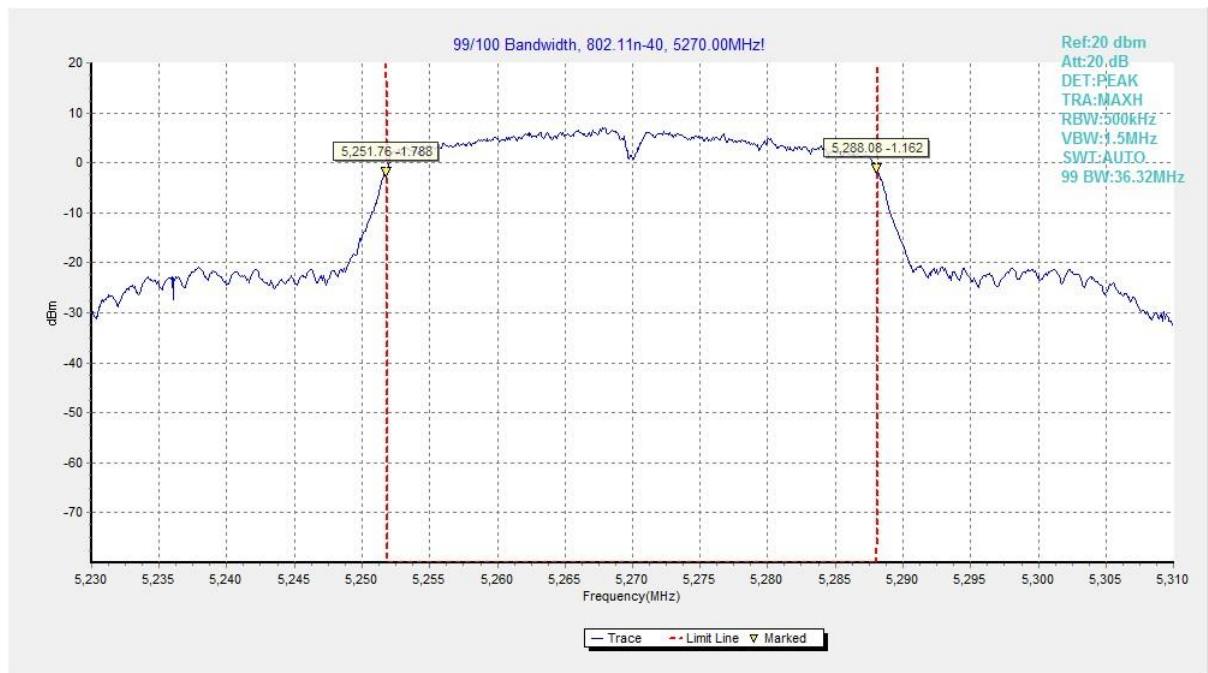
Fig. 31 99% Occupied Bandwidth (802.11n-HT40, 5270MHz)
