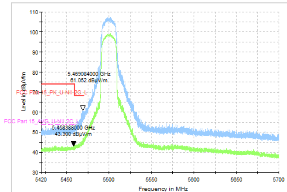
Fig. 43 Band Edges (802.11a, CH100 5500MHz)
