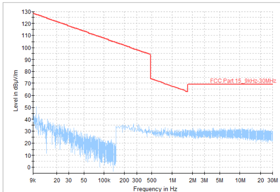
Fig. 80 Radiated Spurious Emission (All Channel, 9kHz ~ 30MHz)
