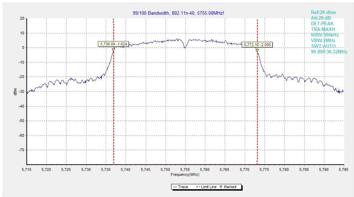
Fig. 35 99% Occupied Bandwidth (802.11n-HT40, 5755MHz)
