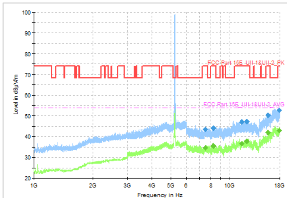
Fig. 58 Transmitter Spurious Emission (802.11a, CH48 5240MHz)
