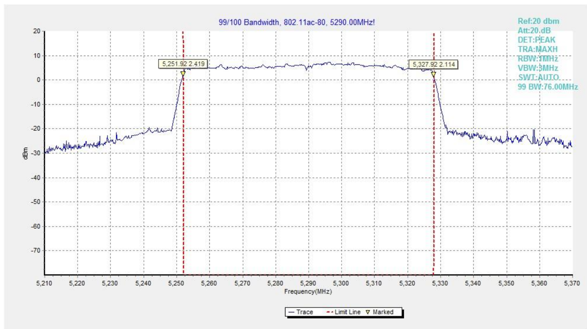
Fig. 38 99% Occupied Bandwidth (802. 11ac-VHT80, 5290MHz)
