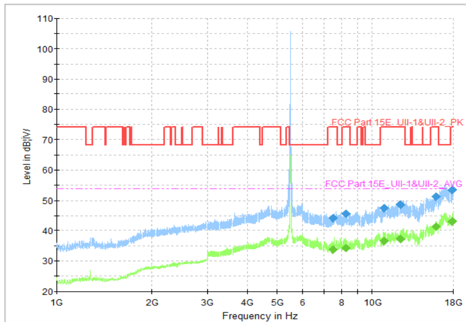
Fig. 61 Transmitter Spurious Emission (802.11a, CH100 5500MHz)
