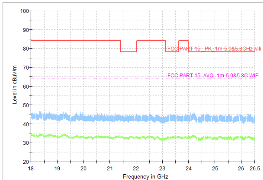
Fig. 78 Transmitter Spurious Emission (All channel, 18GHz~26.5GHz)
