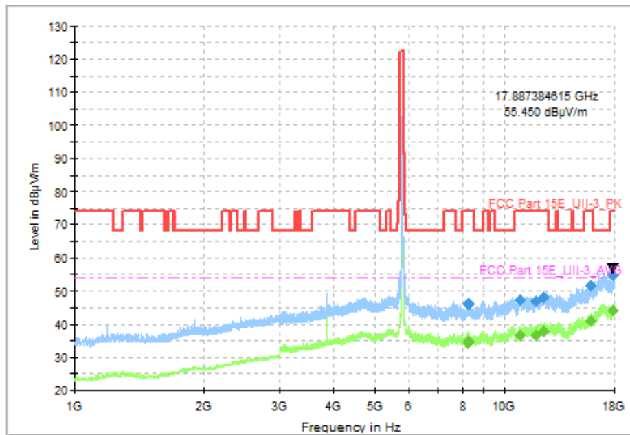
Fig. 72 Transmitter Spurious Emission (802. 11n-HT40, CH159 5795MHz)
