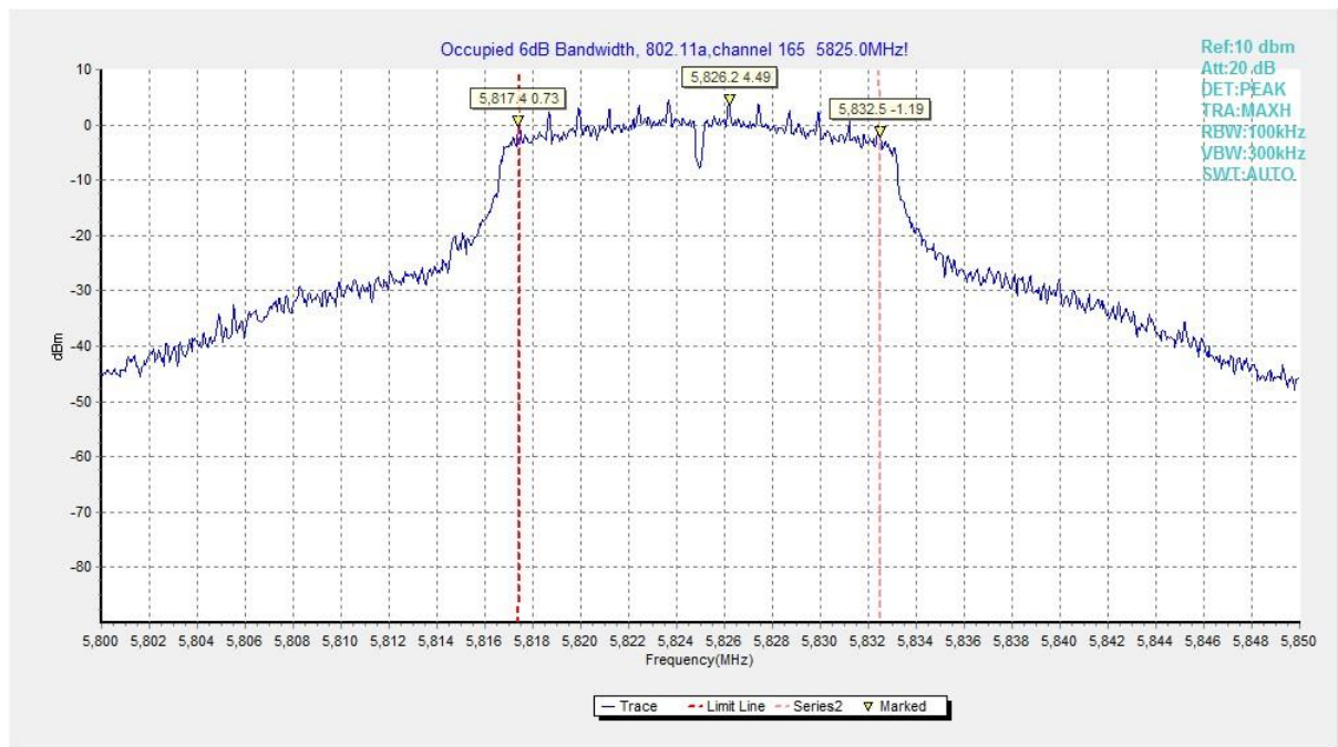
Fig. 17 Occupied 6dB Bandwidth (802.11a, 5825MHz)
