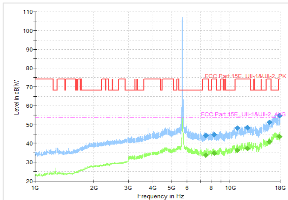
Fig. 62 Transmitter Spurious Emission (802.11a, CH140 5700MHz)
