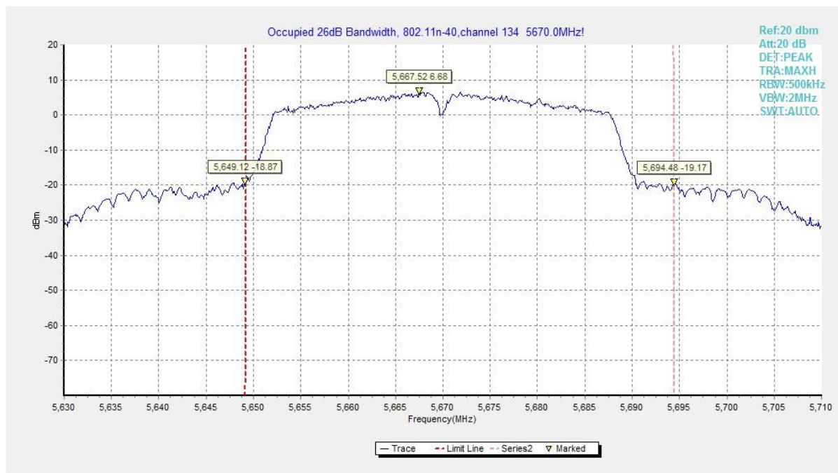
Fig. 12 Occupied 26dB Bandwidth (802.11n-HT40, 5670MHz)
