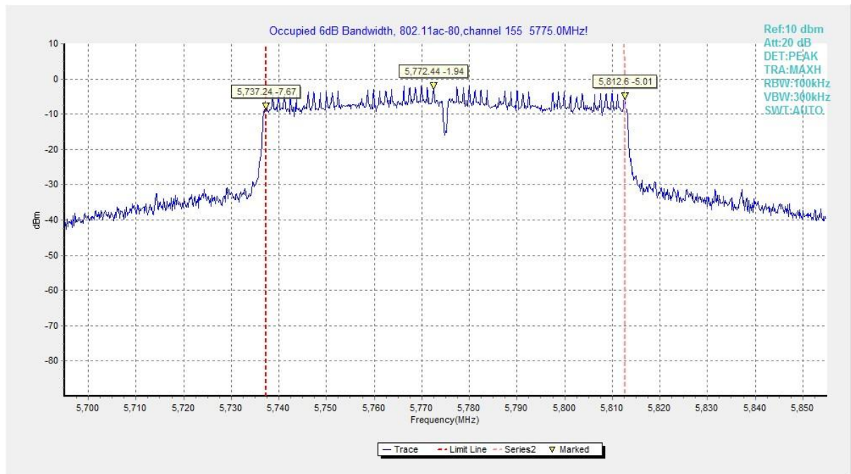
Fig. 20 Occupied 6dB Bandwidth (802.11ac-VHT80, 5775MHz)
