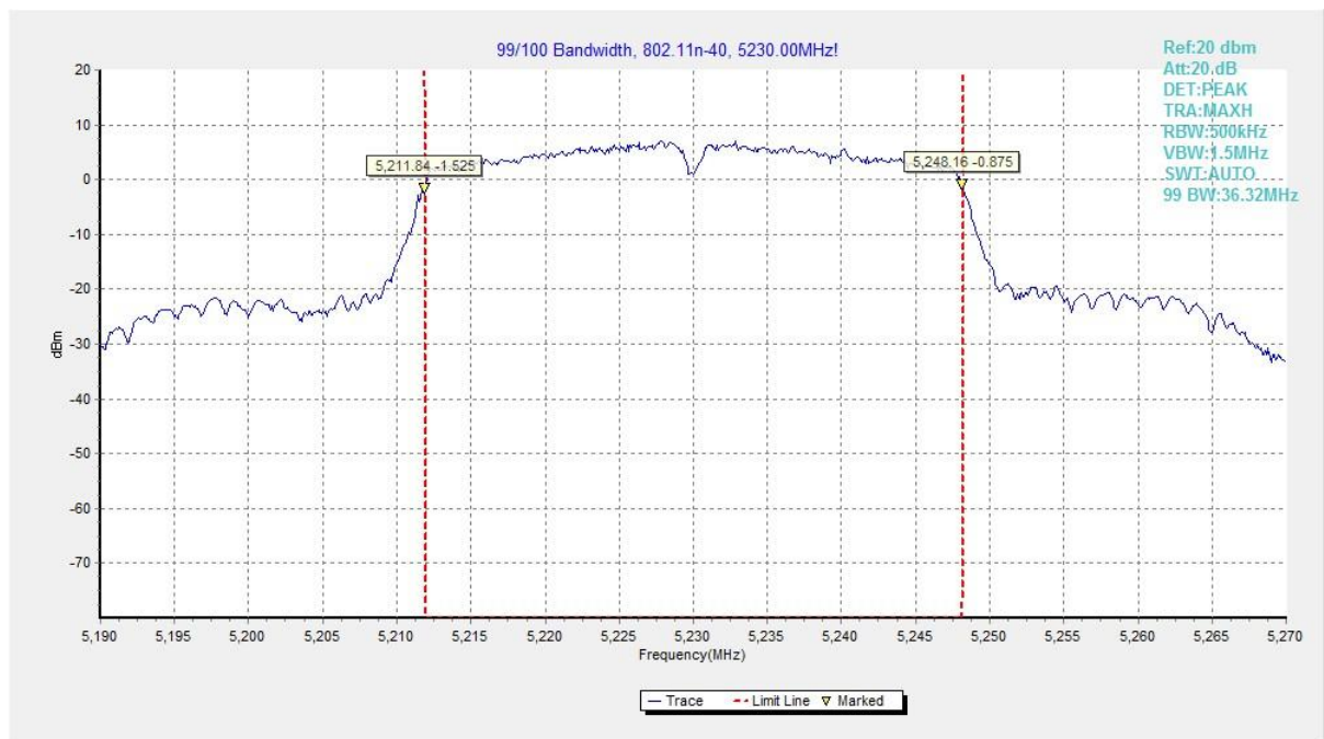
Fig. 30 99% Occupied Bandwidth (802.11n-HT40, 5230MHz)
