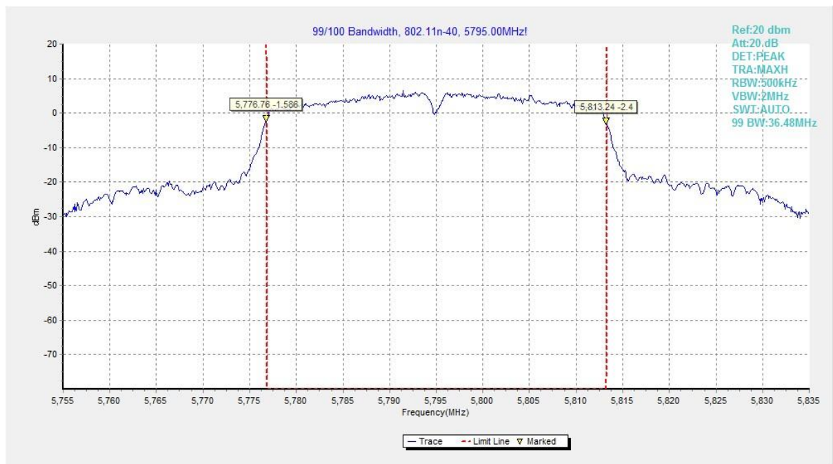
Fig. 36 99% Occupied Bandwidth (802.11n-HT40, 5795MHz)
