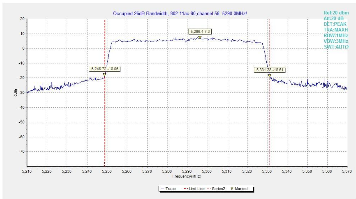
Fig. 14 Occupied 26dB Bandwidth (802. 11ac-VHT80, 5290MHz)
