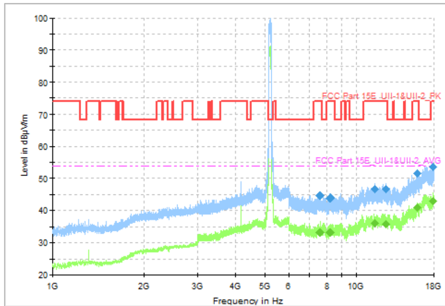
Fig. 73 Transmitter Spurious Emission (802. 11ac-VHT80, CH42 5210MHz)
