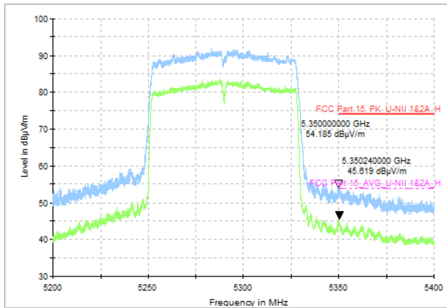
Fig. 54 Band Edges (802.11ac-VHT80, CH58 5290MHz)
