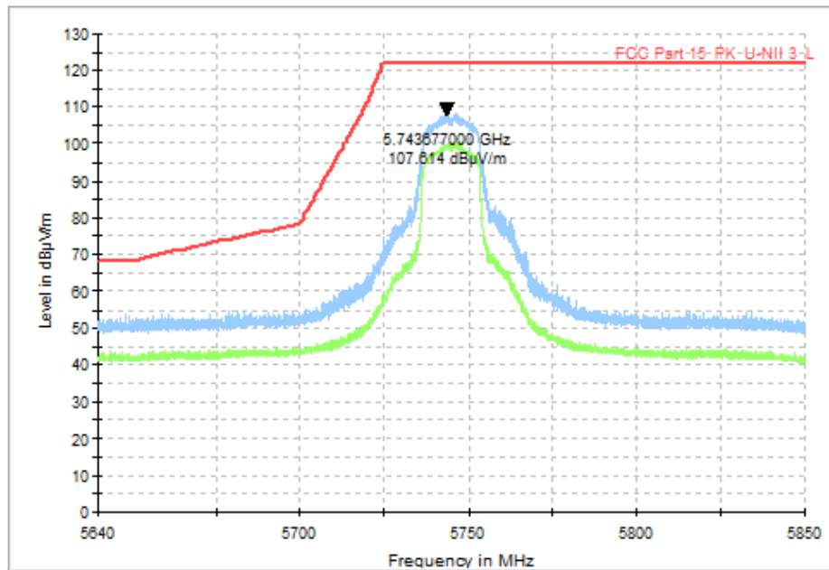
Fig. 45 Band Edges (802.11a, CH149 5745MHz)
