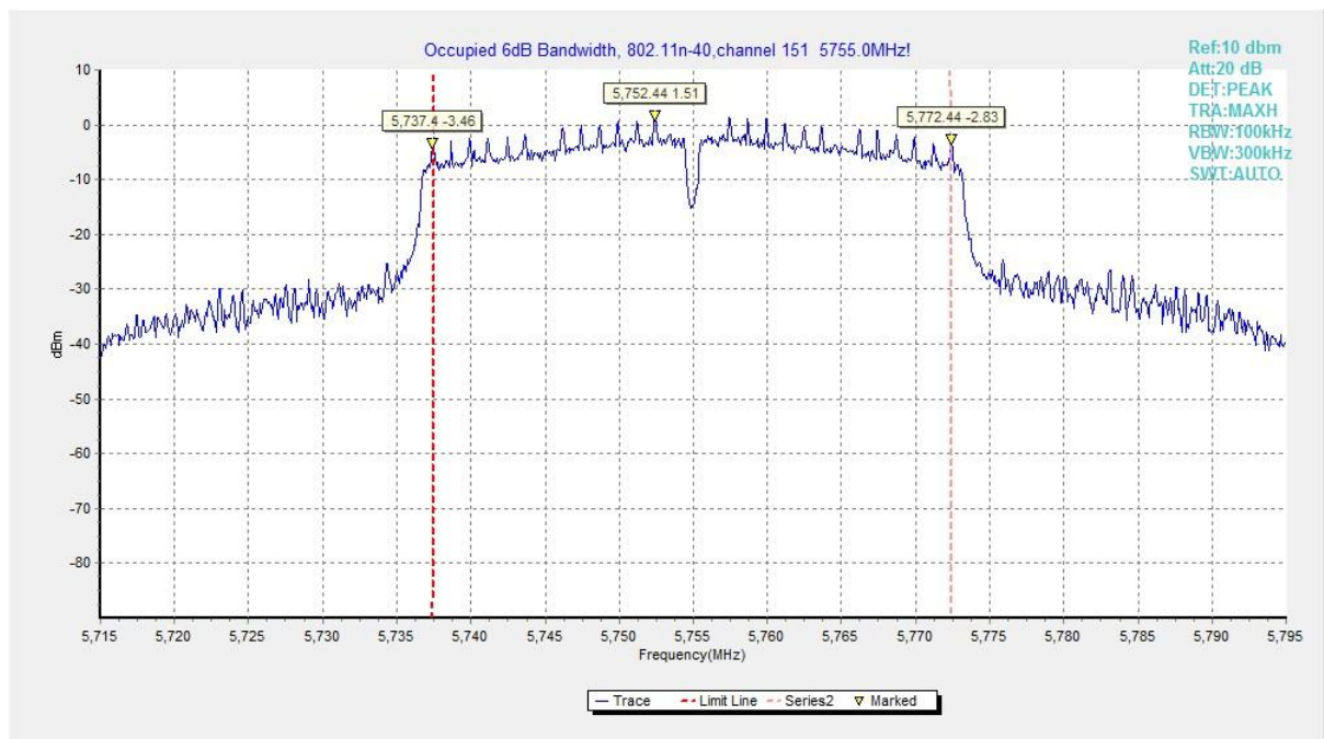
Fig. 18 Occupied 6dB Bandwidth (802.11n-HT40, 5755MHz)
