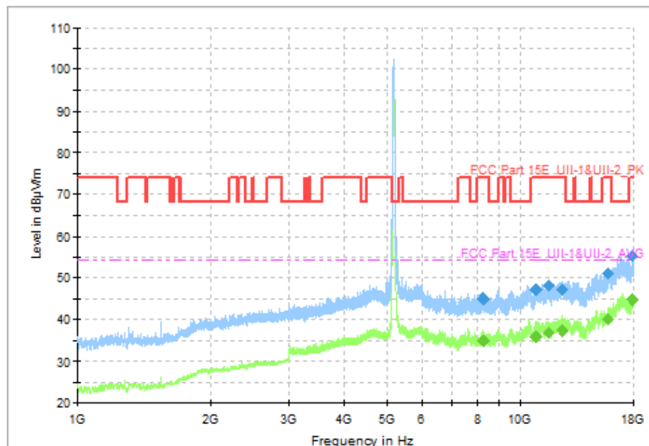
Fig. 65 Transmitter Spurious Emission (802.11n-HT40, CH38 5190MHz)
