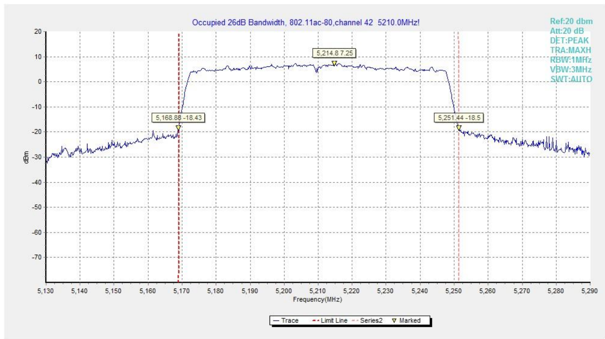
Fig. 13 Occupied 26dB Bandwidth (802. 11ac-VHT80, 5210MHz)
