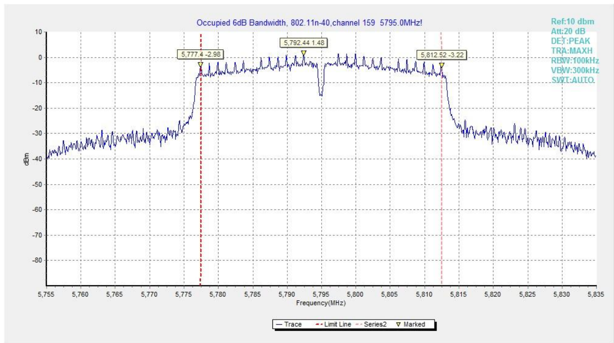
Fig. 19 Occupied 6dB Bandwidth (802.11n-HT40, 5795MHz)
