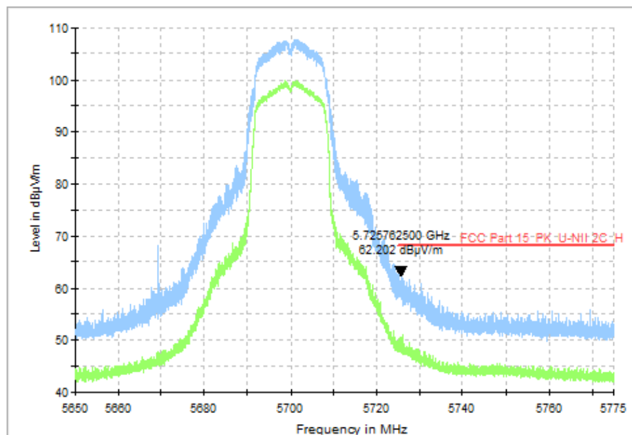
Fig. 44 Band Edges (802.11a, CH140 5700MHz)
