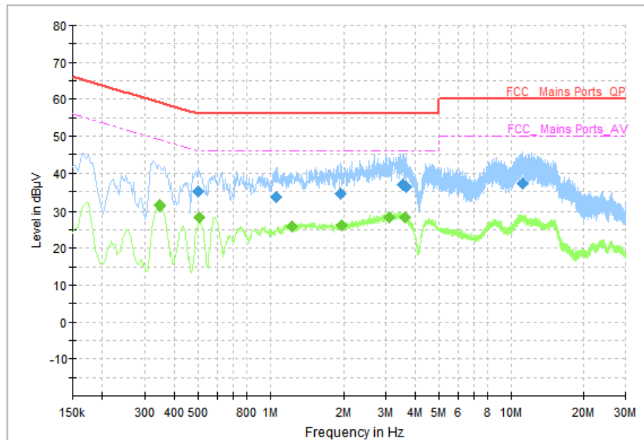
Fig. 82 AC Power line Conducted Emission (Idle)
