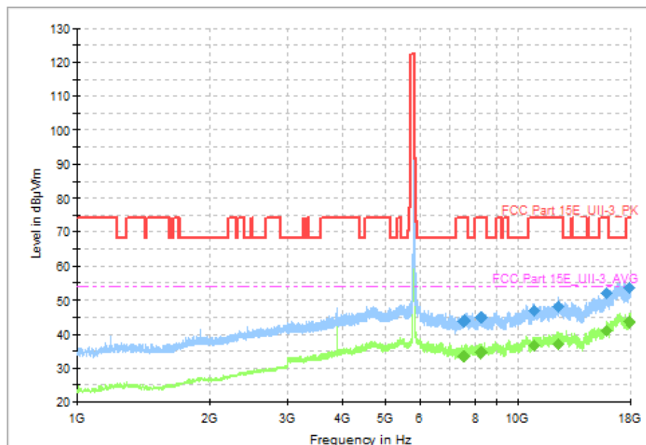
Fig. 64 Transmitter Spurious Emission (802. 11a, CH165 5825MHz)
