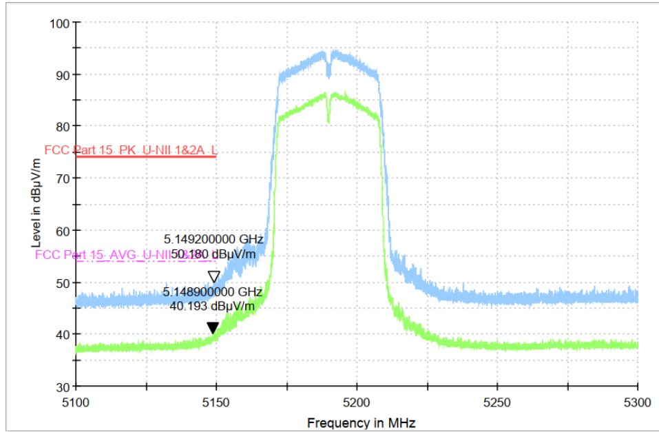
Fig. 47 Band Edges (802.11n-HT40, CH38 5190MHz)
