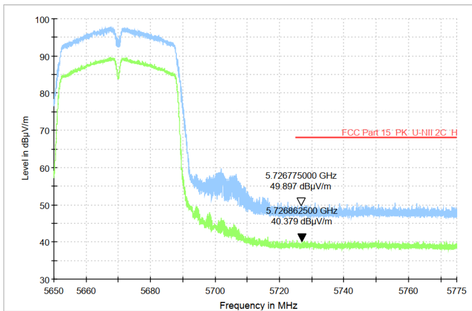
Fig. 50 Band Edges (802.11n-HT40, CH134 5670MHz)
