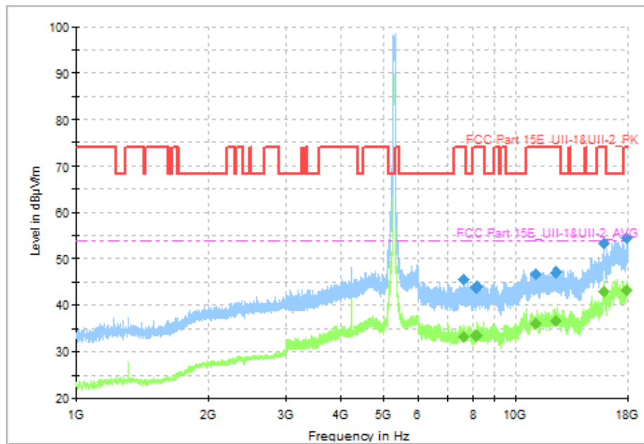
Fig. 74 Transmitter Spurious Emission (802. 11ac-VHT80, CH58 5290MHz)
