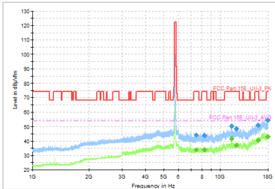
Fig. 71 Transmitter Spurious Emission (802. 11n-HT40, CH151 5755MHz)
