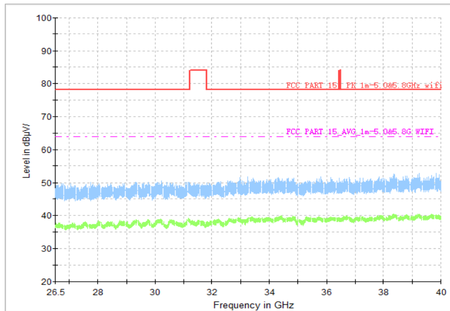
Fig. 79 Transmitter Spurious Emission (All channel, 26.5GHz~40GHz)
