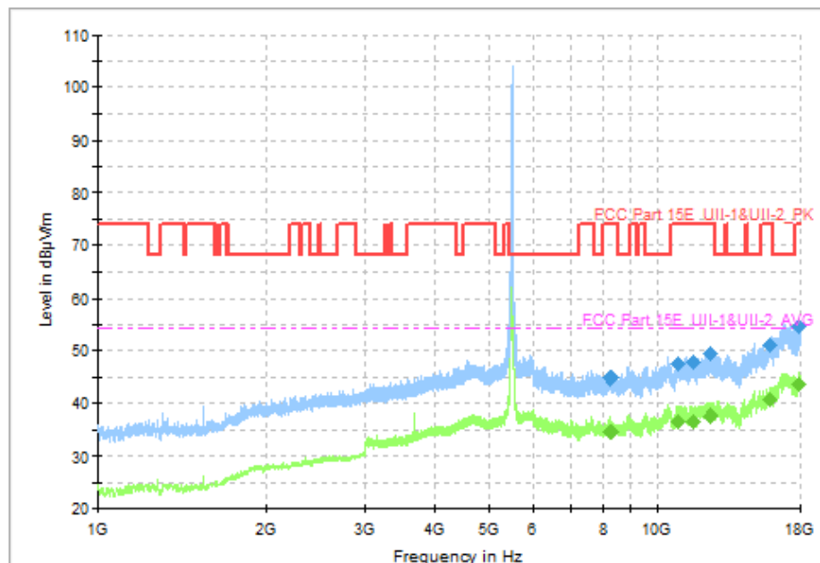
Fig. 69 Transmitter Spurious Emission (802.11n-HT40, CH102 5510MHz)
