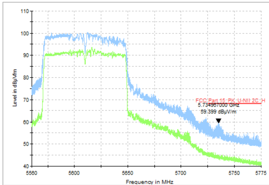
Fig. 55 Band Edges (802.11ac-VHT80, CH122 5610MHz)
