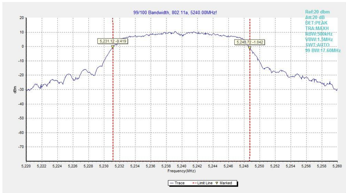
Fig. 22 99% Occupied Bandwidth (802.11a, 5240MHz)
