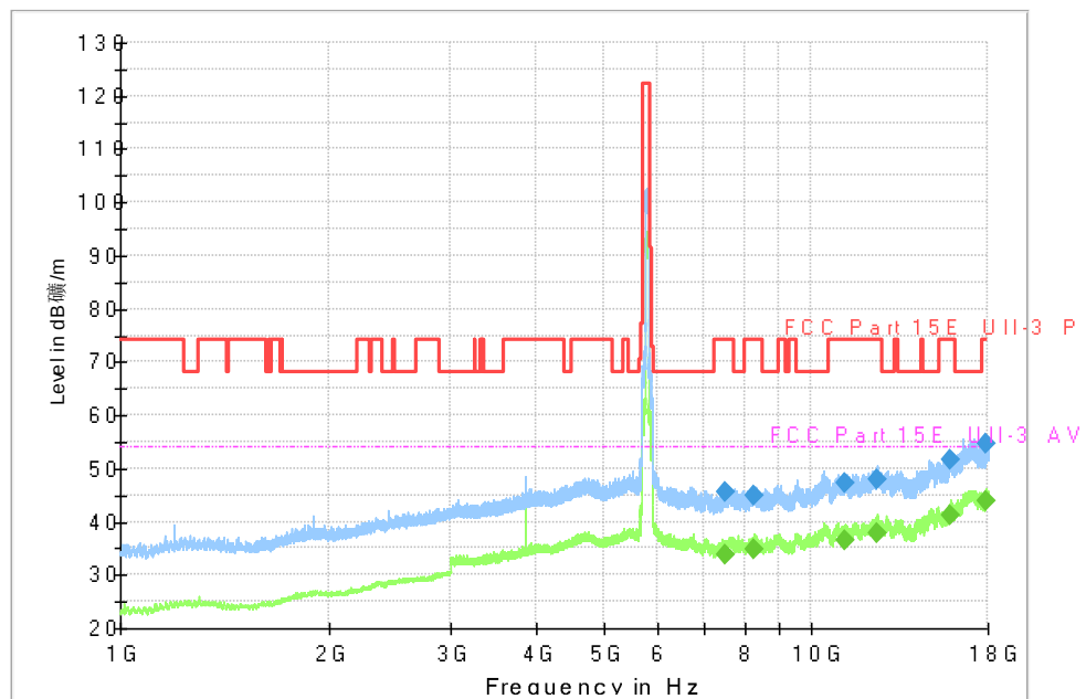
Fig. 76 Transmitter Spurious Emission (802. 11ac-VHT80, CH155 5775MHz)
