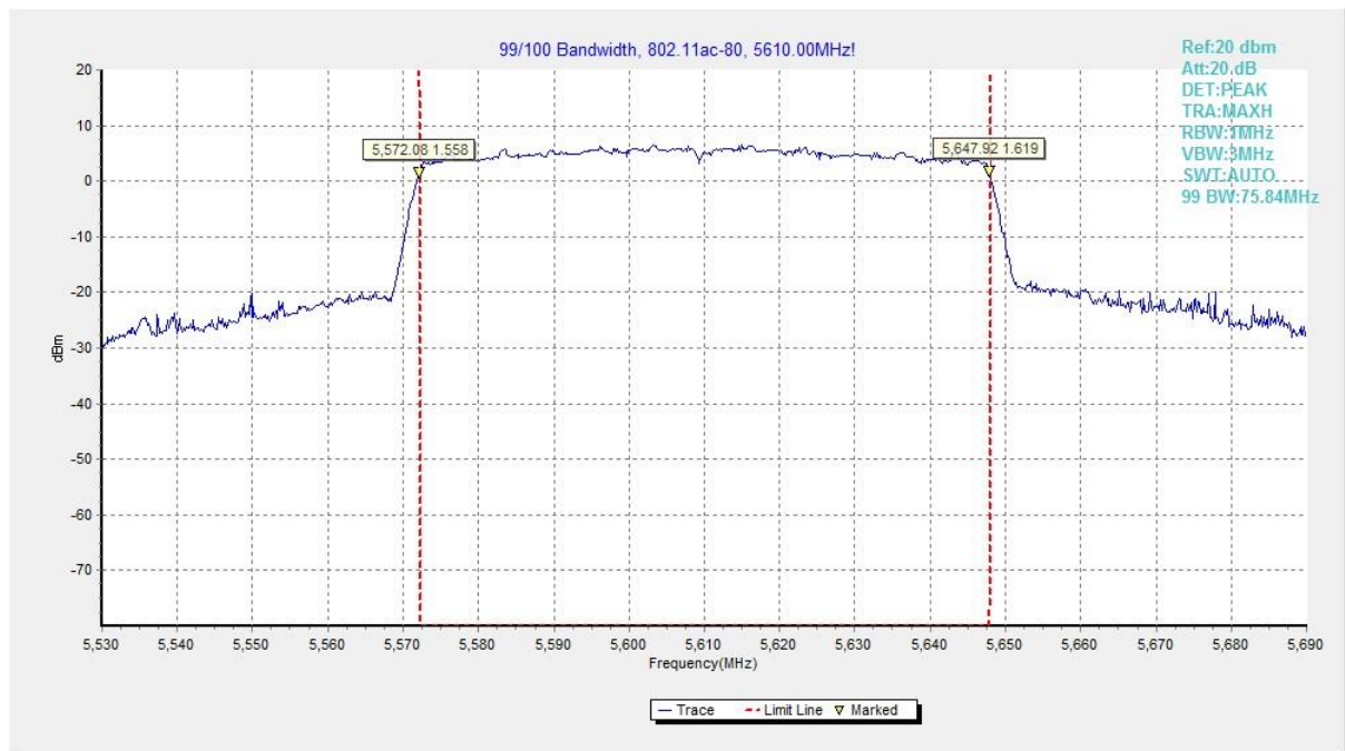
Fig. 39 99% Occupied Bandwidth (802.11ac-VHT80, 5610MHz)
