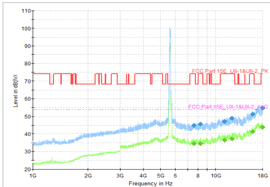
Fig. 75 Transmitter Spurious Emission (802. 11ac-VHT80, CH122 5610MHz)
