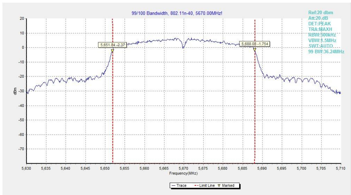
Fig. 34 99% Occupied Bandwidth (802.11n-HT40, 5670MHz)
