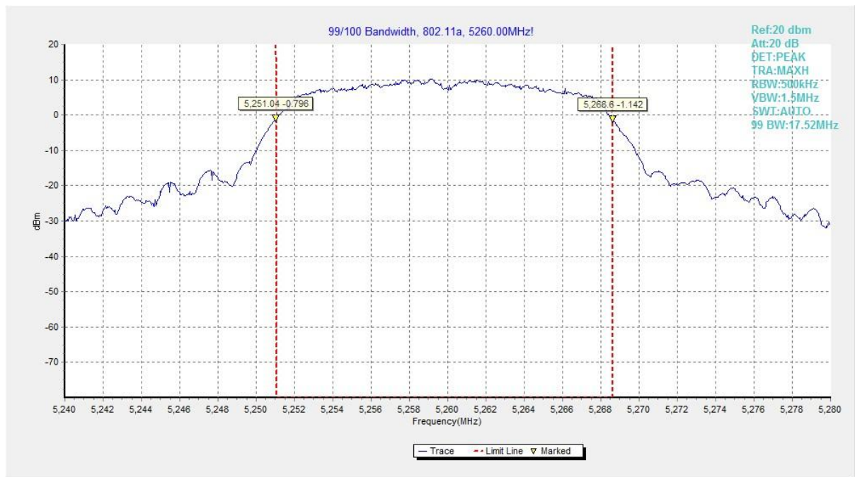
Fig. 23 99% Occupied Bandwidth (802.11a, 5260MHz)
