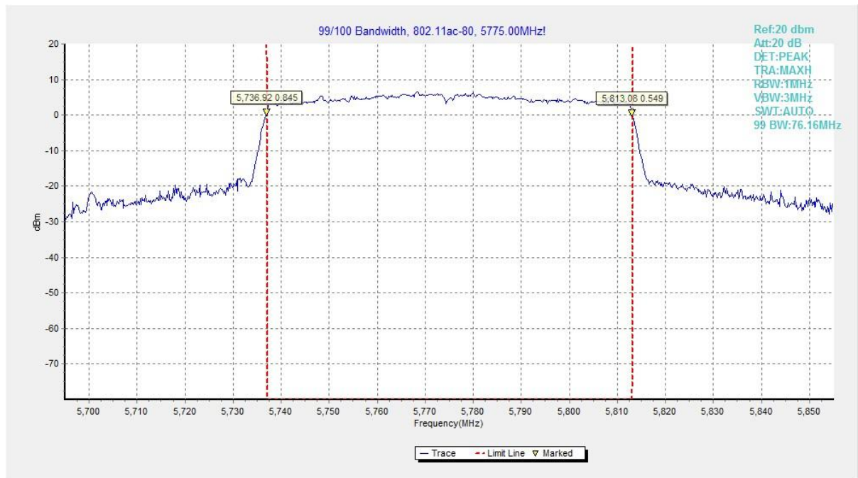
Fig. 40 99% Occupied Bandwidth (802.11ac-VHT80, 5775MHz)
