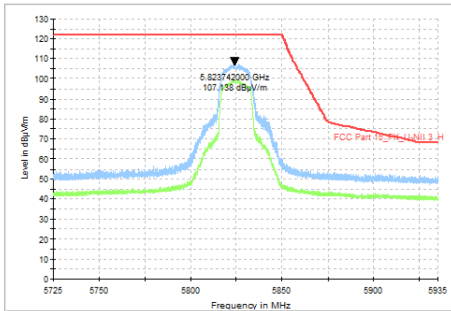
Fig. 46 Band Edges (802.11a, CH165 5825MHz)
