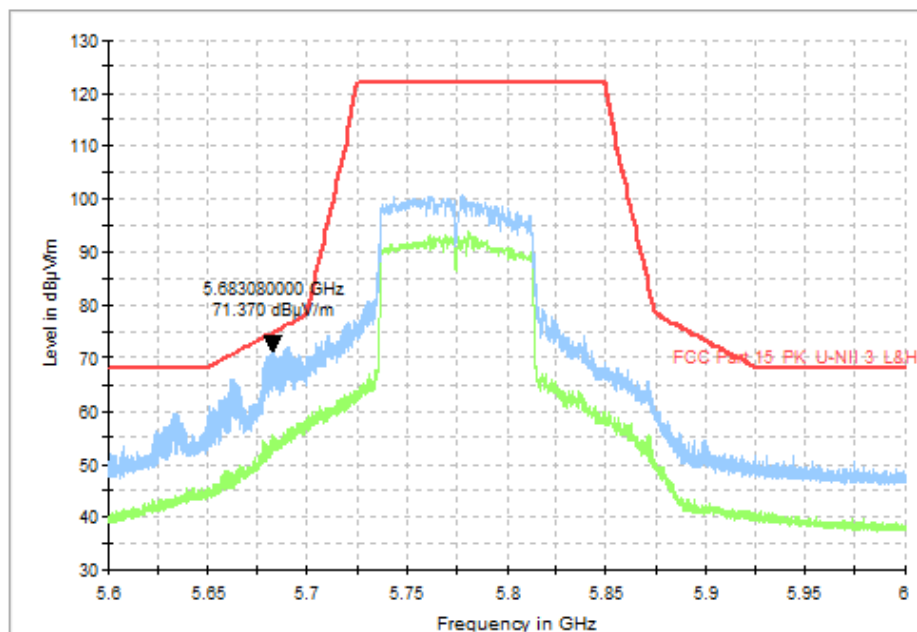
Fig. 56 Band Edges (802.11ac-VHT80, CH155 5775MHz)
