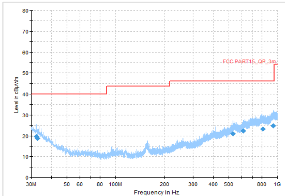
Fig. 77 Transmitter Spurious Emission (All channel, 30MHz~1GHz)
