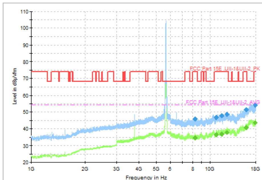
Fig. 70 Transmitter Spurious Emission (802.11n-HT40, CH134 5670MHz)
