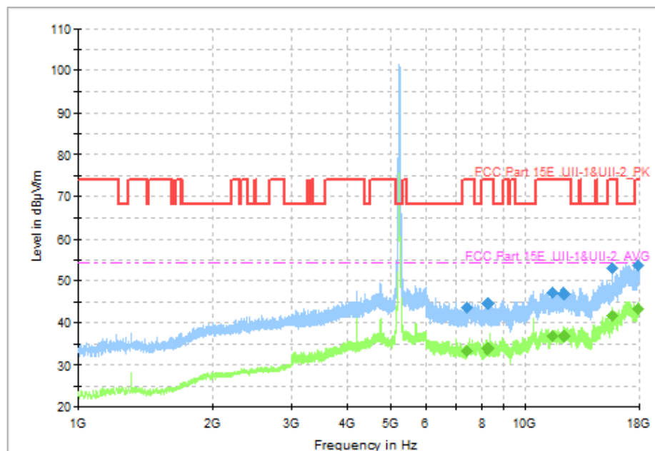
Fig. 66 Transmitter Spurious Emission (802.11n-HT40, CH46 5230MHz)
