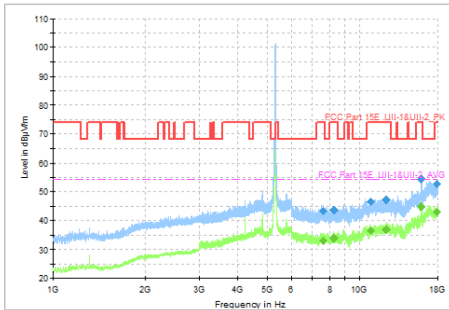
Fig. 68 Transmitter Spurious Emission (802.11n-HT40, CH62 5310MHz)
