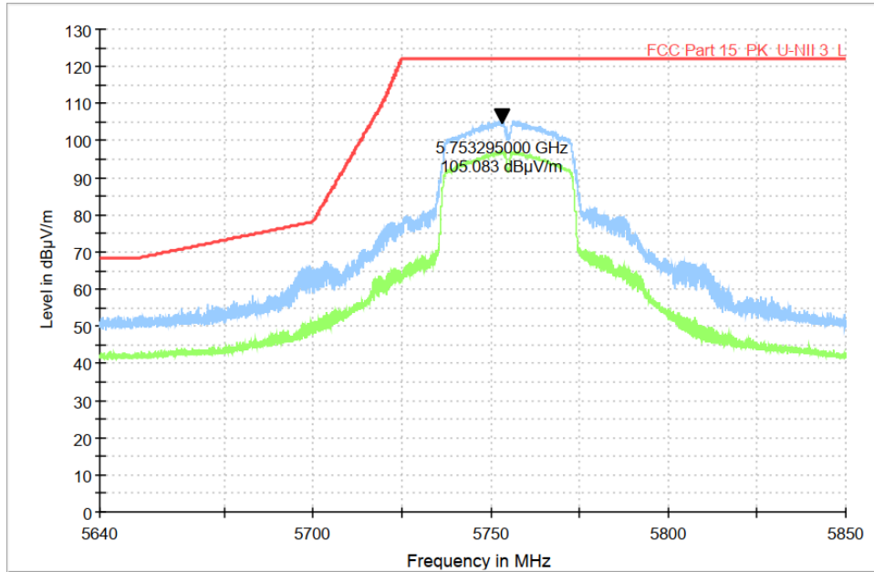
Fig. 51 Band Edges (802.11n-HT40, CH151 5755MHz)
