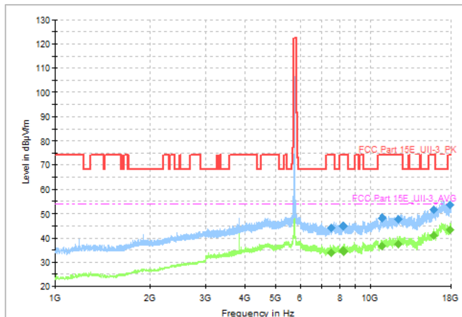
Fig. 63 Transmitter Spurious Emission (802. 11a, CH149 5745MHz)
