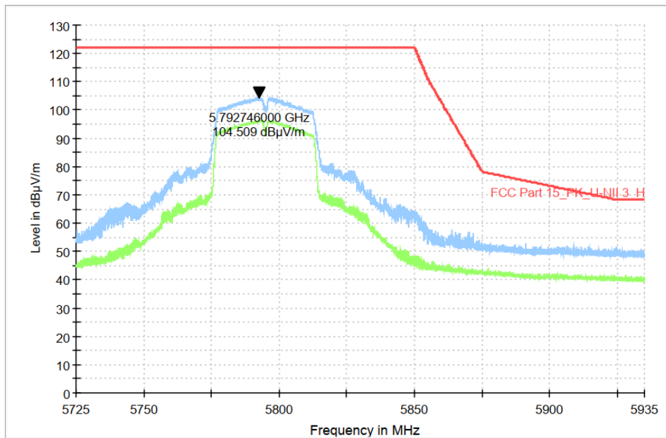
Fig. 52 Band Edges (802.11n-HT40, CH159 5795MHz)
