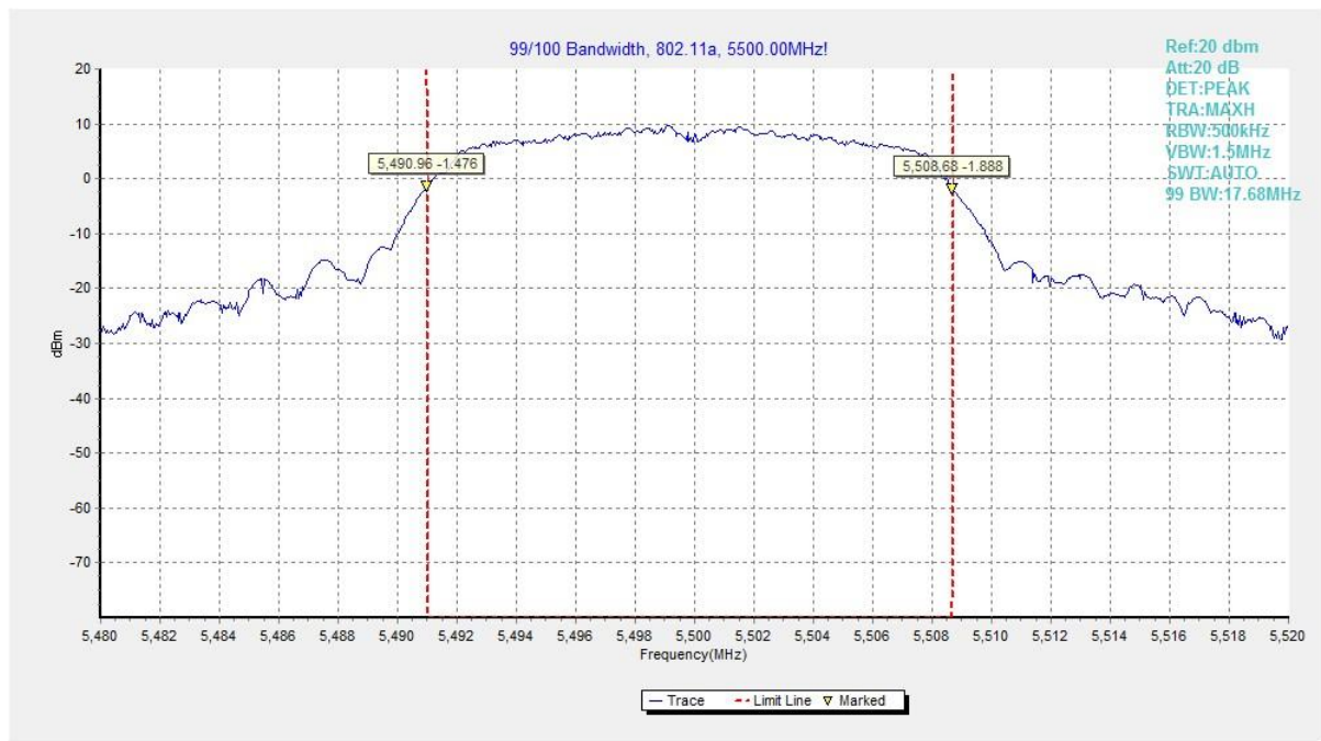
Fig. 25 99% Occupied Bandwidth (802.11a, 5500MHz)
