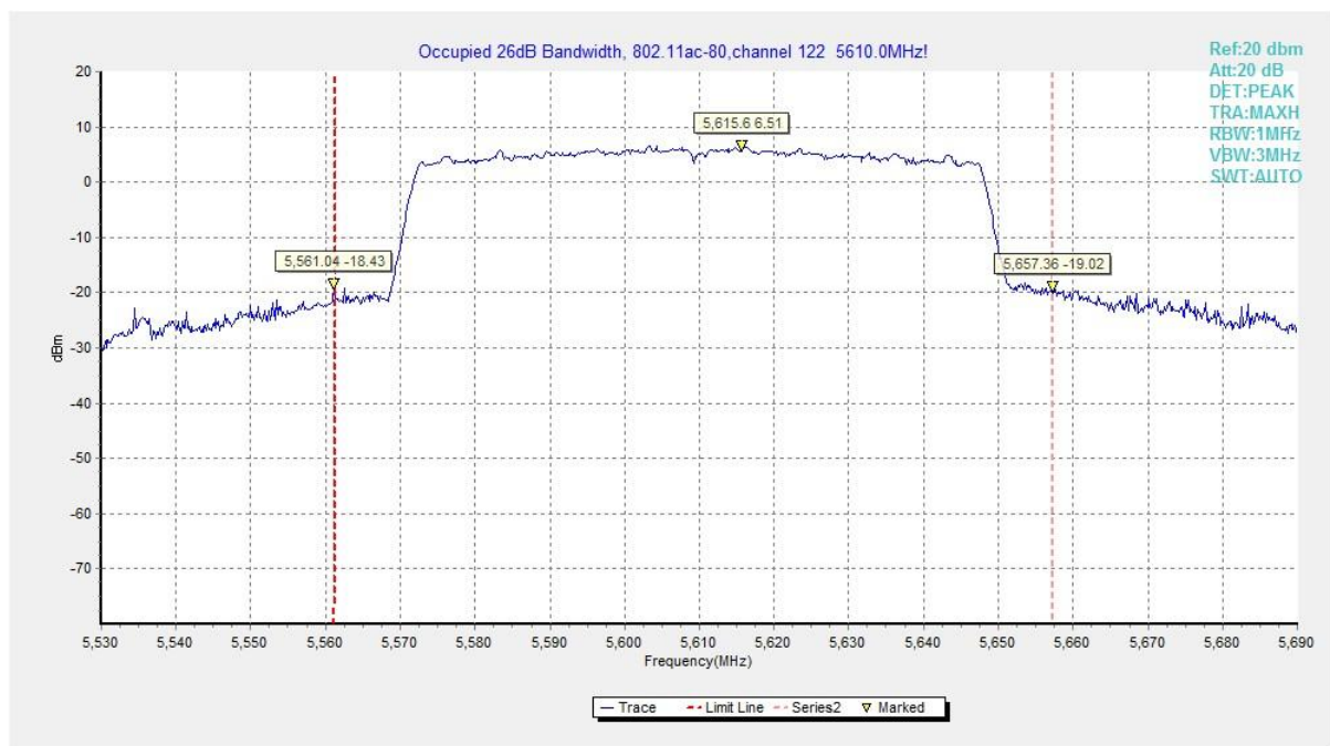
Fig. 15 Occupied 26dB Bandwidth (802. 11ac-VHT80, 5610MHz)
