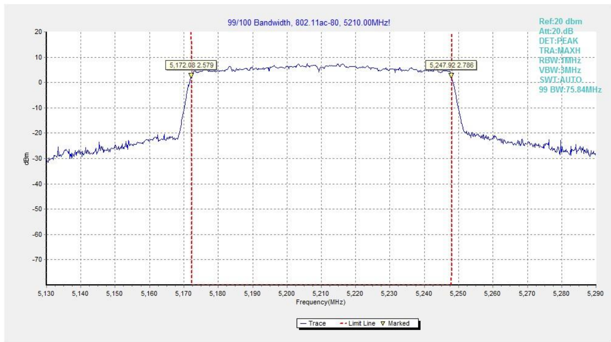
Fig. 37 99% Occupied Bandwidth (802. 11ac-VHT80, 5210MHz)
