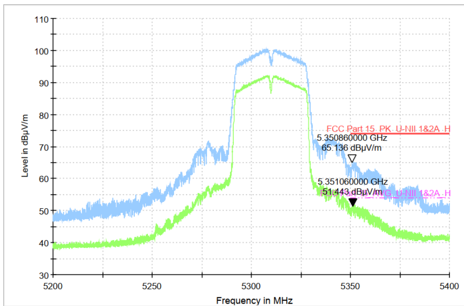
Fig. 48 Band Edges (802.11n-HT40, CH62 5310MHz)
