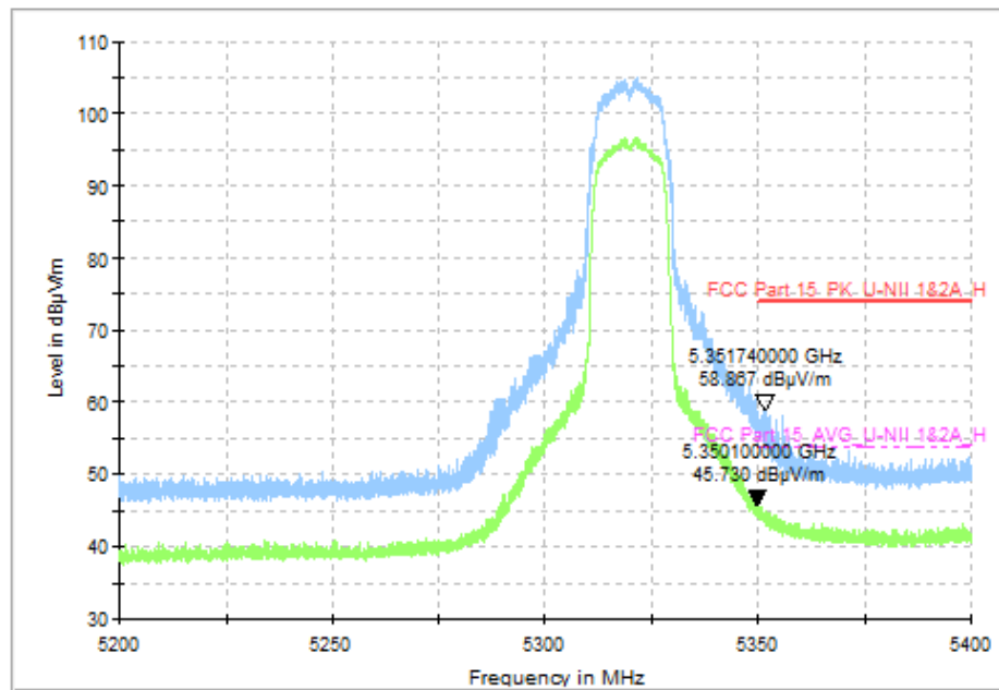
Fig. 42 Band Edges (802.11a, CH64 5320MHz)
