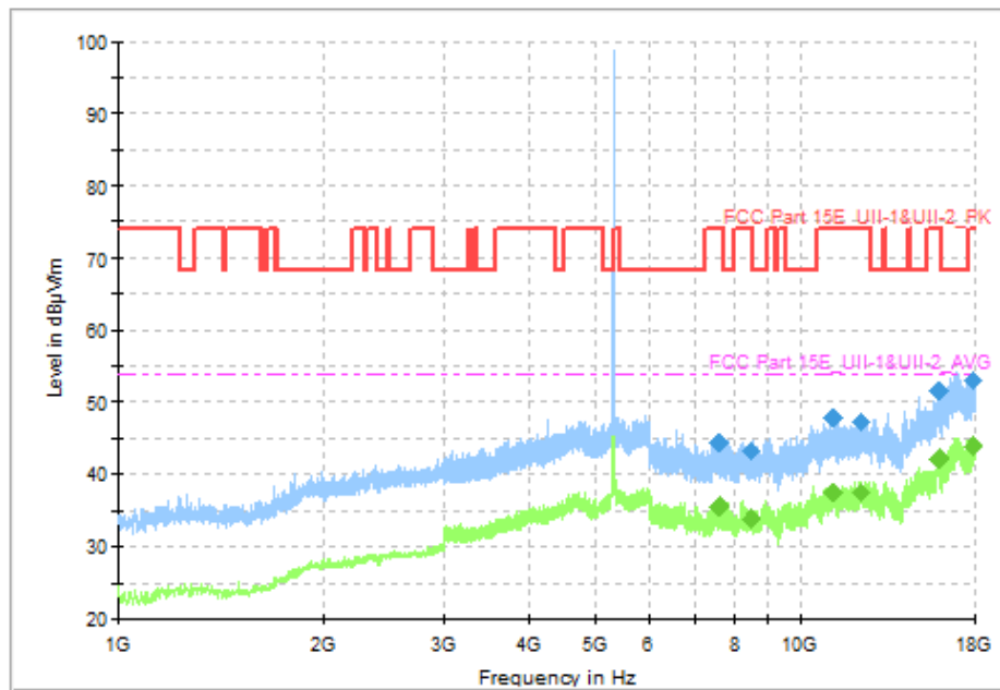
Fig. 60 Transmitter Spurious Emission (802.11a, CH64 5320MHz)
