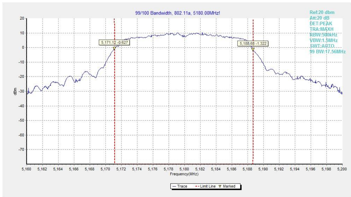
Fig. 21 99% Occupied Bandwidth (802.11a, 5180MHz)
