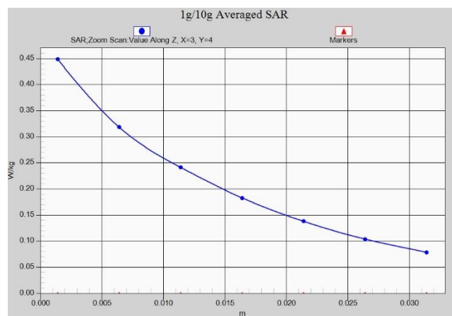
Z-Scan at power reference point (LTE B71 Body)
