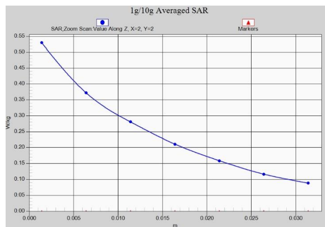
Z-Scan at power reference point (LTE B12 Body)
