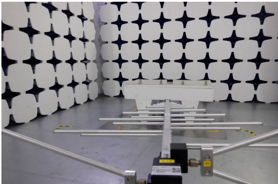
Radiated Spurious Emissions Below 1GHz
