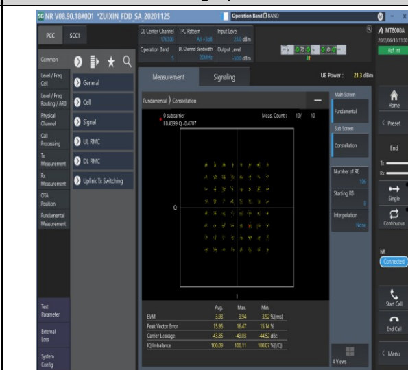
1-N5--15-20-M-8-CP-64QAM-Outer_Full-106@0-Ant1 t1-see graph-PASS
