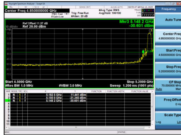
11N20SISO-Ant1-5180-PASS
