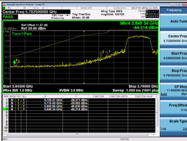
11AC40SISO-Ant1-5755-PASS
