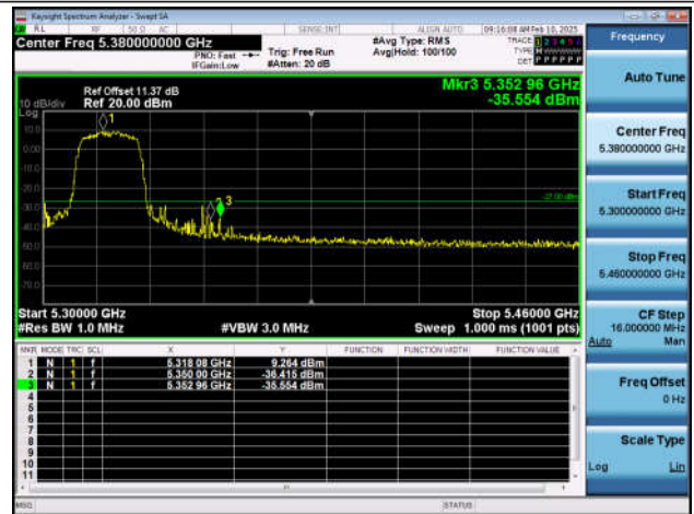
11AC40SISO-Ant1-5310-PASS
