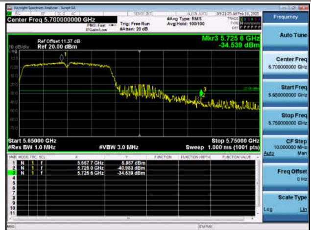
11N40SISO-Ant1-5670-PASS
