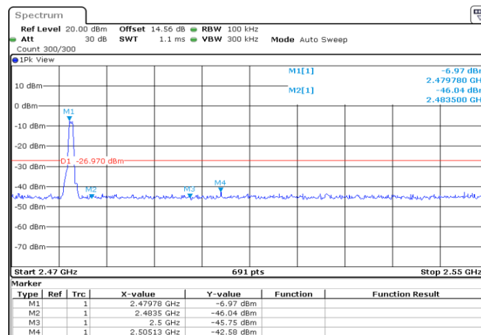
BLE_BT4.0_Ant1_High_2480
