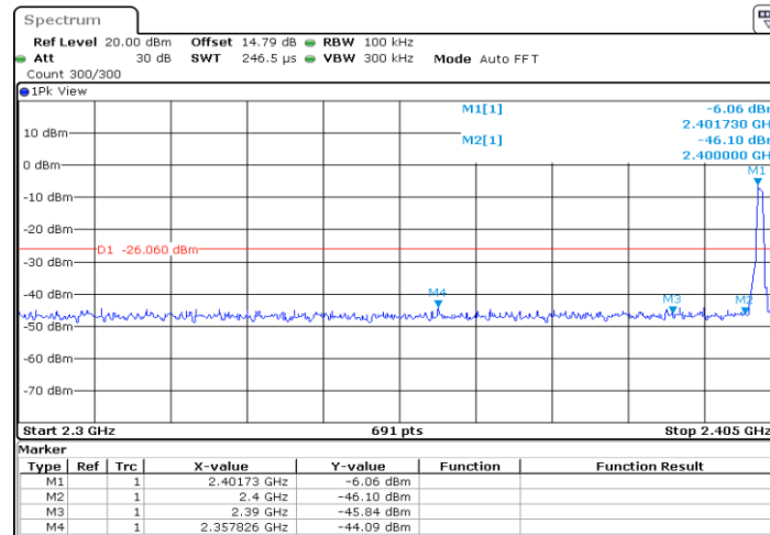
BLE_BT4.0_Ant1_Low_2402
