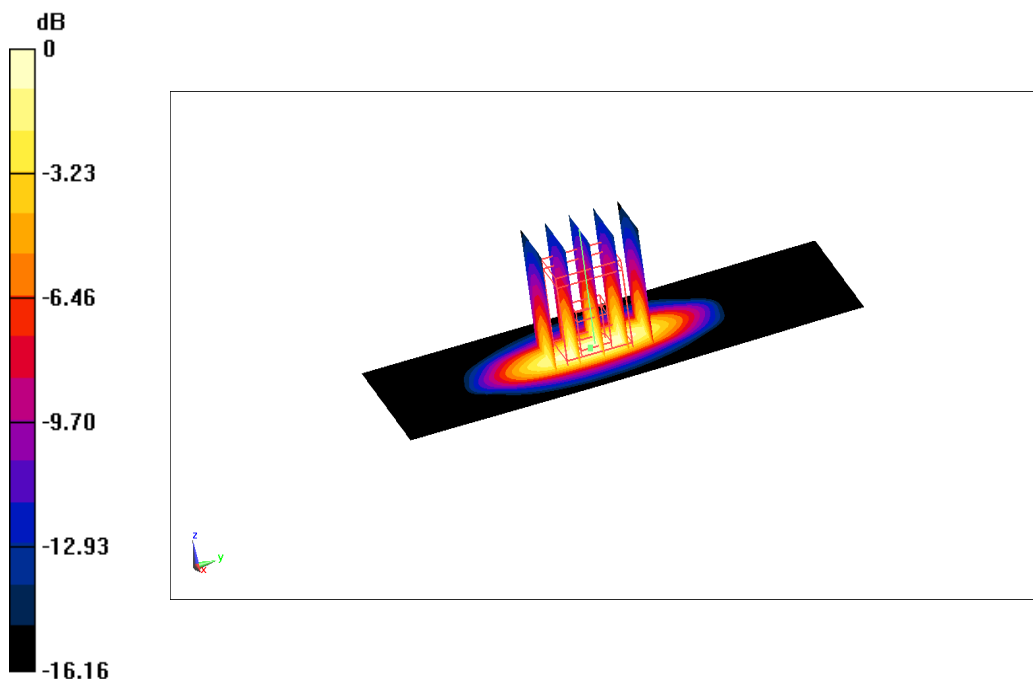
Fig.B.19 validation 1750 MHz 250mW
