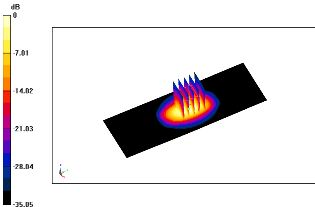
Fig.B.5 validation 1750 MHz 250mW
