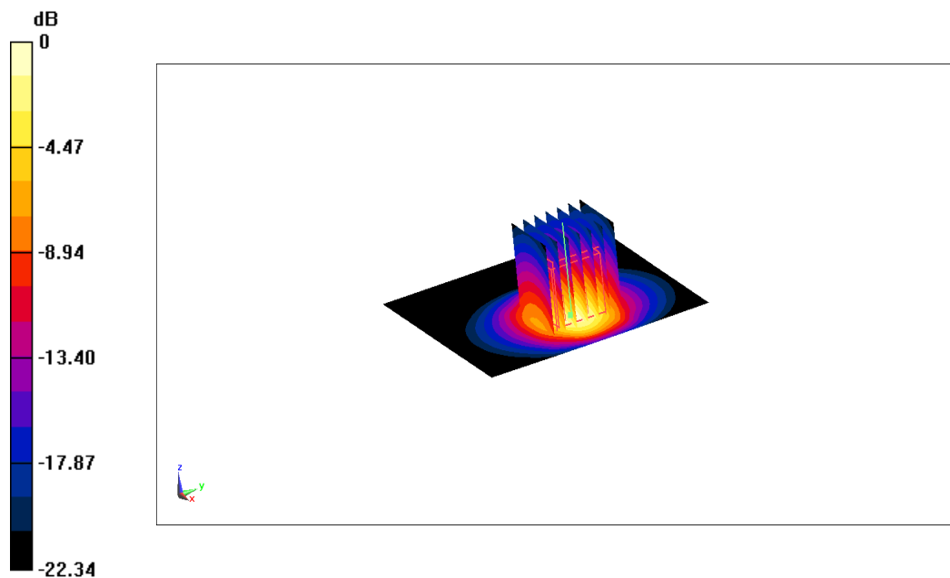
Fig.B.13 validation 2450 MHz 250m
