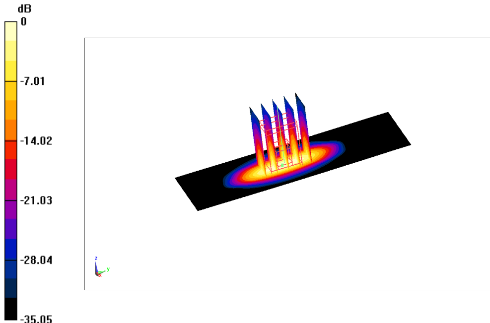
Fig.B.6 validation 1750 MHz 250mW
