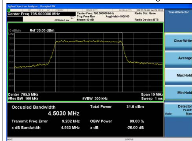
LTE Band 14 QPSK 5MHz CH-High
