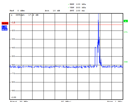
LTE Band 14 10MHz CH- Middle 30MHz~1GHz
