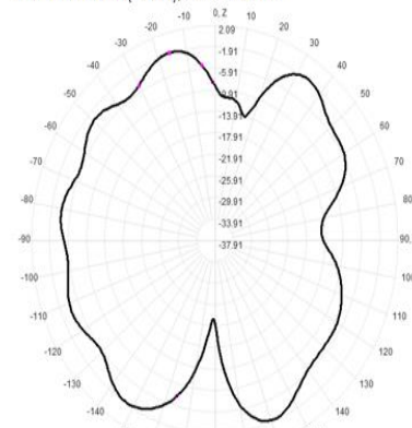
2440.0MHz Total(E2-YZ), Max= -1.59dBi
