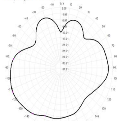
Total(H-XY), Max= 2.05dBi, CirD=16.36
