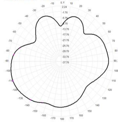
Total(H-XY), Max= 1.61dBi, CirD=14.96
