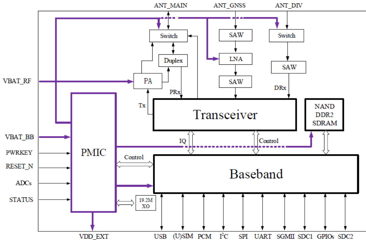
Figure 2-1 Functional Diagram
