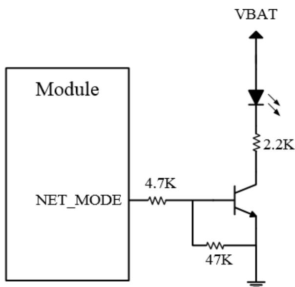
Figure 5-8 Network Indicate Light Reference Circuits
