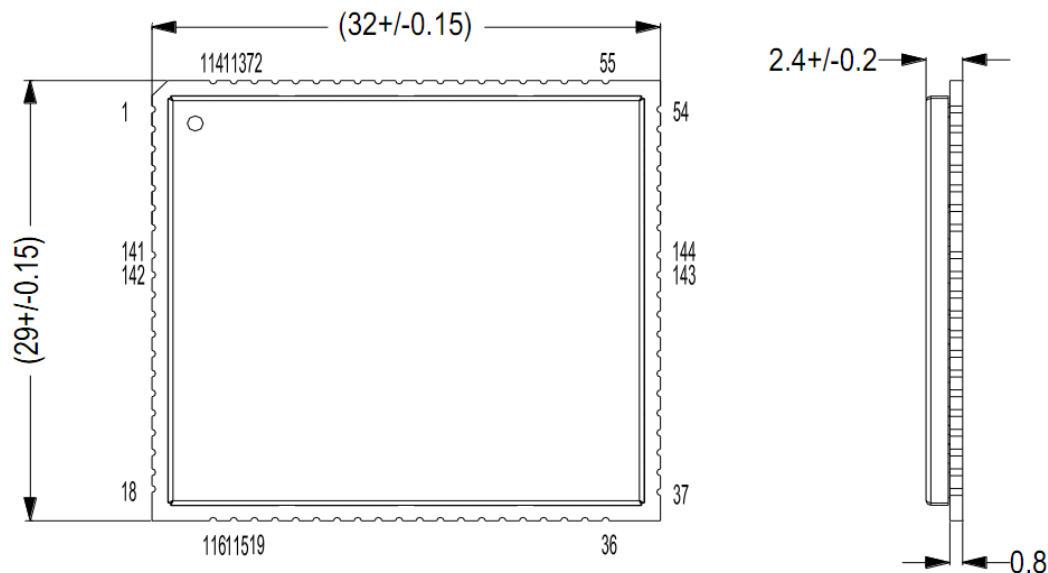
Figure 9-1 Structure Dimension (Unit: mm)
