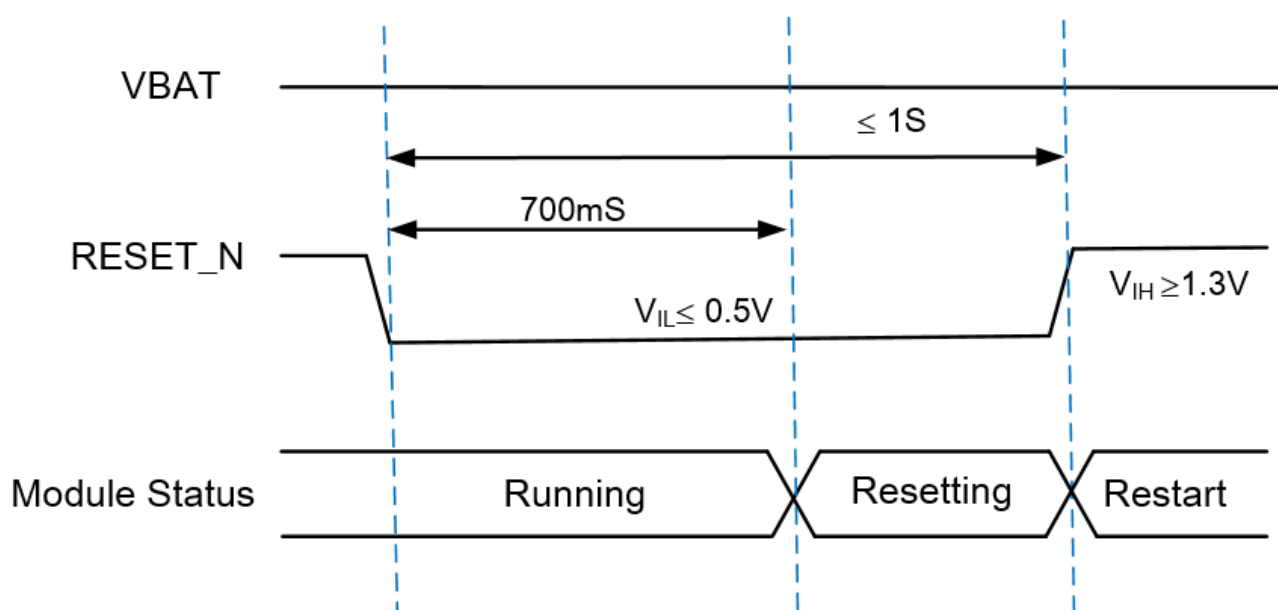
Figure 5-7 Reset Timing
