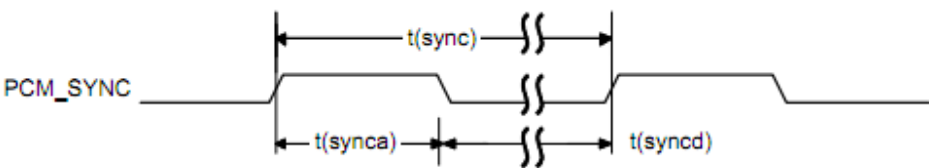
Figure 5-14 PCM_SYNC Timing
