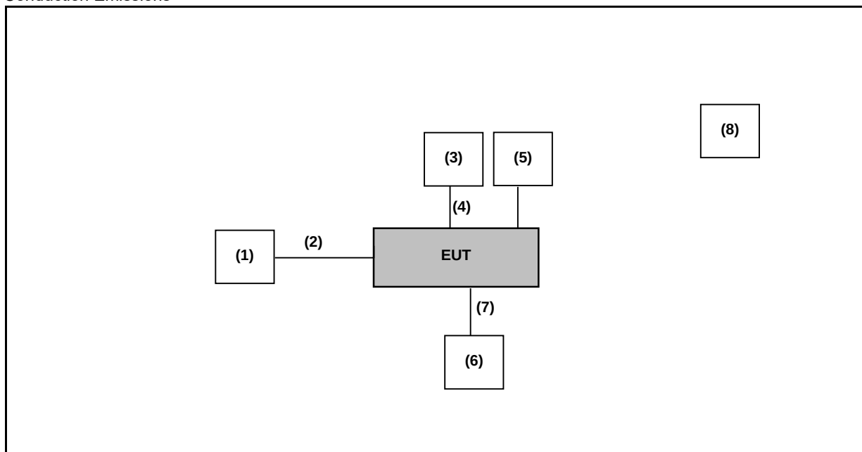
Conduction Emissions
