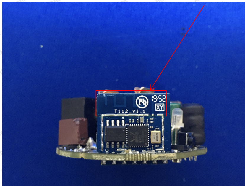
WIFI Antenna
