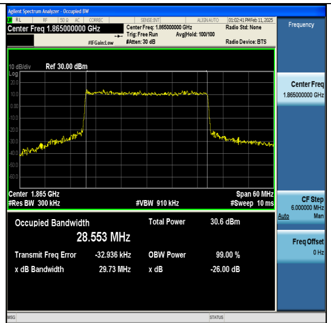
NTNV-n25-PC3-15-30-L-DFT-16QAM-Outer_Full-Ant1- PASS
