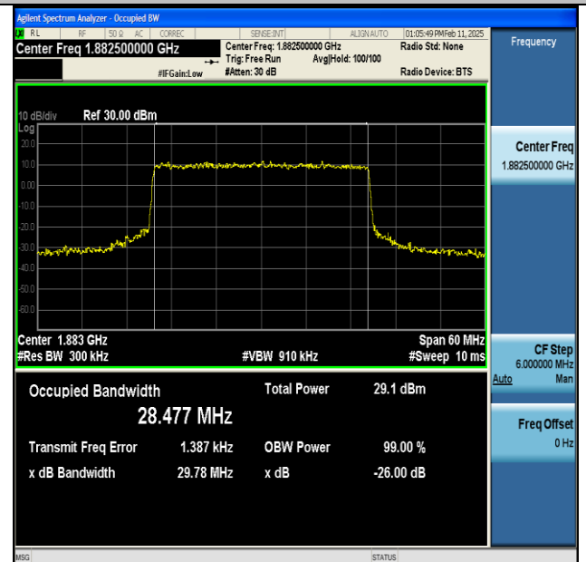
NTNV-n25-PC3-15-30-M-CP-64QAM-Outer_Full-Ant1-PASS
