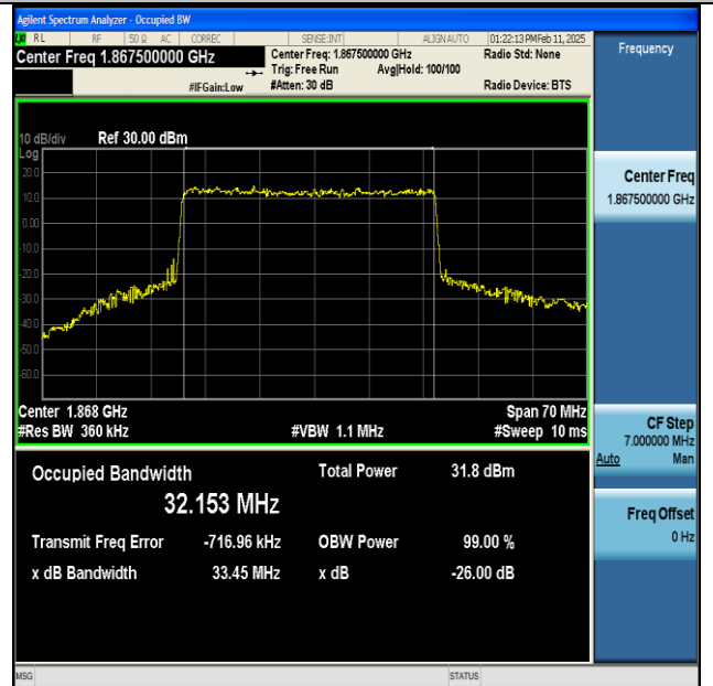
NTNV-n25-PC3-15-35-L-DFT-QPSK-Outer_Full-Ant1- PASS
