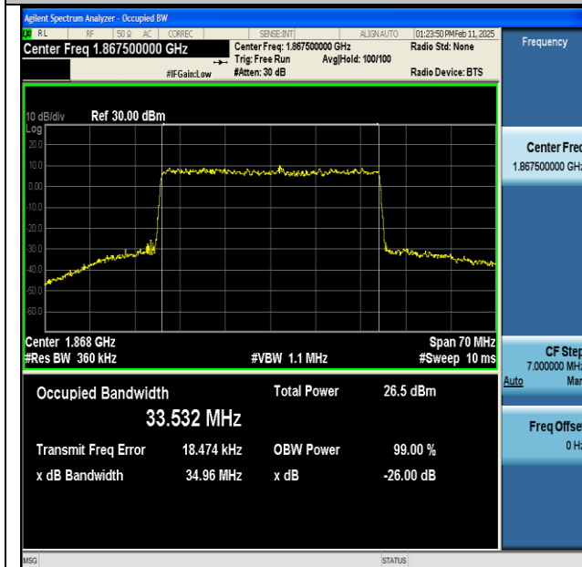
NTNV-n25-PC3-15-35-L-CP-256QAM-Outer_Full-Ant1- PASS
