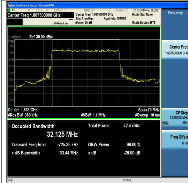
NTNV-n25-PC3-15-35-L-DFT-BPSK-Outer_Full-Ant1- PASS
