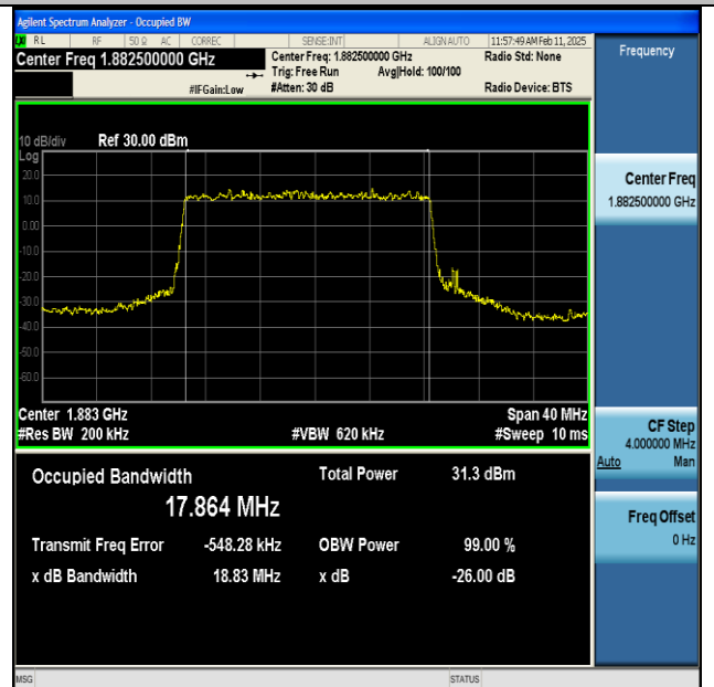
NTNV-n25-PC3-15-20-M-DFT-QPSK-Outer_Full-Ant1- PASS
