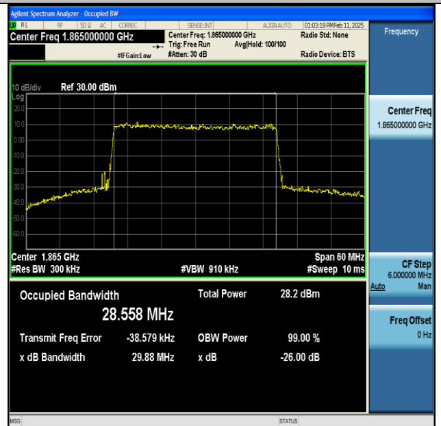
NTNV-n25-PC3-15-30-L-DFT-256QAM-Outer_Full-Ant1- PASS
