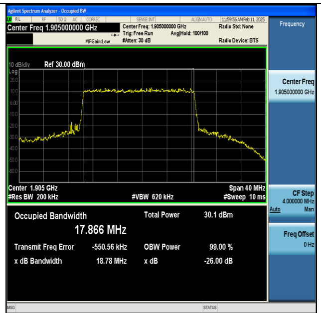
NTNV-n25-PC3-15-20-H-DFT-16QAM-Outer_Full-Ant1- PASS
