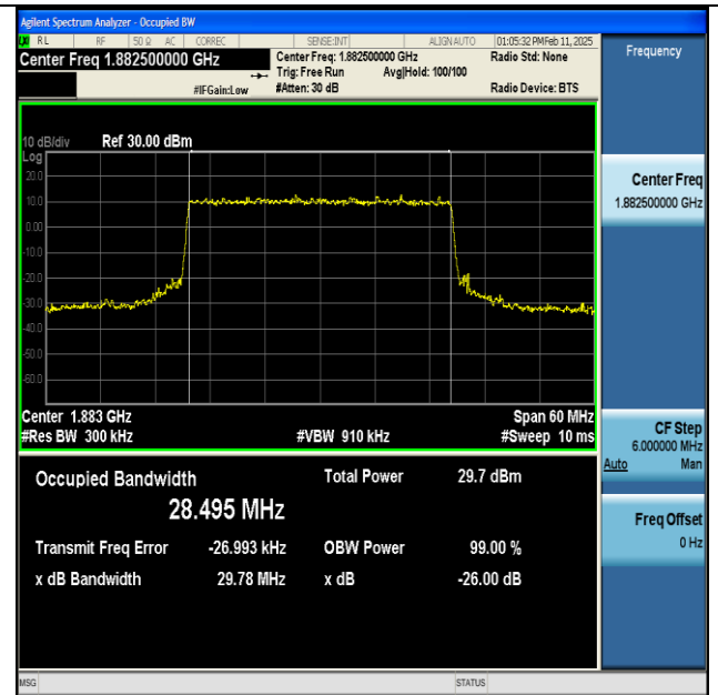
NTNV-n25-PC3-15-30-M-CP-QPSK-Outer_Full-Ant1-PASS
