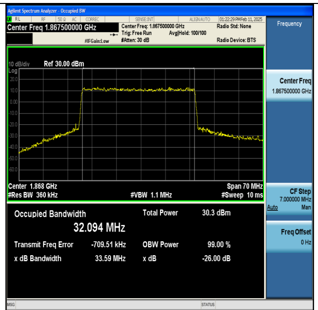
NTNV-n25-PC3-15-35-L-DFT-64QAM-Outer_Full-Ant1- PASS
