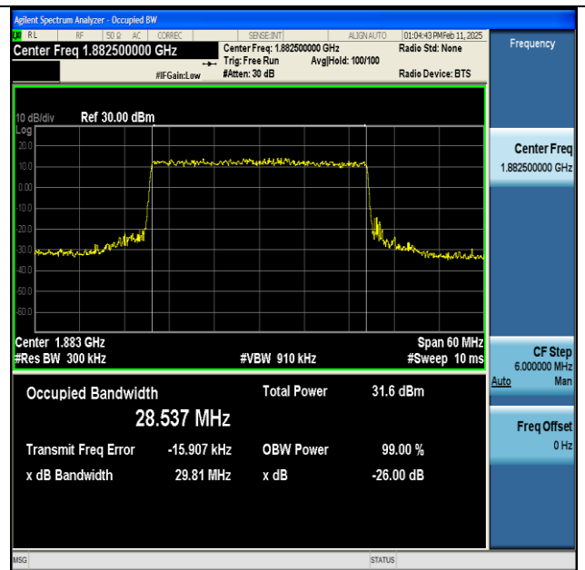
NTNV-n25-PC3-15-30-M-DFT-QPSK-Outer_Full-Ant1- PASS
