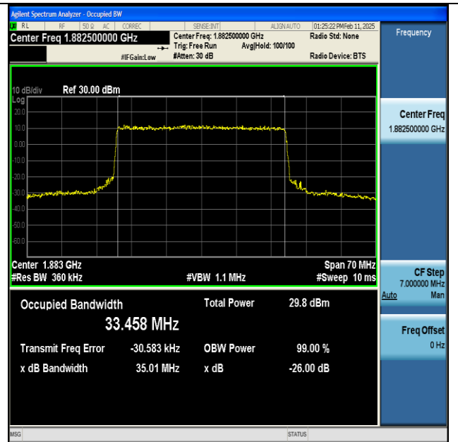
NTNV-n25-PC3-15-35-M-CP-16QAM-Outer_Full-Ant1-PASS
