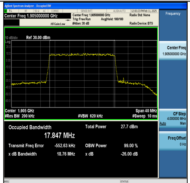
NTNV-n25-PC3-15-20-H-DFT-256QAM-Outer_Full-Ant1- PASS
