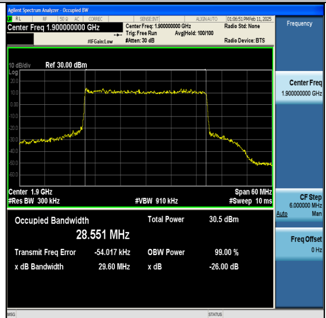
NTNV-n25-PC3-15-30-H-DFT-16QAM-Outer_Full-Ant1- PASS
