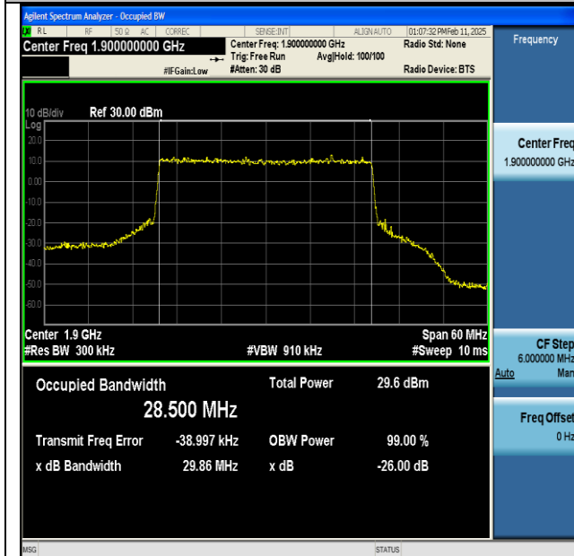
NTNV-n25-PC3-15-30-H-DFT-64QAM-Outer_Full-Ant1- PASS
