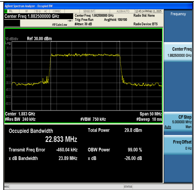
NTNV-n25-PC3-15-25-M-DFT-256QAM-Outer_Full-Ant1- PASS
