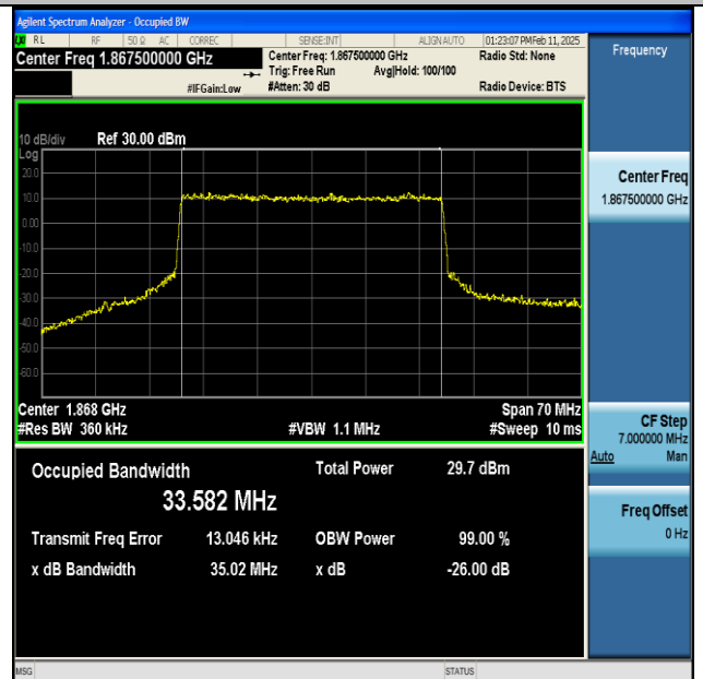
NTNV-n25-PC3-15-35-L-CP-QPSK-Outer_Full-Ant1-PASS
