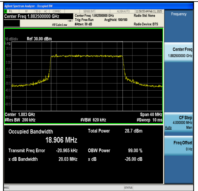
NTNV-n25-PC3-15-20-M-CP-64QAM-Outer_Full-Ant1- PASS
