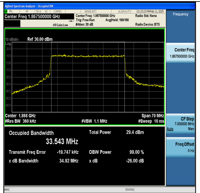
NTNV-n25-PC3-15-35-L-CP-64QAM-Outer_Full-Ant1- PASS
