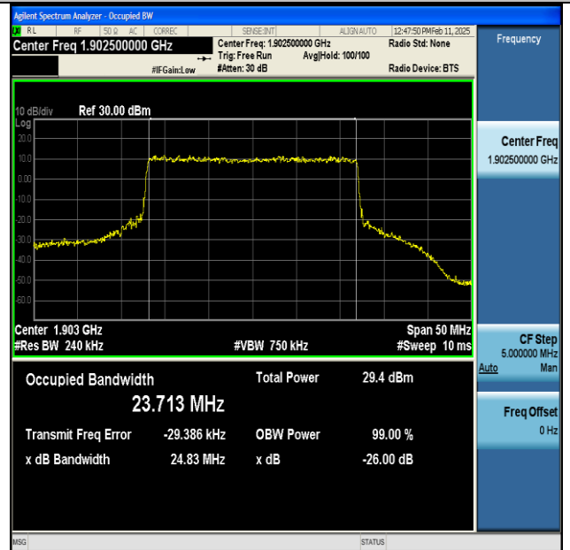
NTNV-n25-PC3-15-25-H-DFT-64QAM-Outer_Full-Ant1- PASS
