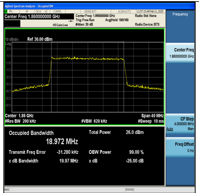
NTNV-n25-PC3-15-20-L-CP-256QAM-Outer_Full-Ant1- PASS
