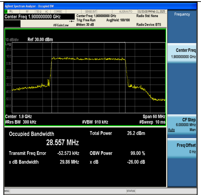
NTNV-n25-PC3-15-30-H-CP-256QAM-Outer_Full-Ant1- PASS
