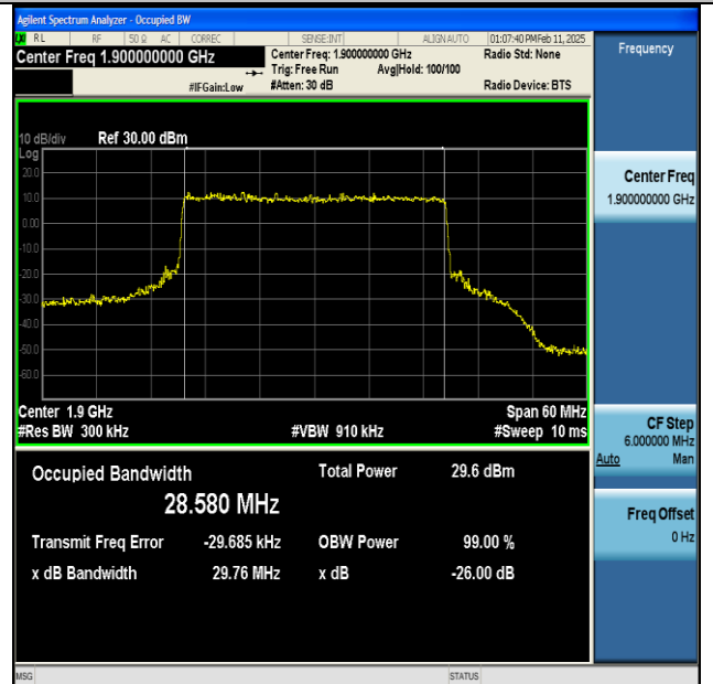
NTNV-n25-PC3-15-30-H-CP-16QAM-Outer_Full-Ant1- PASS
