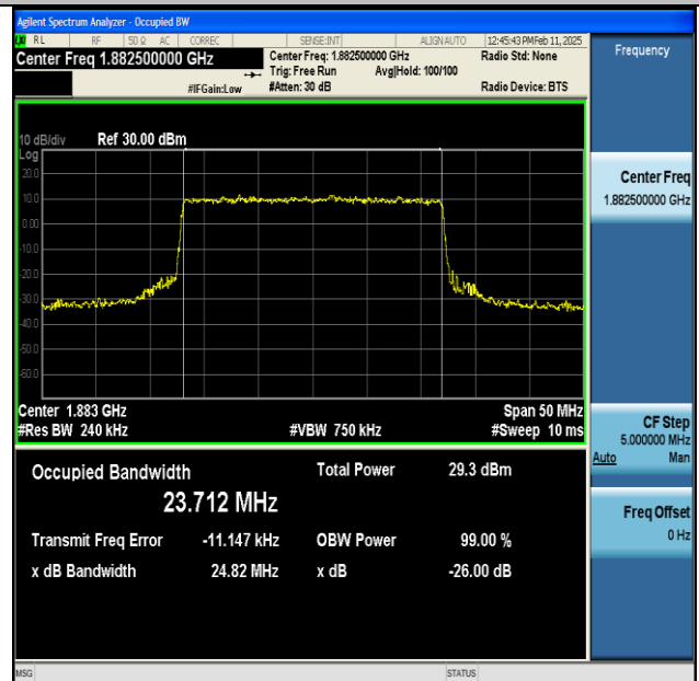
NTNV-n25-PC3-15-25-M-CP-16QAM-Outer_Full-Ant1- PASS
