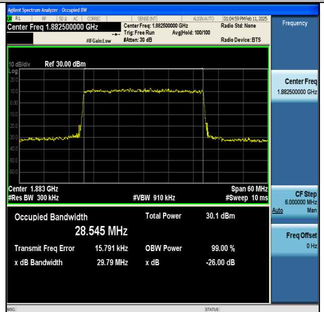
NTNV-n25-PC3-15-30-M-DFT-64QAM-Outer_Full-Ant1- PASS
