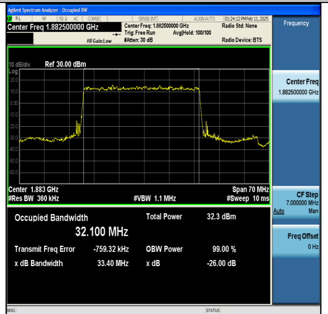
NTNV-n25-PC3-15-35-M-DFT-BPSK-Outer_Full-Ant1- PASS
