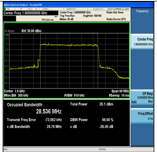
NTNV-n25-PC3-15-30-H-DFT-256QAM-Outer_Full-Ant1- PASS
