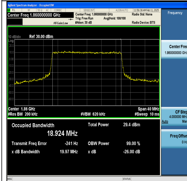
NTNV-n25-PC3-15-20-L-DFT-64QAM-Outer_Full-Ant1- PASS
