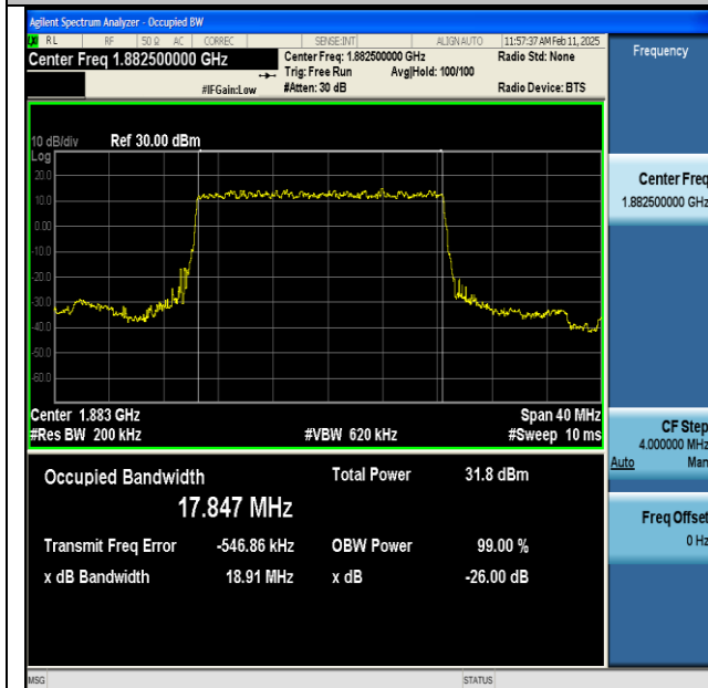
NTNV-n25-PC3-15-20-M-DFT-BPSK-Outer_Full-Ant1- PASS
