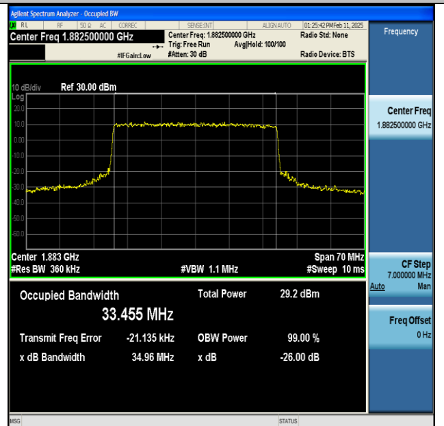
NTNV-n25-PC3-15-35-M-CP-256QAM-Outer_Full-Ant1-PASS
