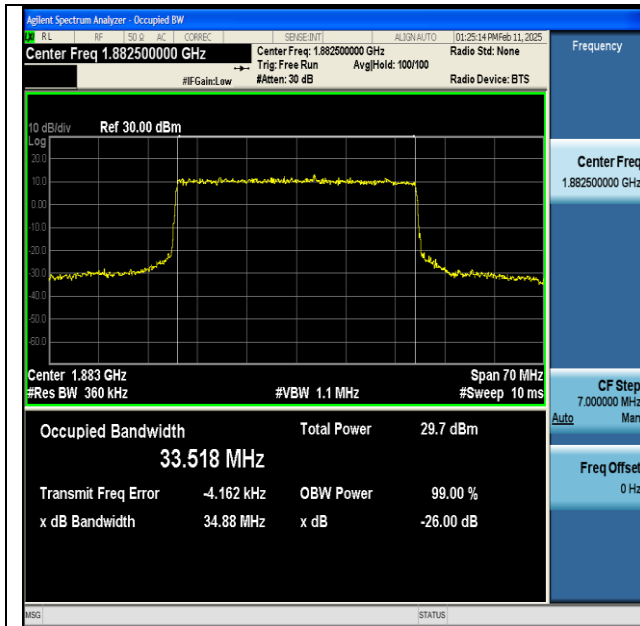
NTNV-n25-PC3-15-35-M-CP-QPSK-Outer_Full-Ant1-PASS
