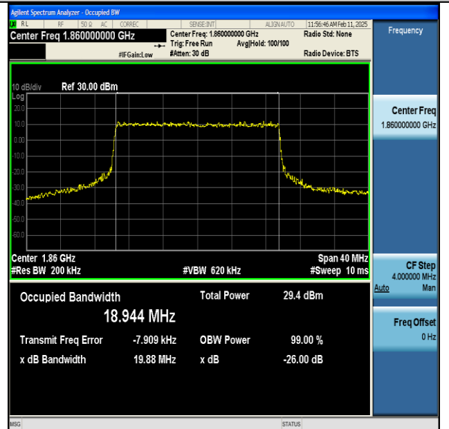
NTNV-n25-PC3-15-20-L-CP-16QAM-Outer_Full-Ant1- PASS
