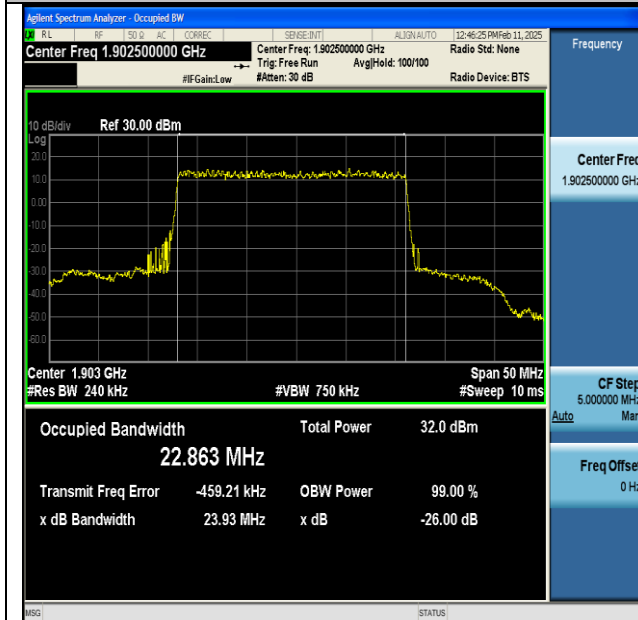
NTNV-n25-PC3-15-25-H-DFT-BPSK-Outer_Full-Ant1- PASS
