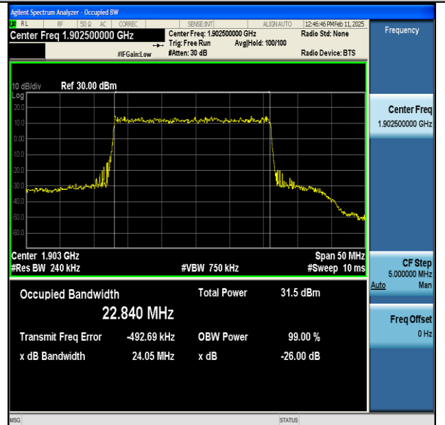
NTNV-n25-PC3-15-25-H-DFT-QPSK-Outer_Full-Ant1- PASS
