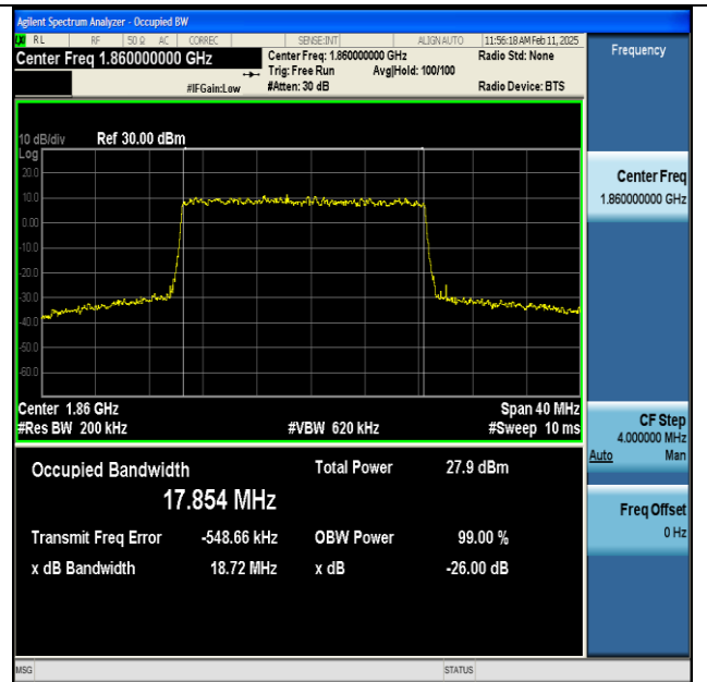
NTNV-n25-PC3-15-20-L-DFT-256QAM-Outer_Full-Ant1- PASS
