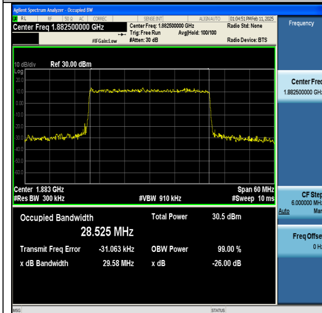
NTNV-n25-PC3-15-30-M-DFT-16QAM-Outer_Full-Ant1- PASS
