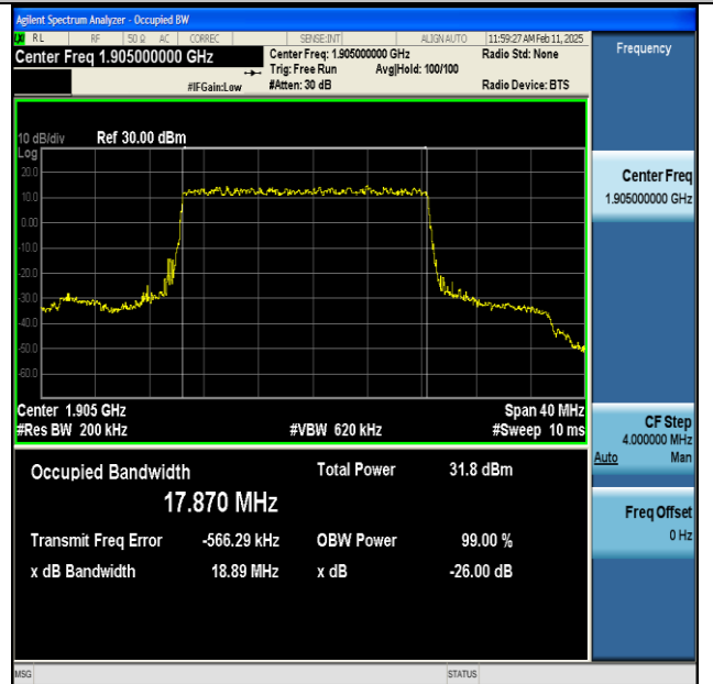
NTNV-n25-PC3-15-20-H-DFT-BPSK-Outer_Full-Ant1- PASS
