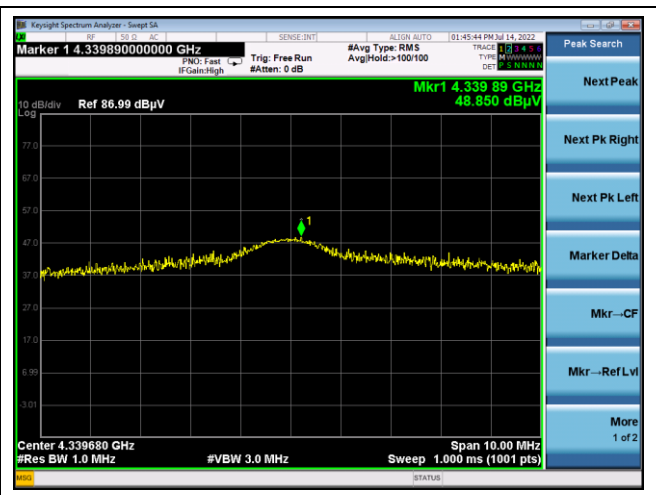
10 th harmonic
