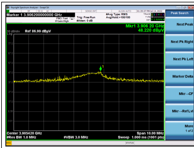
9 th harmonic
