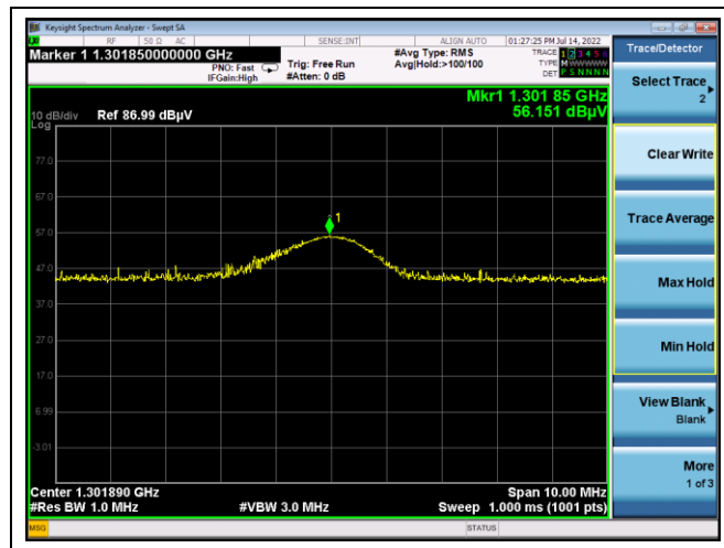
3 rd harmonic
