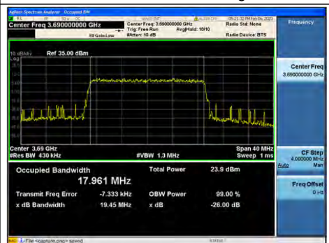
Band48 / 20MHz / 64QAM/ High CH
