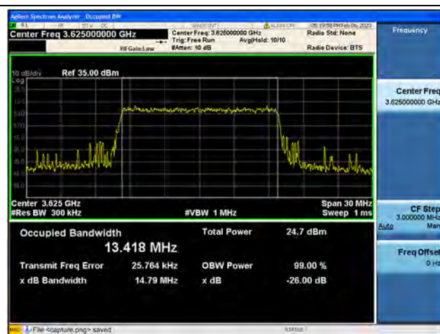
Band48 / 15MHz / 64QAM/ Mid CH
