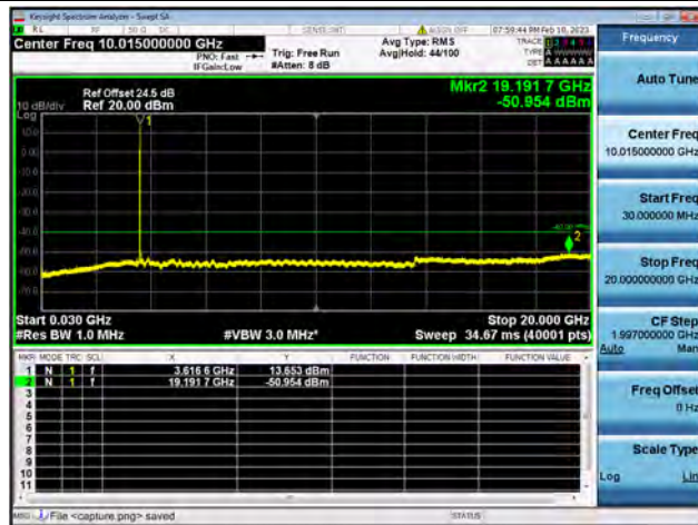
Band48-30M-20G / 20MHz / Mid CH / 16QAM
