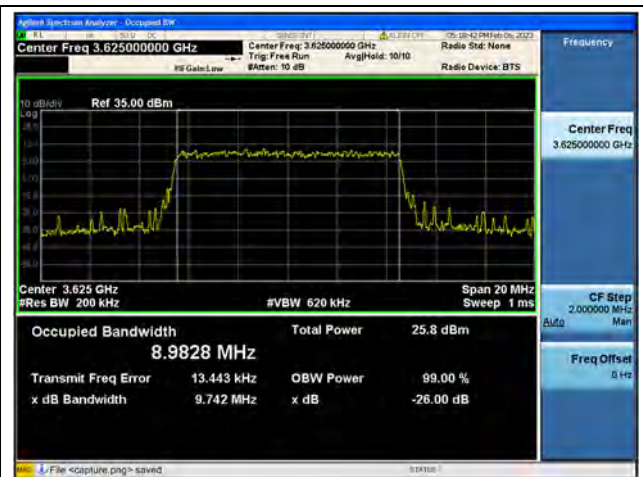
Band48 / 10MHz / 16QAM/ Mid CH
