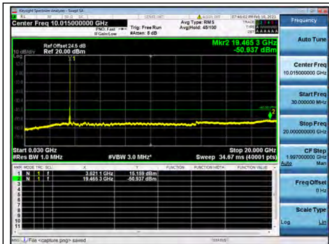
Band48-30M-20G / 10MHz / Mid CH / QPSK
