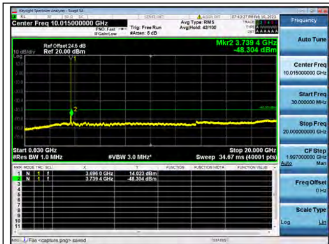
Band48-30M-20G / 5MHz / High CH / QPSK
