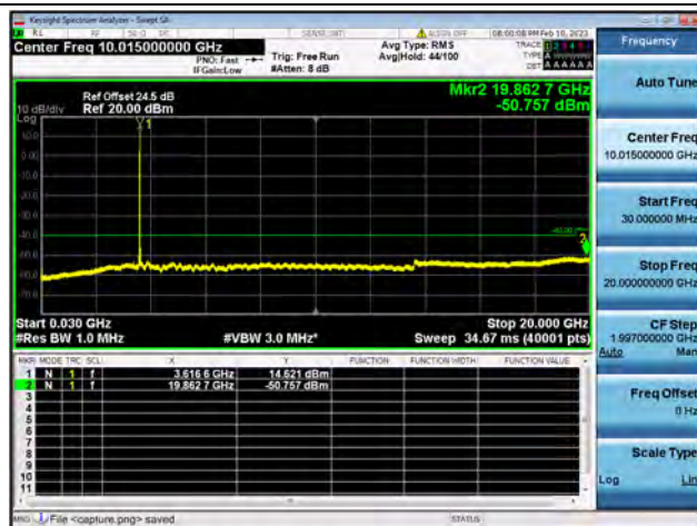
Band48-30M-20G / 20MHz / Mid CH / 64QAM
