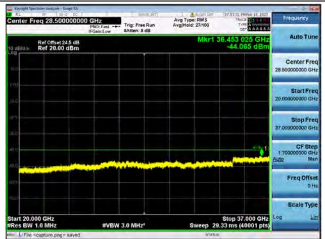
Band48-20G-37G / 10MHz / High CH / 16QAM
