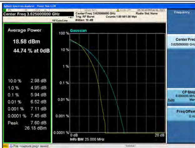
Band48 / 15MHz / Mid CH / 16QAM
