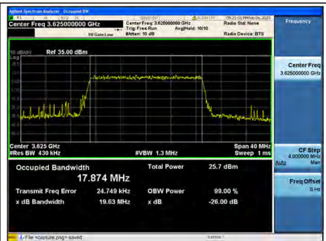
Band48 / 20MHz / 16QAM/ Mid CH
