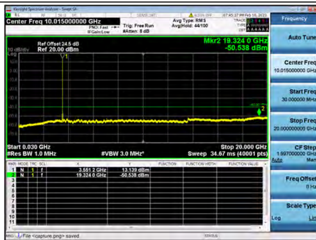
Band48-30M-20G / 10MHz / Low CH / 64QAM
