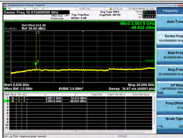
Band48-30M-20G / 20MHz / Low CH / 64QAM
