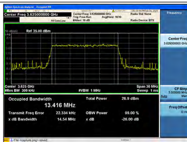
Band48 / 15MHz / QPSK/ Mid CH
