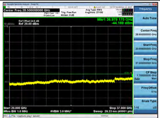
Band48-20G-37G / 15MHz / High CH / 16QAM
