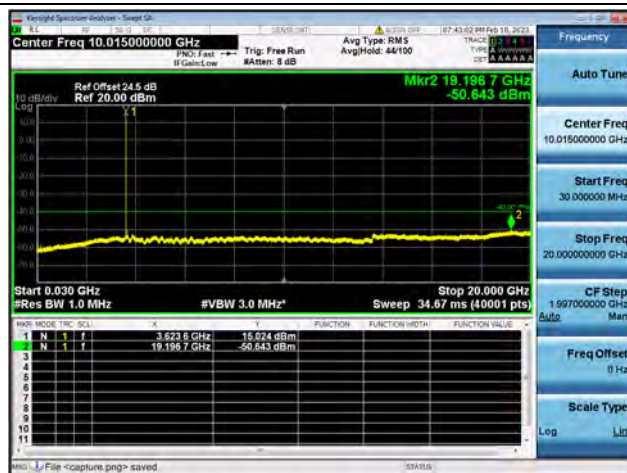
Band48-30M-20G / 5MHz / Mid CH / 64QAM
