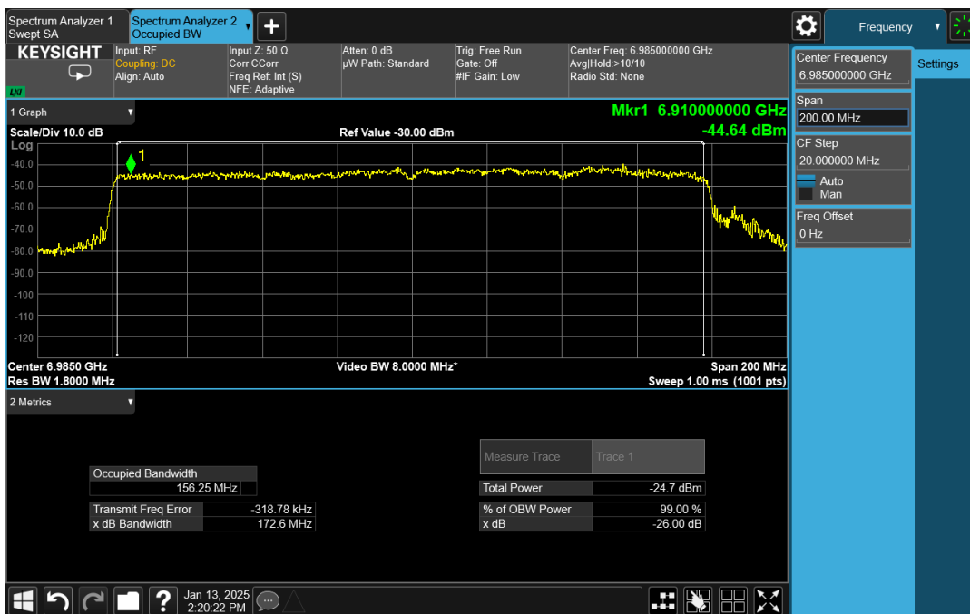
Plot 3: AWGN BW 160MHz
