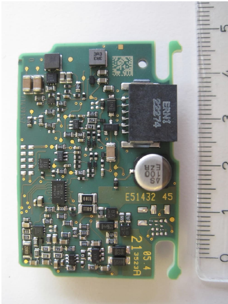
Main board, top view
