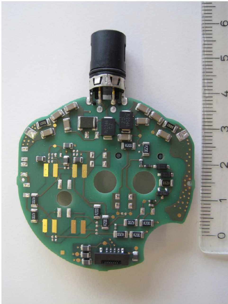
Terminal board, bottom view
