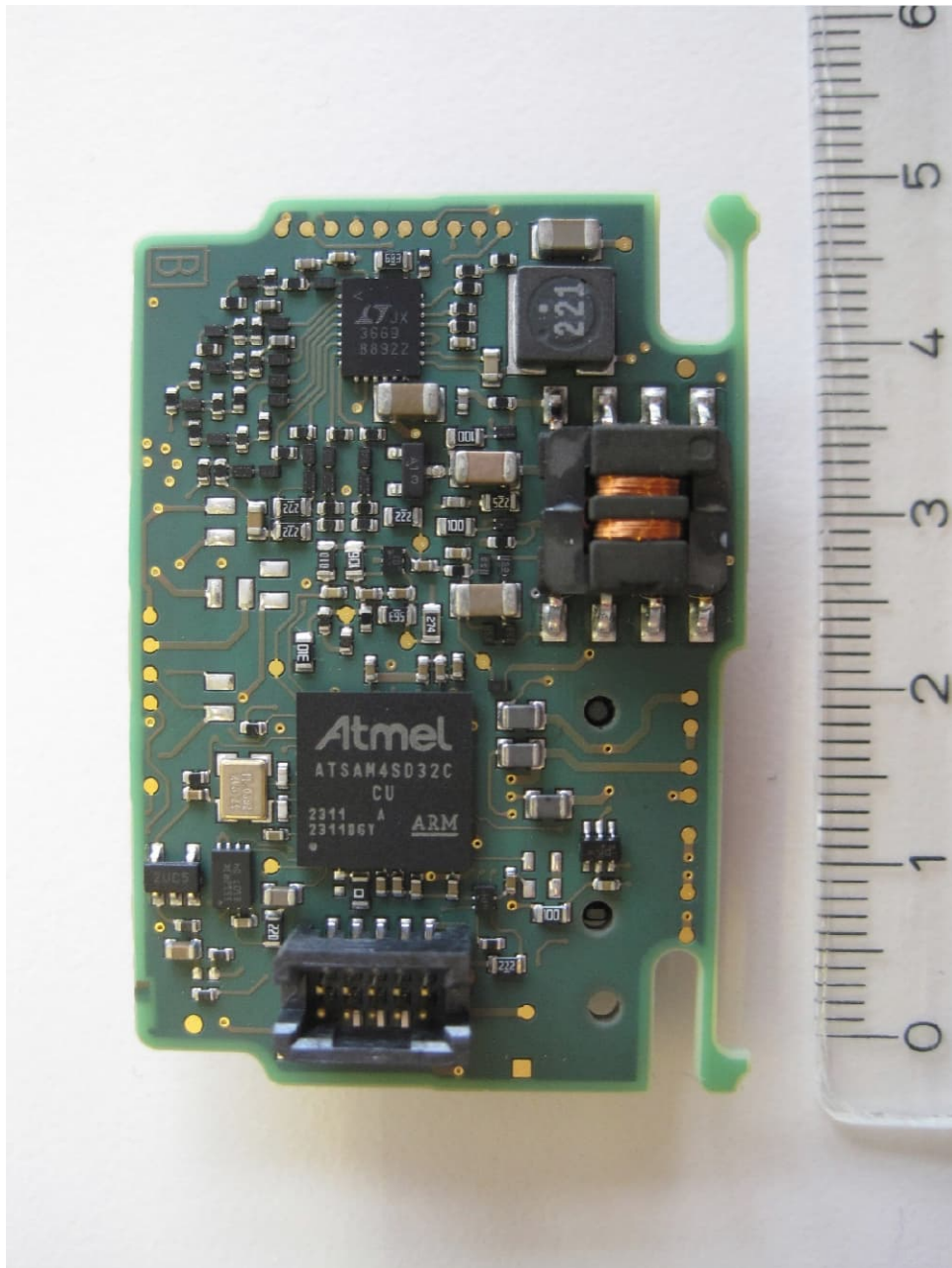
Main board, bottom view
