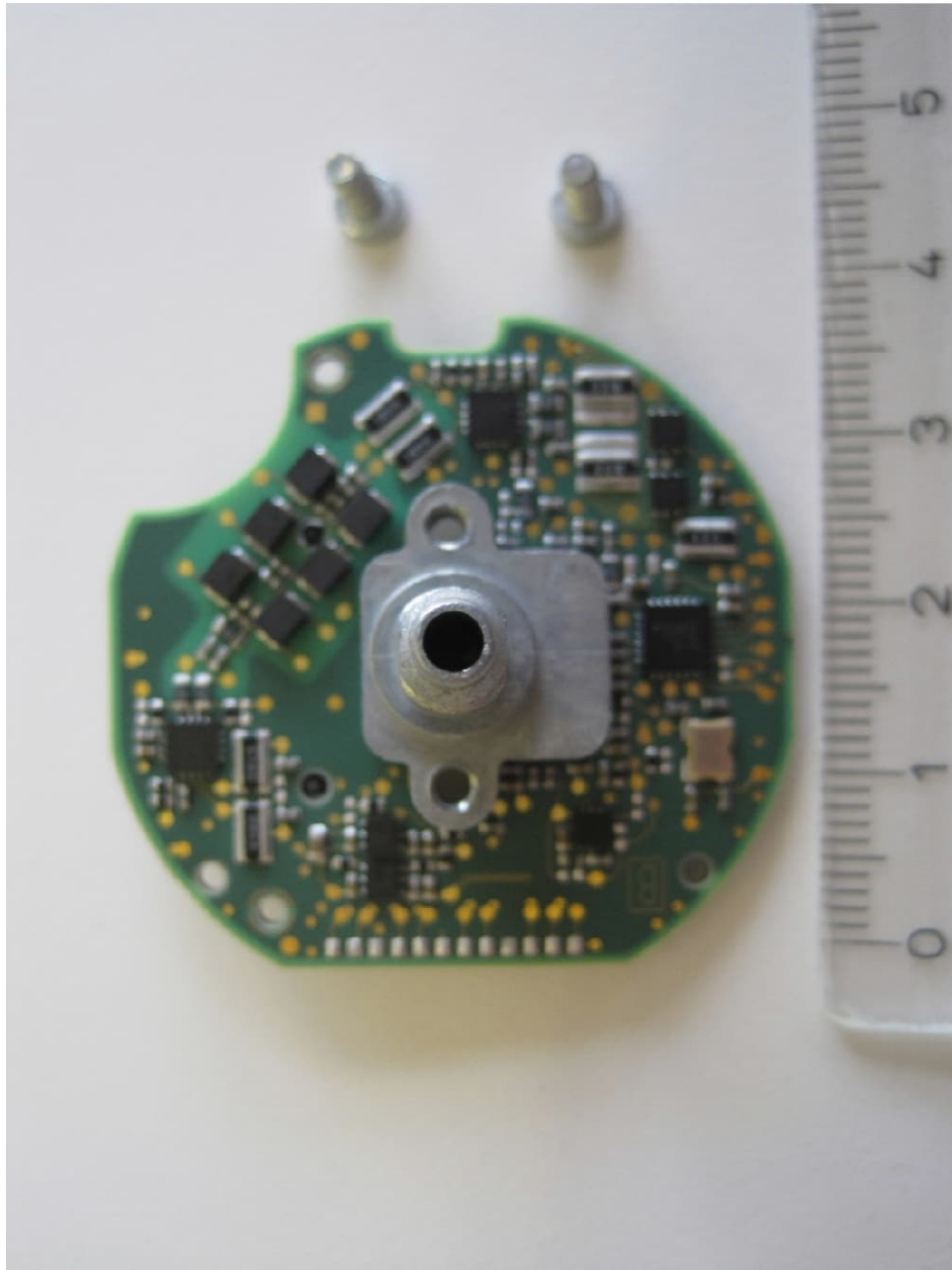
Sensor board, top view
