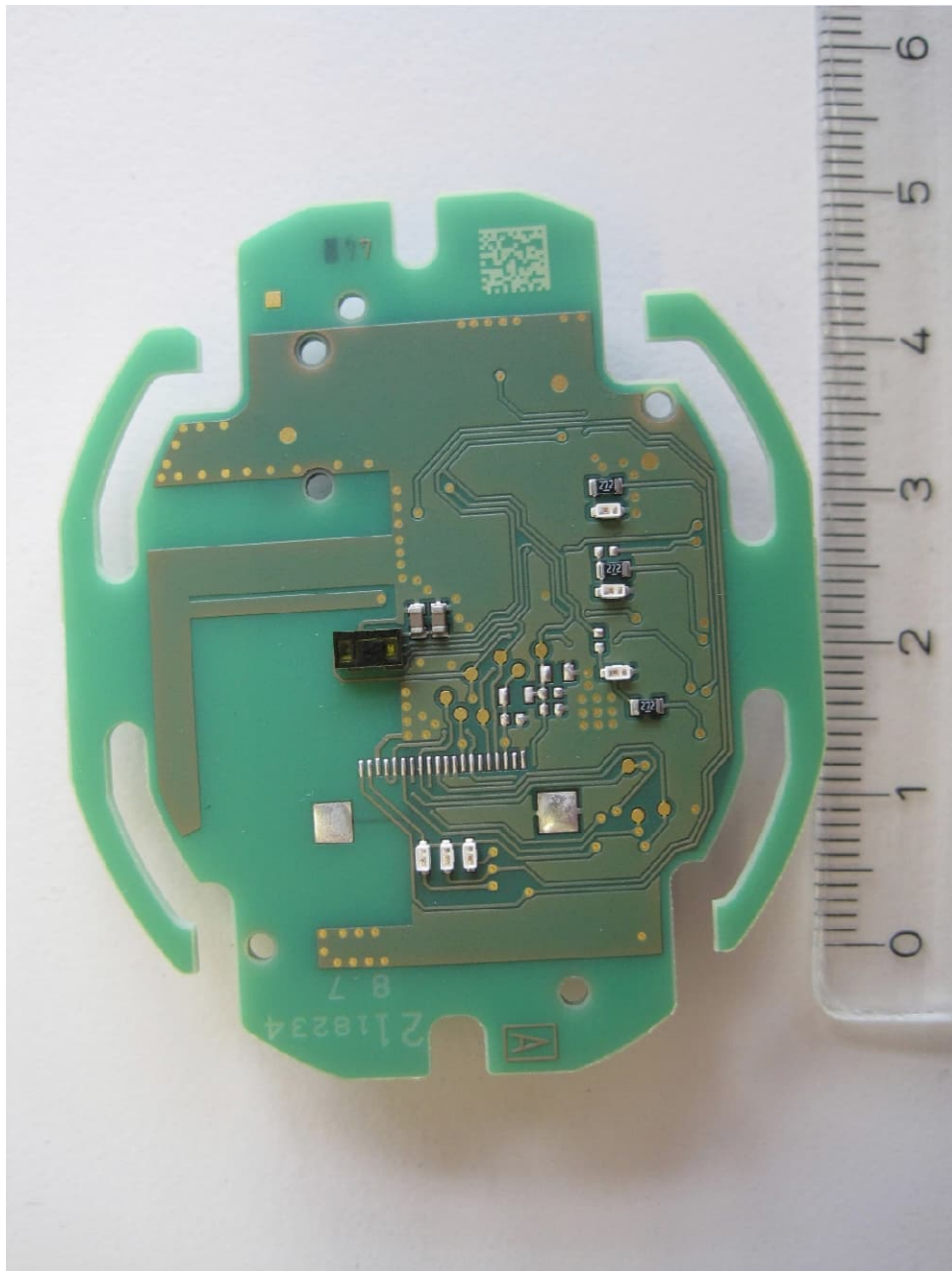
LED board, top view
