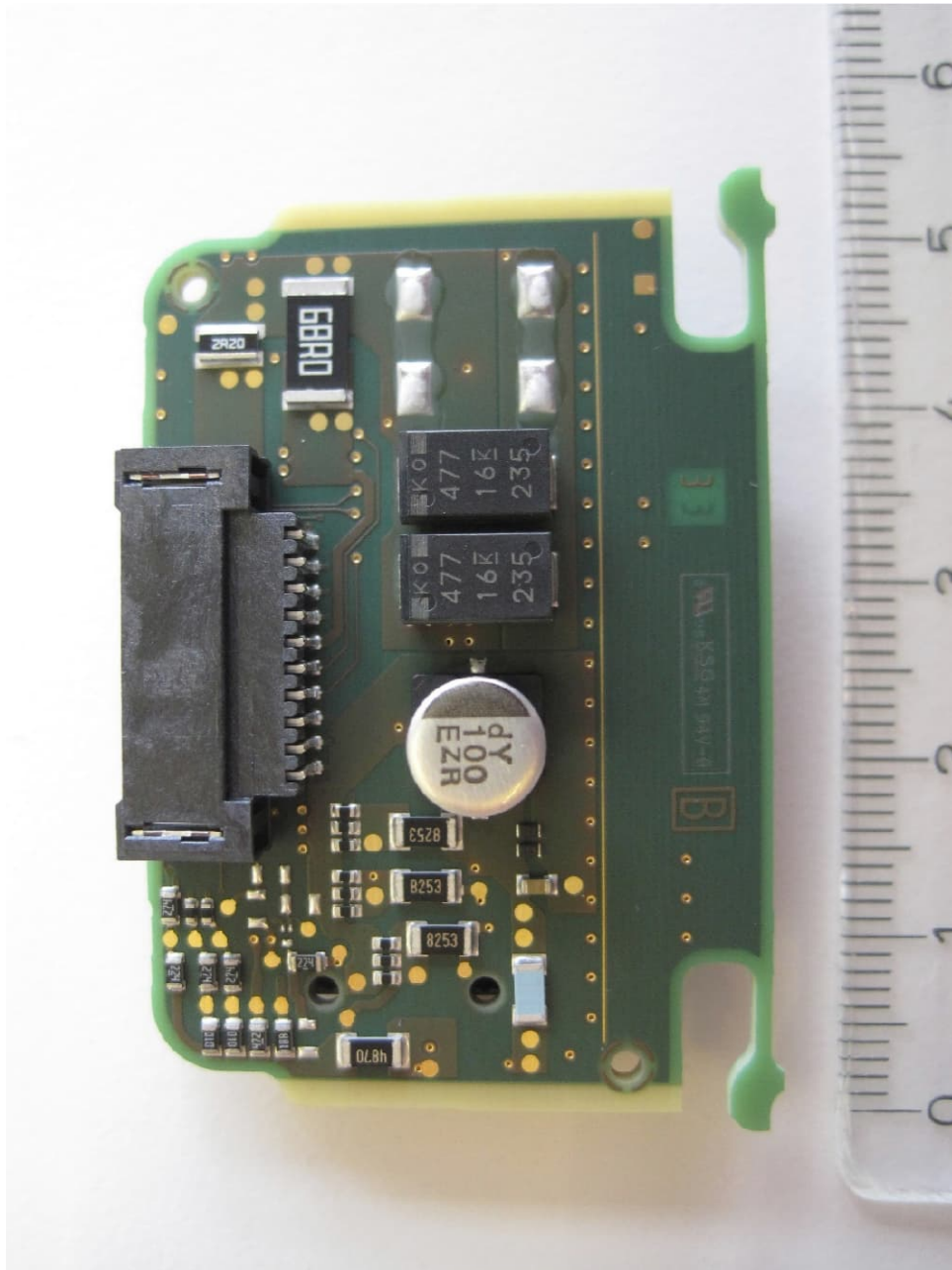
Power board, top view
