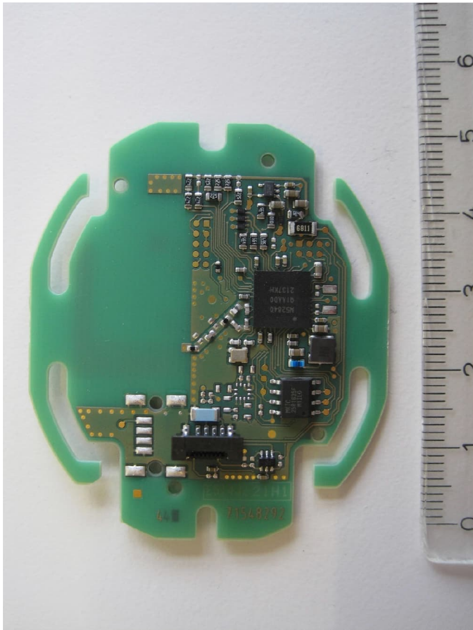
LED board, bottom view
