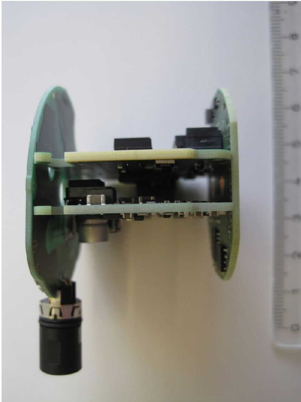
PCBs removed from electronic housing
