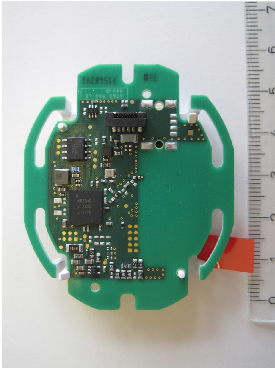
LCD board, bottom view
