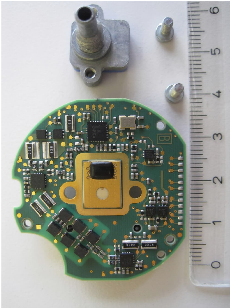
Sensor board, top view, wave guide removed
