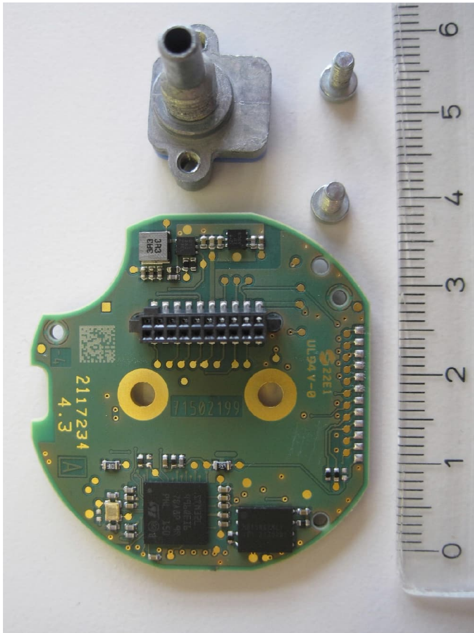
Sensor board, bottom view
