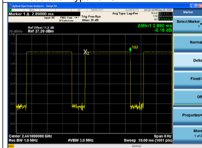
Modulation type: GFSK DH5 2441MHz
