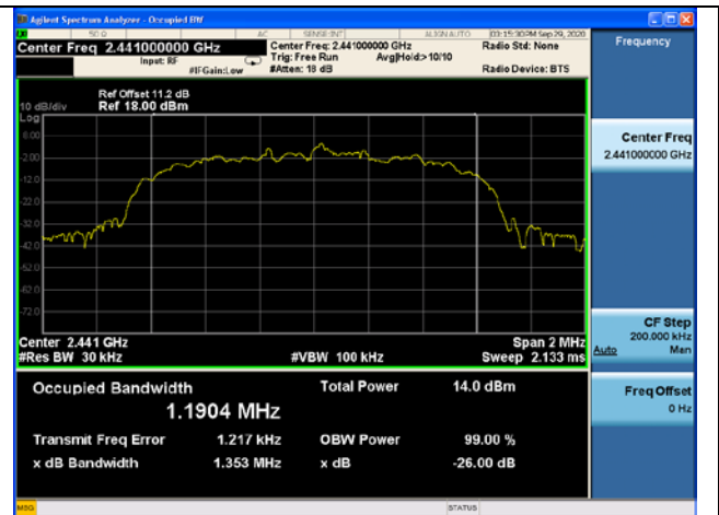
Modulation type: 8DPSK2441MHz
