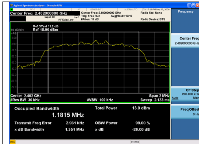
Modulation type: 8DPSK2402MHz
