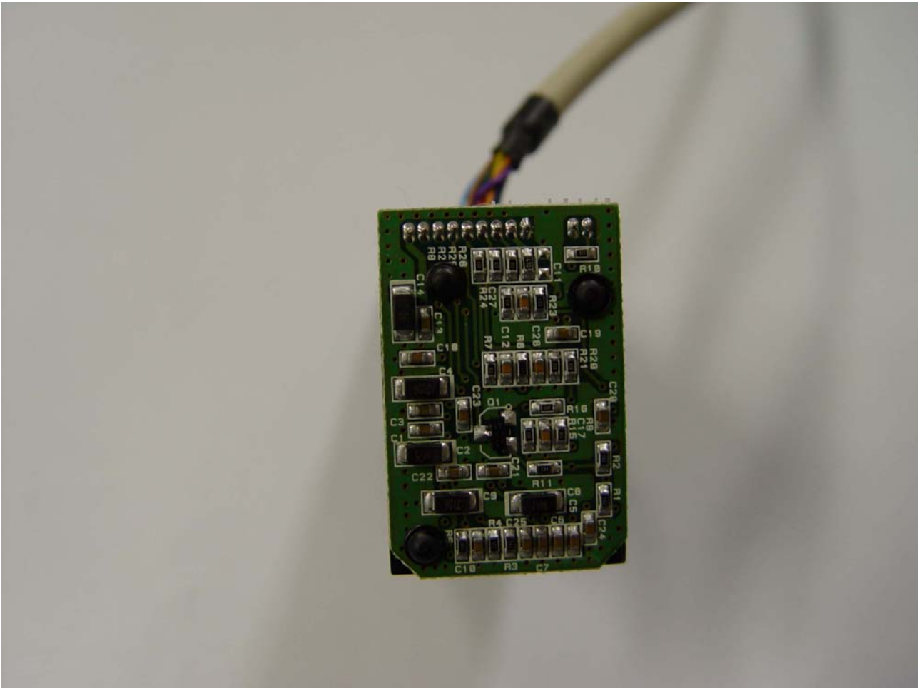
Figure 3. Fingerprint Optic Module front Side
