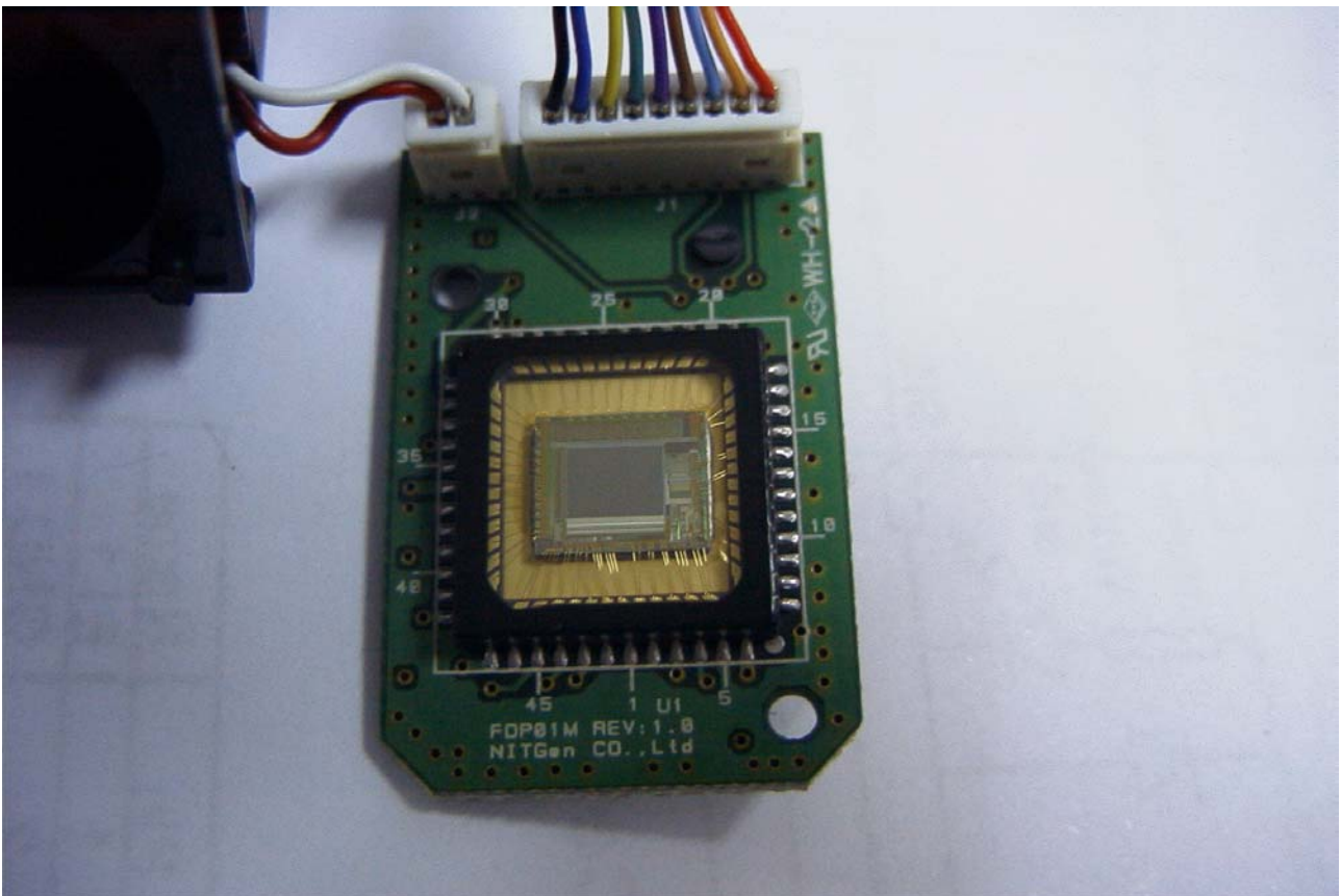
Figure 4. Fingerprint Optic Module back side
