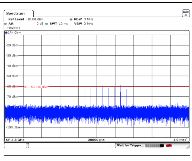
Single Burst of Radar Type 6
