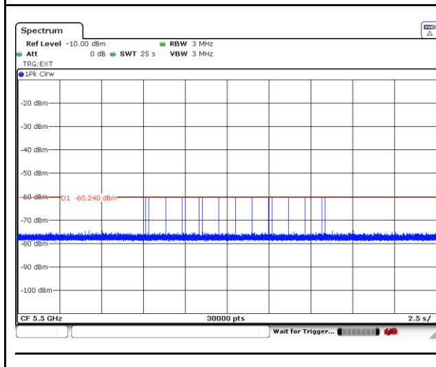
Single Burst of Radar Type 5
