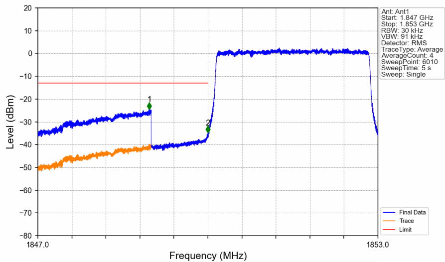
Band2_3MHz_16QAM_LCH_1851.5MHz_RB_15_0_NTNV
